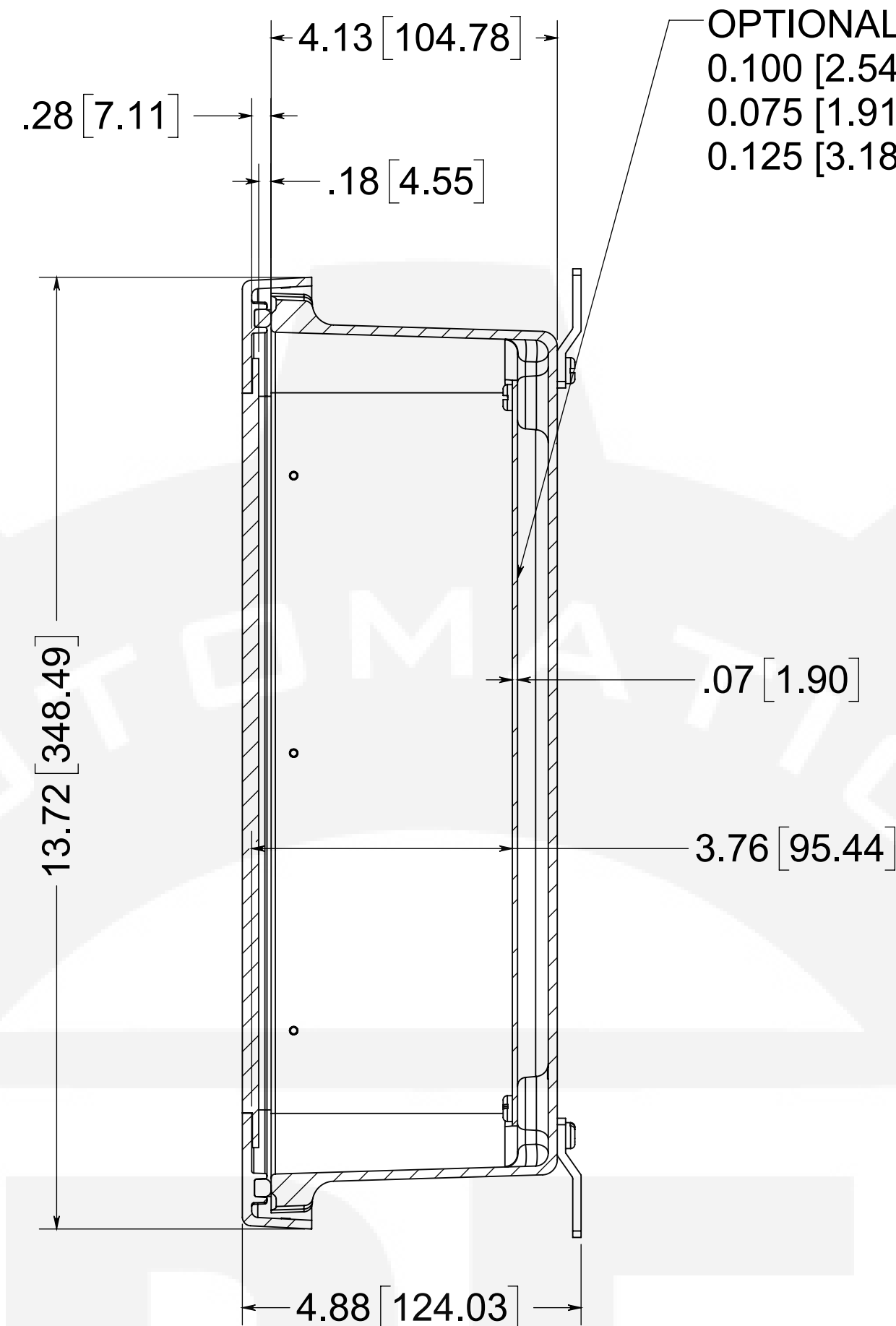
SECTION B-B
