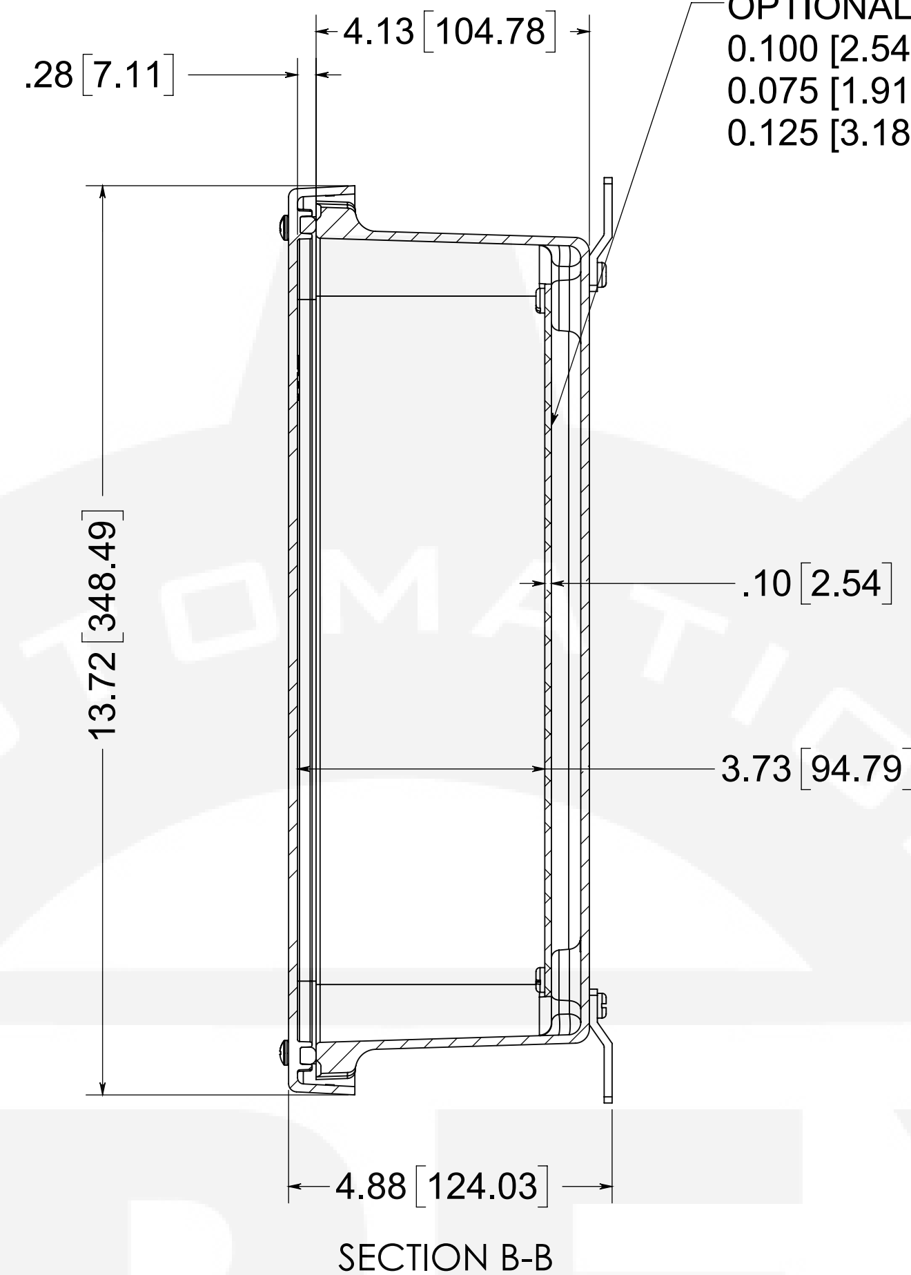
SECTION B-B
