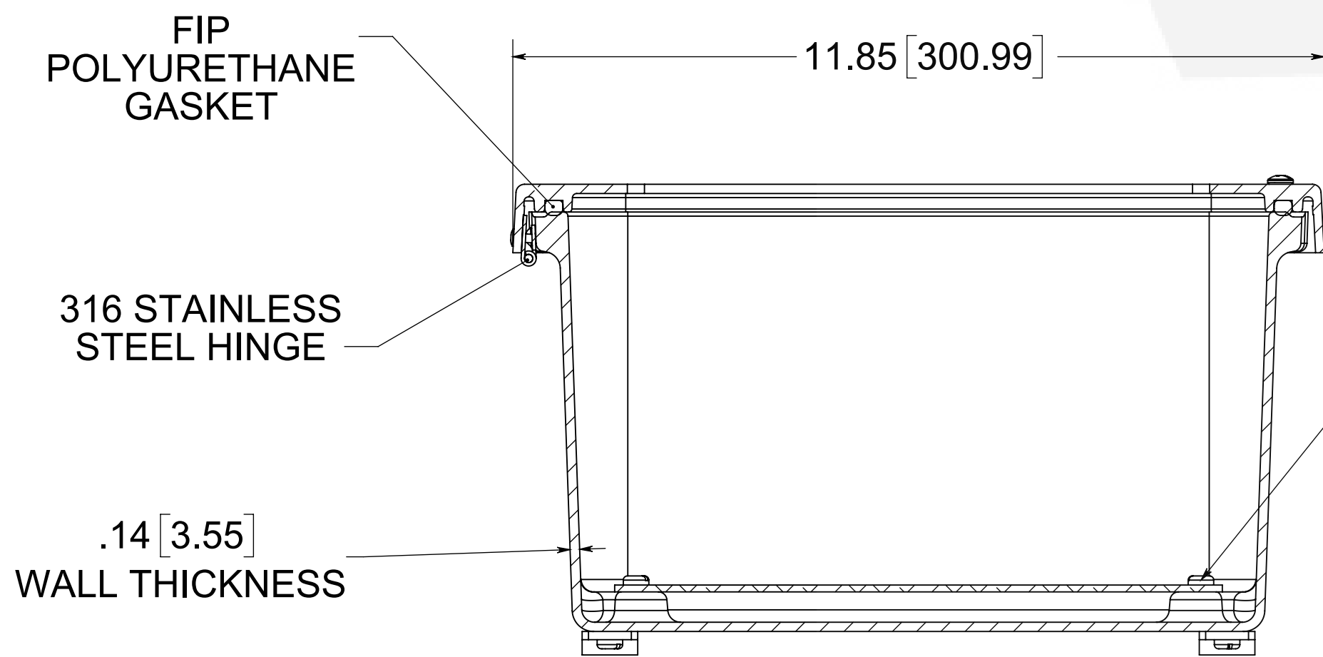
SECTION B-B
