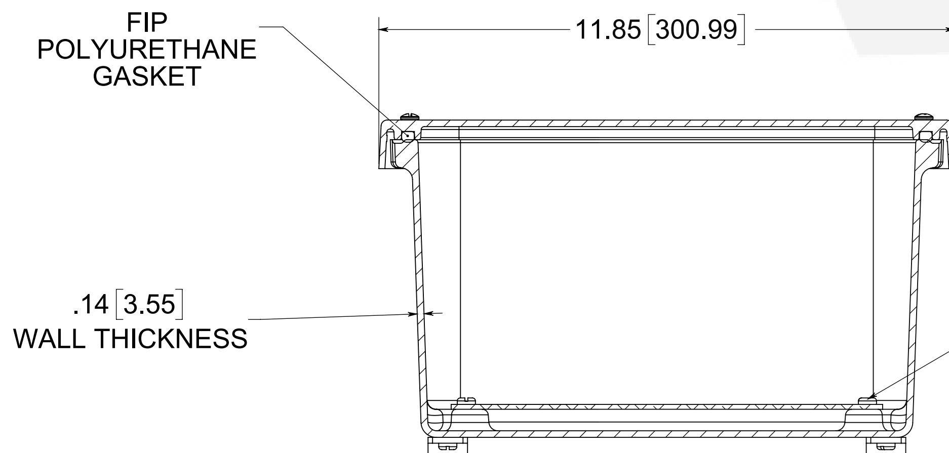
SECTION B-B
