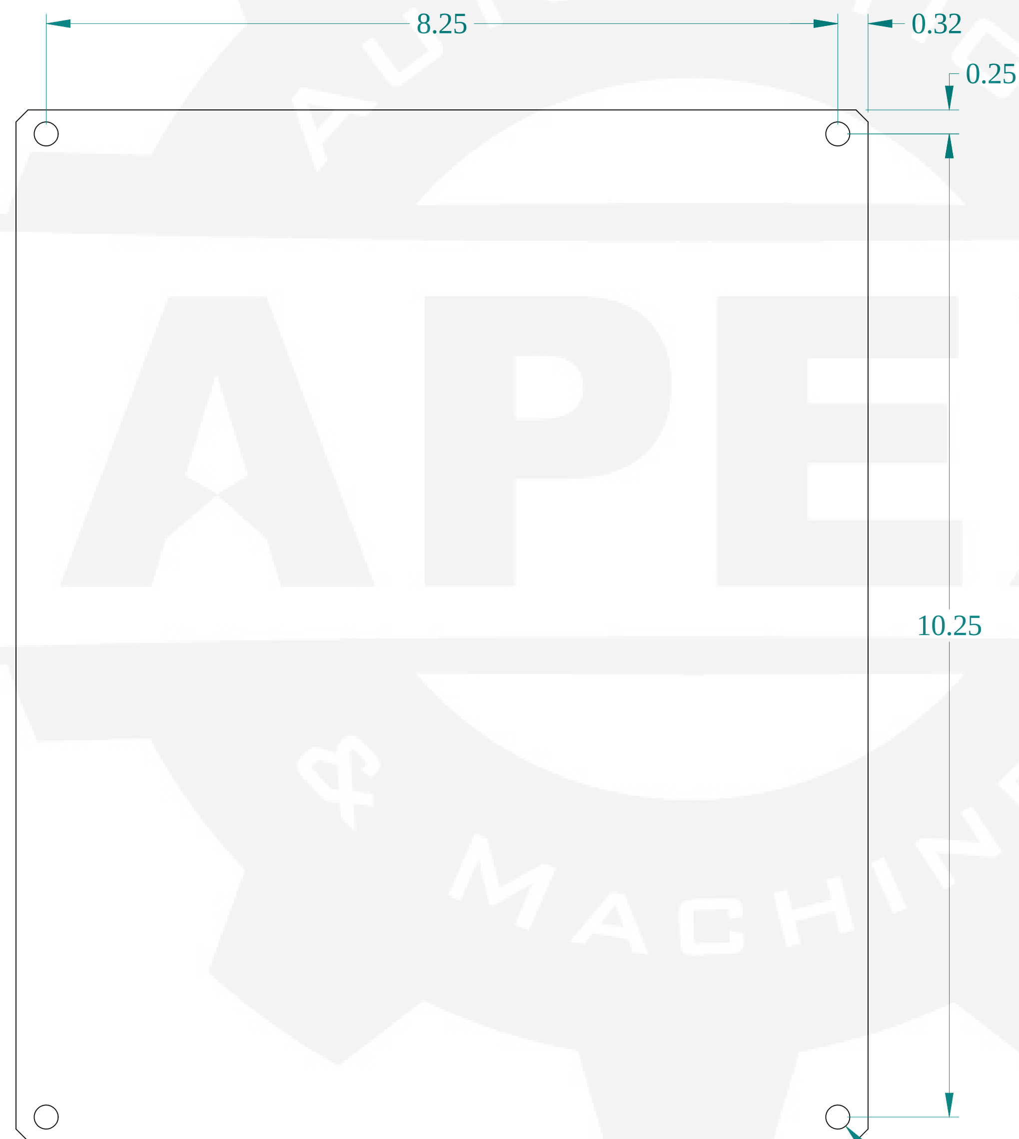
FRONT VIEW
