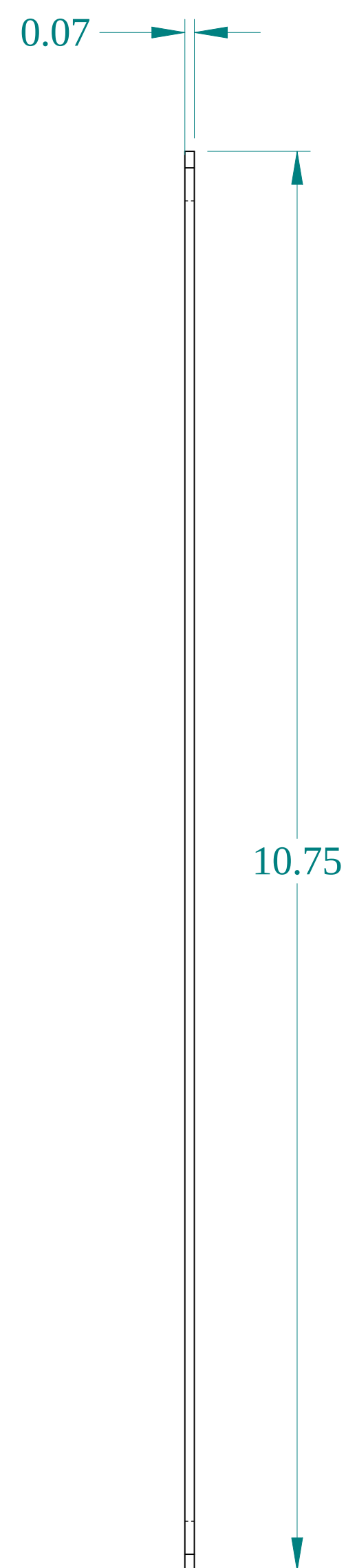
SIDE VIEW
