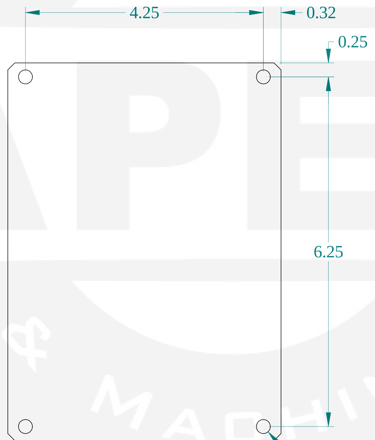
FRONT VIEW
