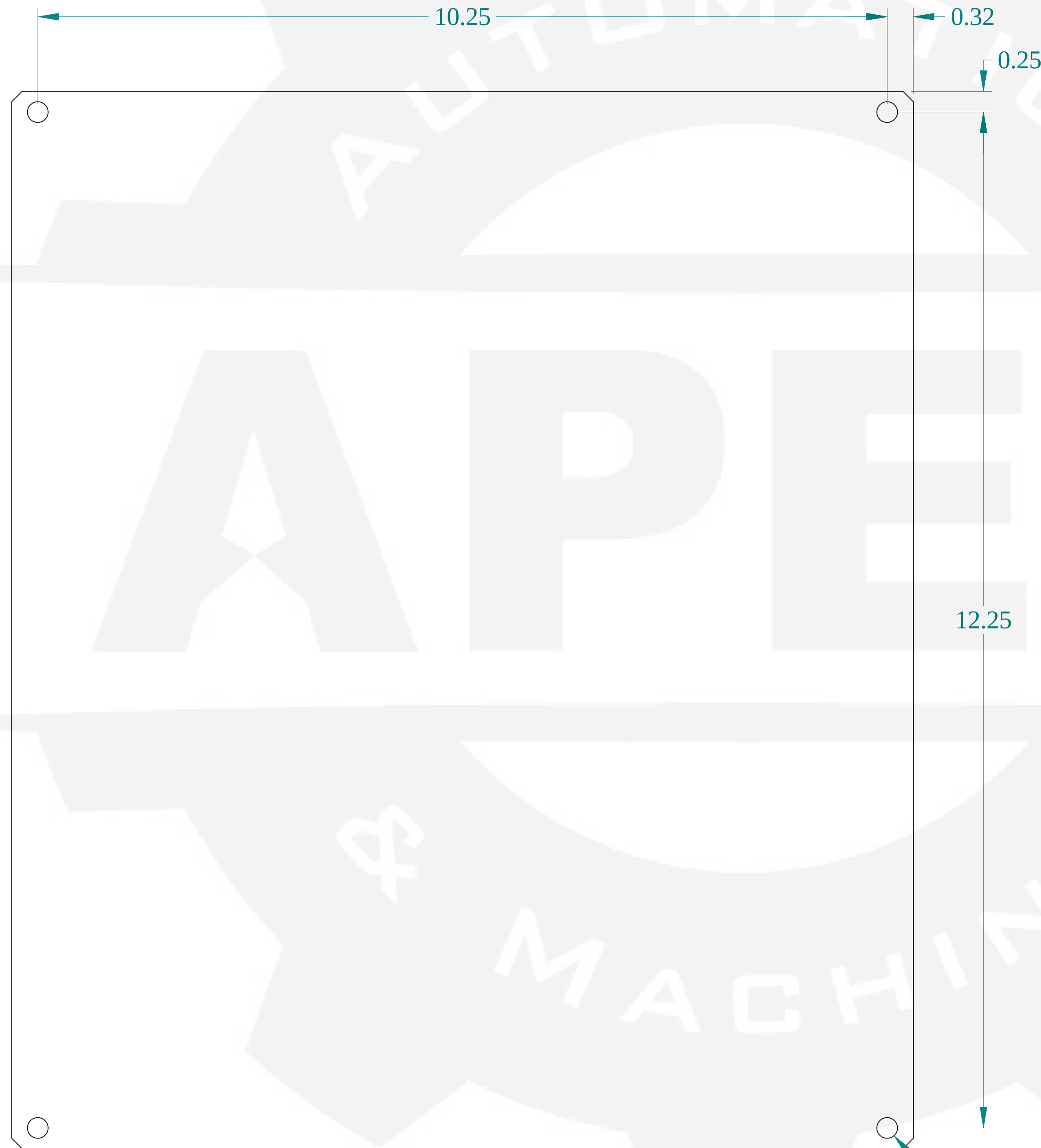
FRONT VIEW
