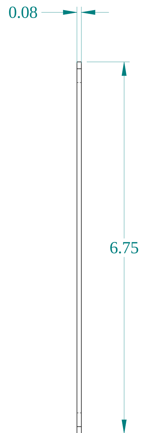
SIDE VIEW
