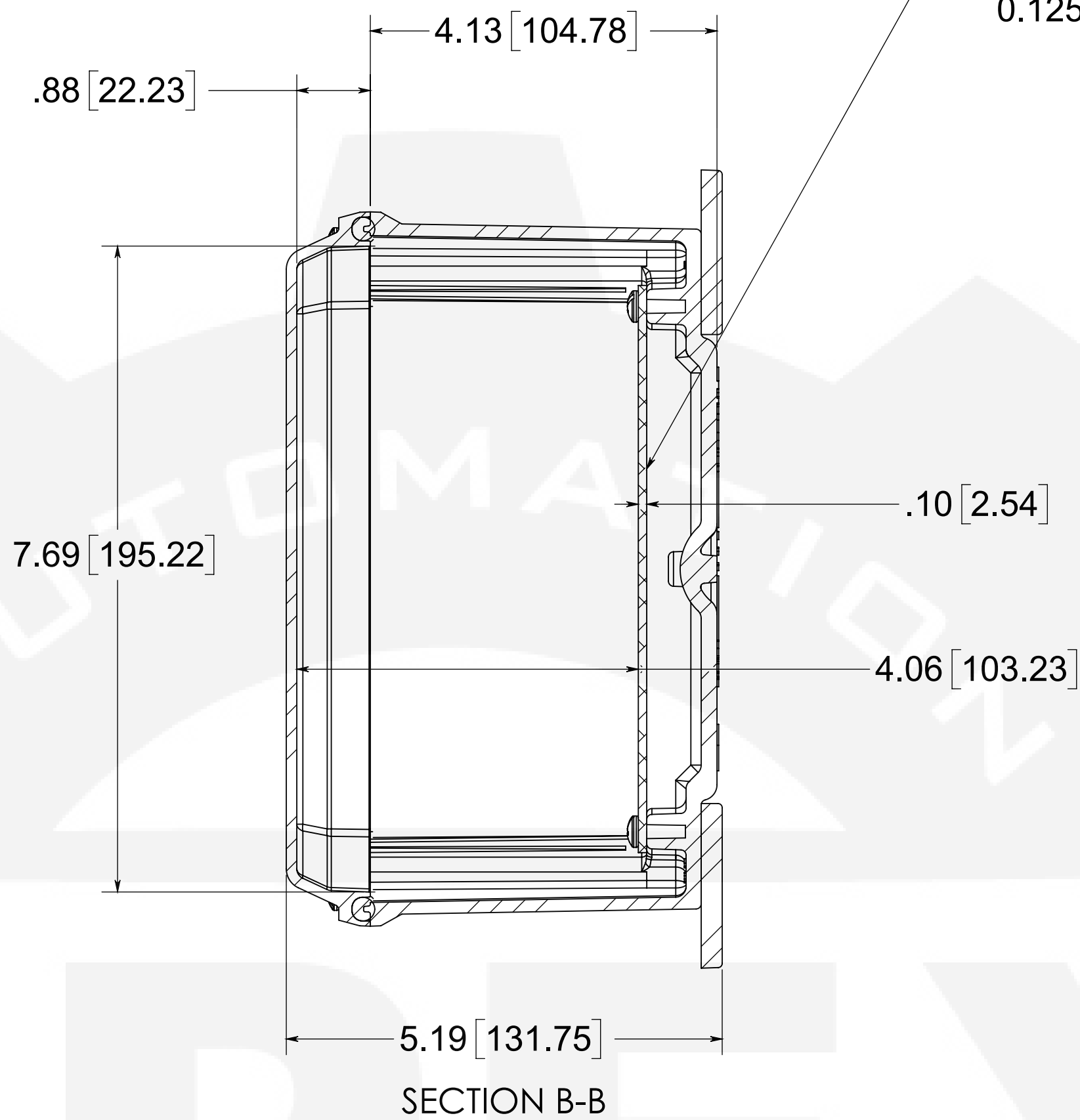
SECTION B-B
