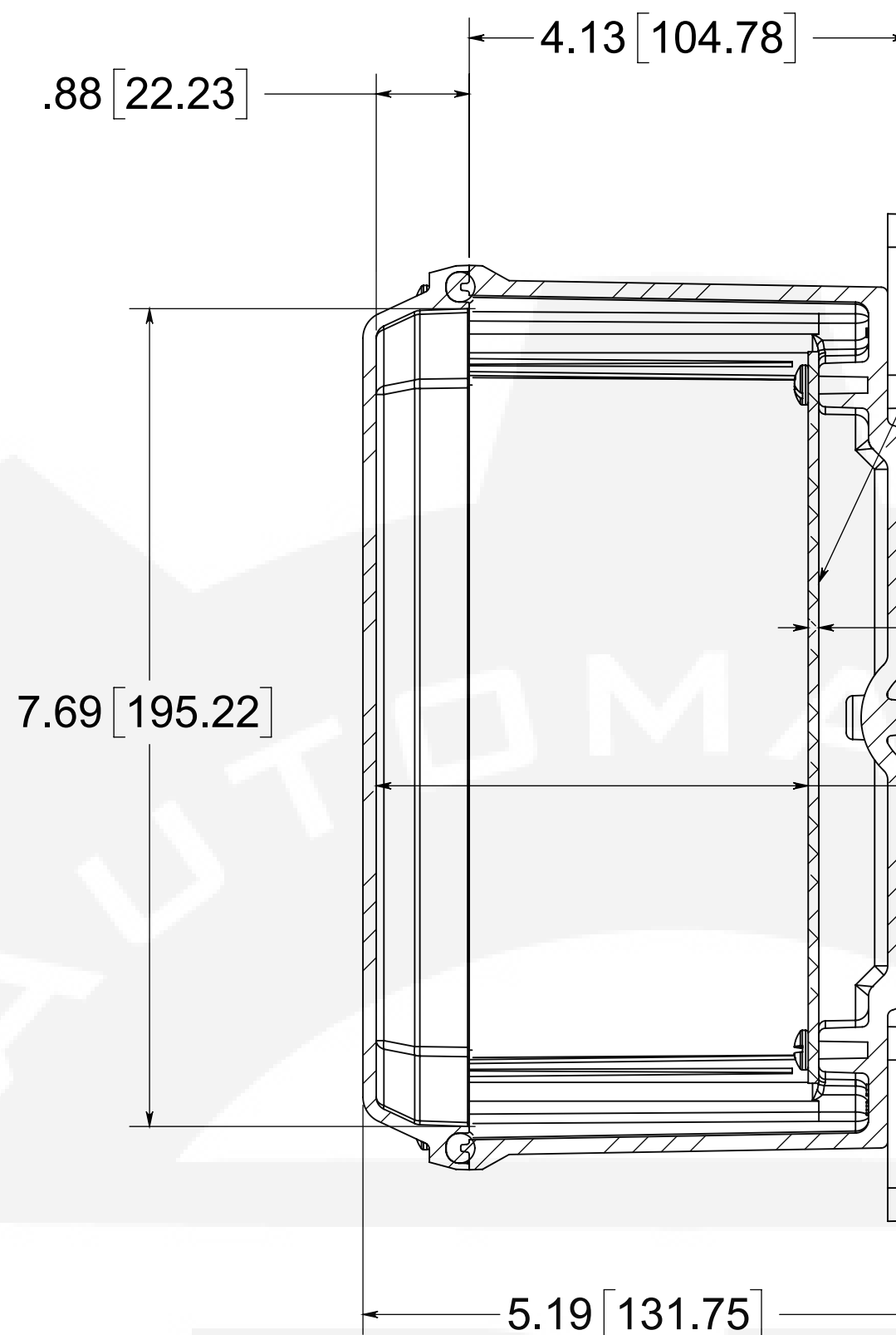
SECTION B-B
