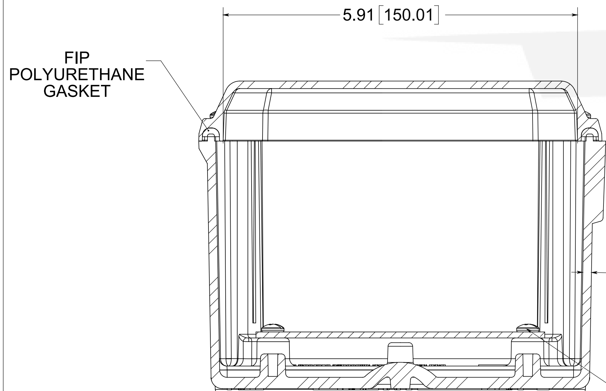
SECTION F-F
