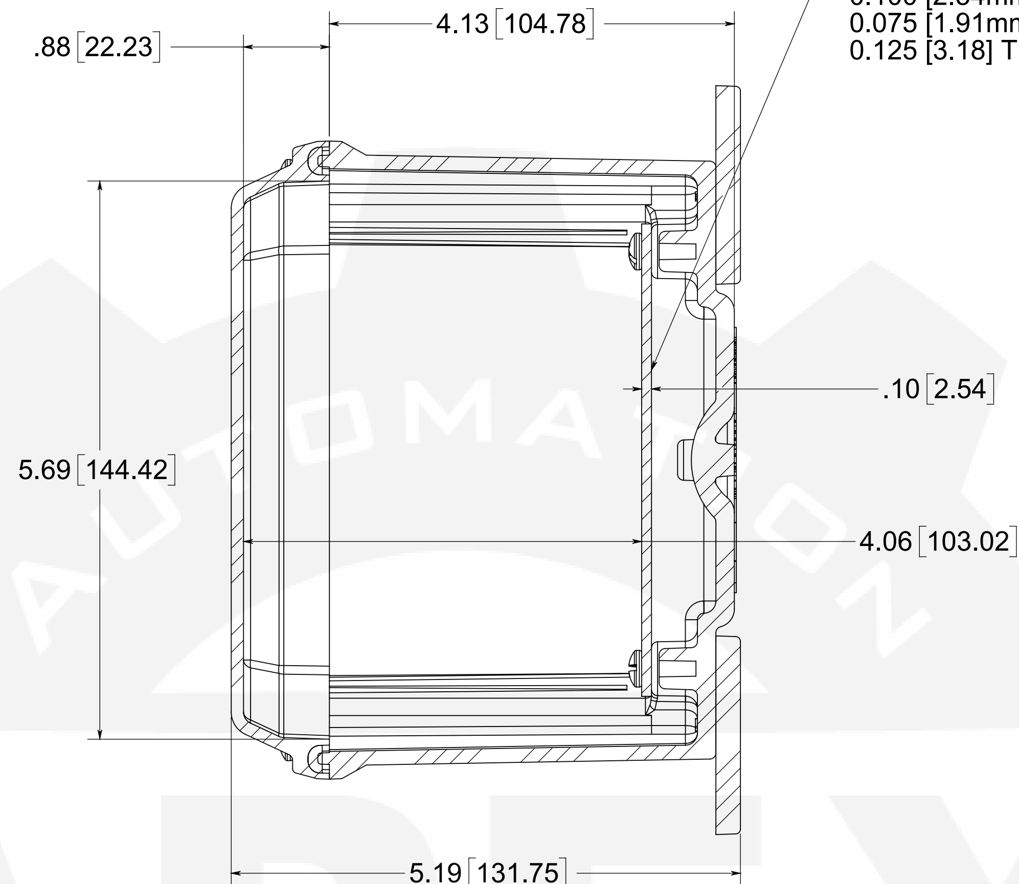
SECTION B-B
