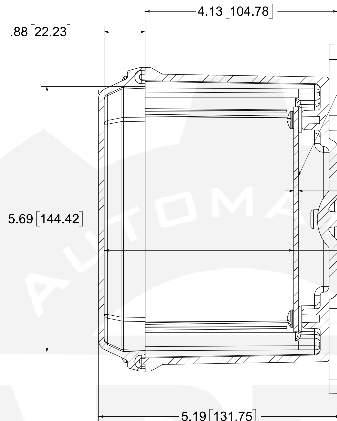
SECTION B-B
