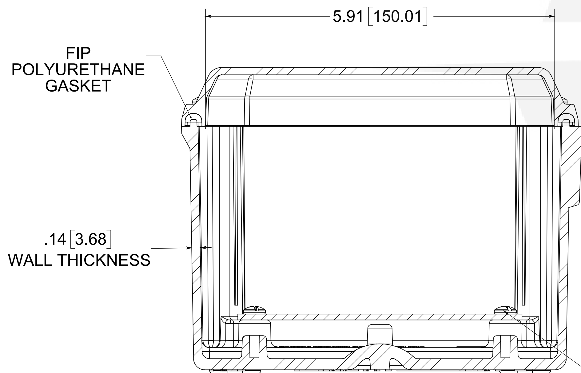
SECTION B-B
