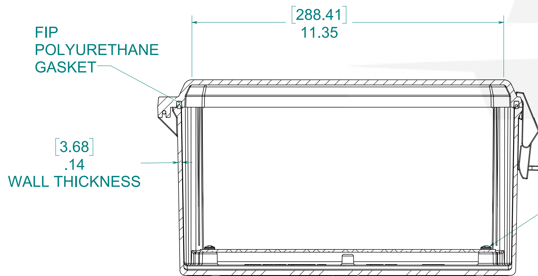
SECTION B-B
