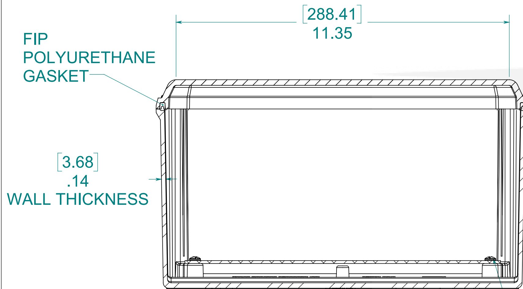
SECTION B-B
