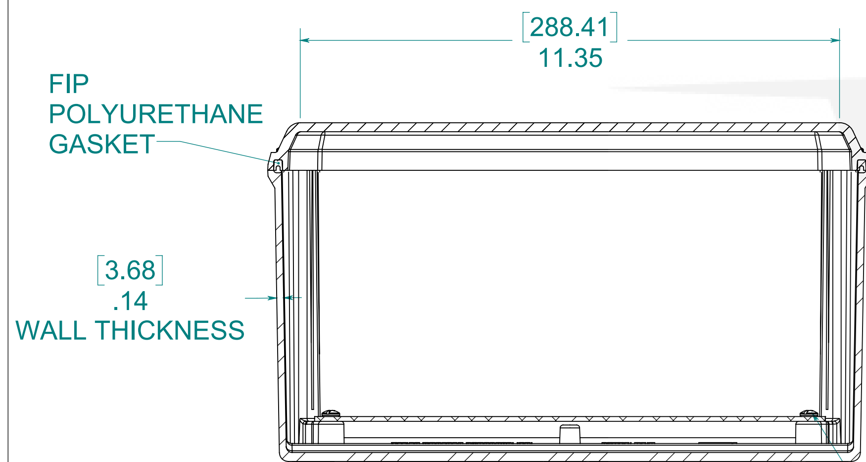
SECTION B-B
