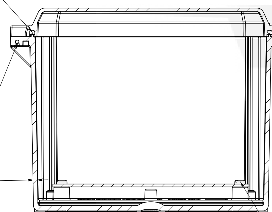
SECTION B-B
