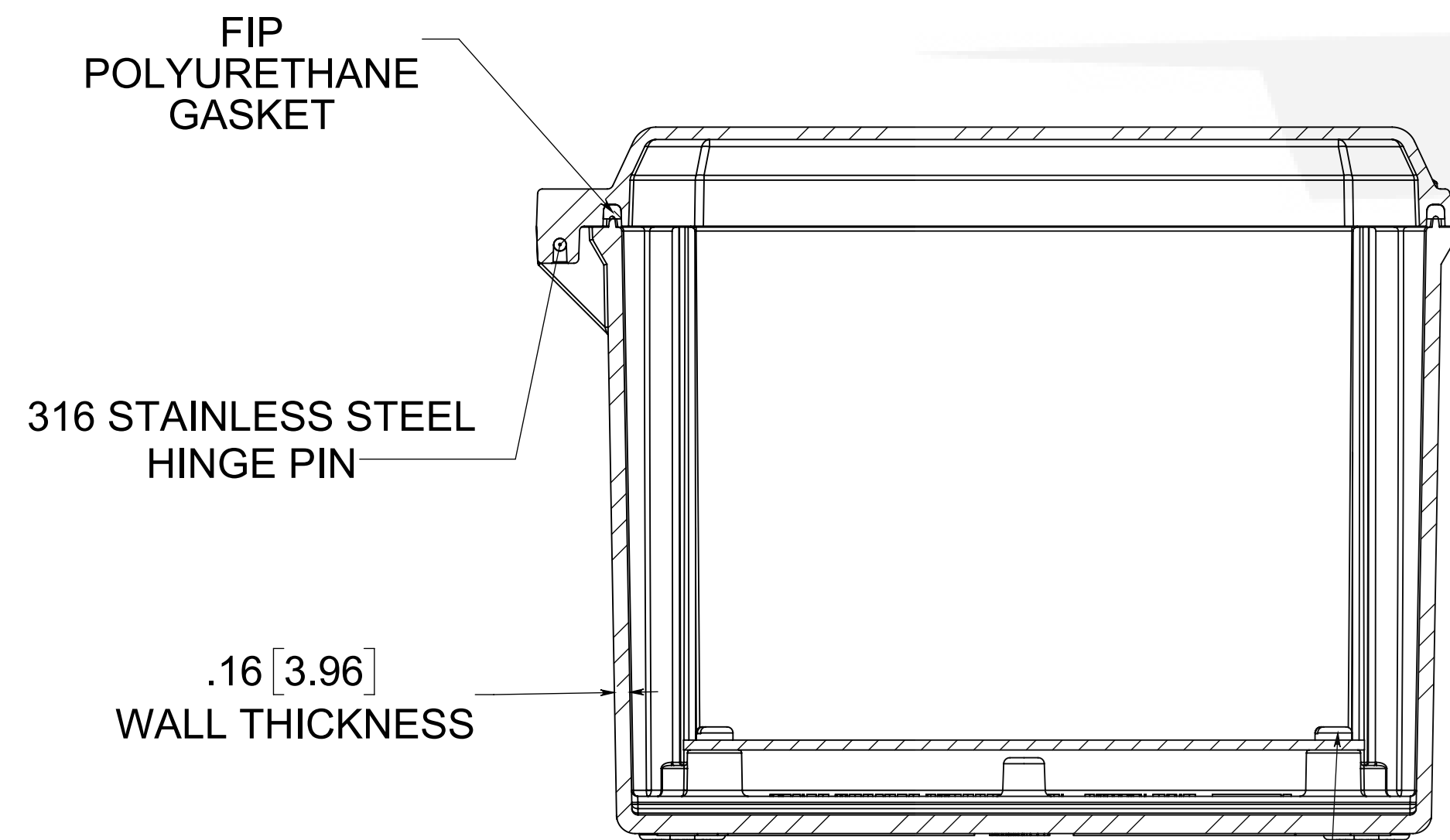
SECTION B-B
