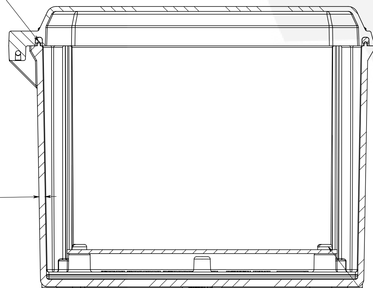
SECTION B-B
