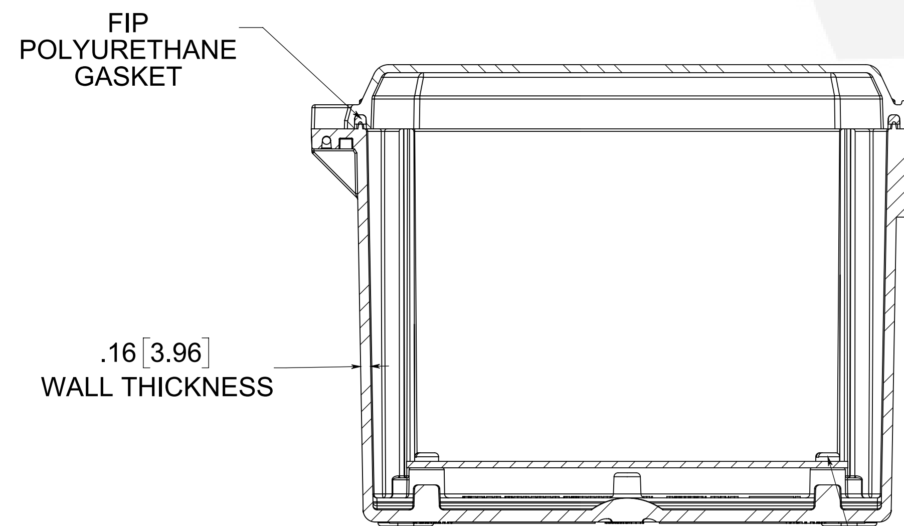
SECTION B-B
