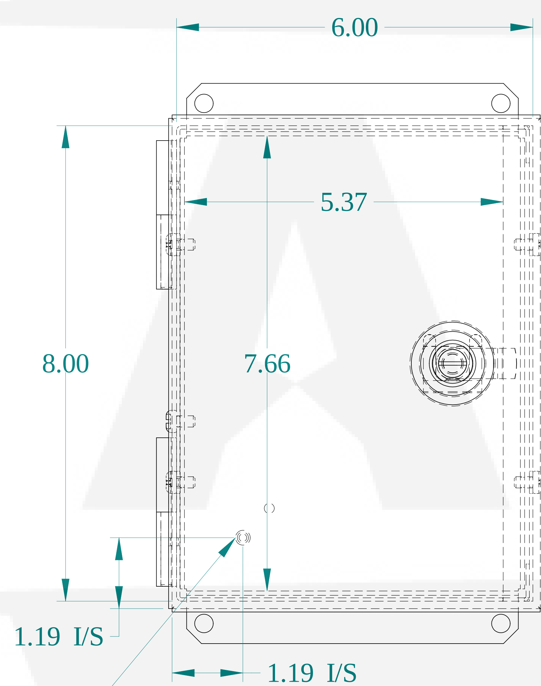
FRONT VIEW
