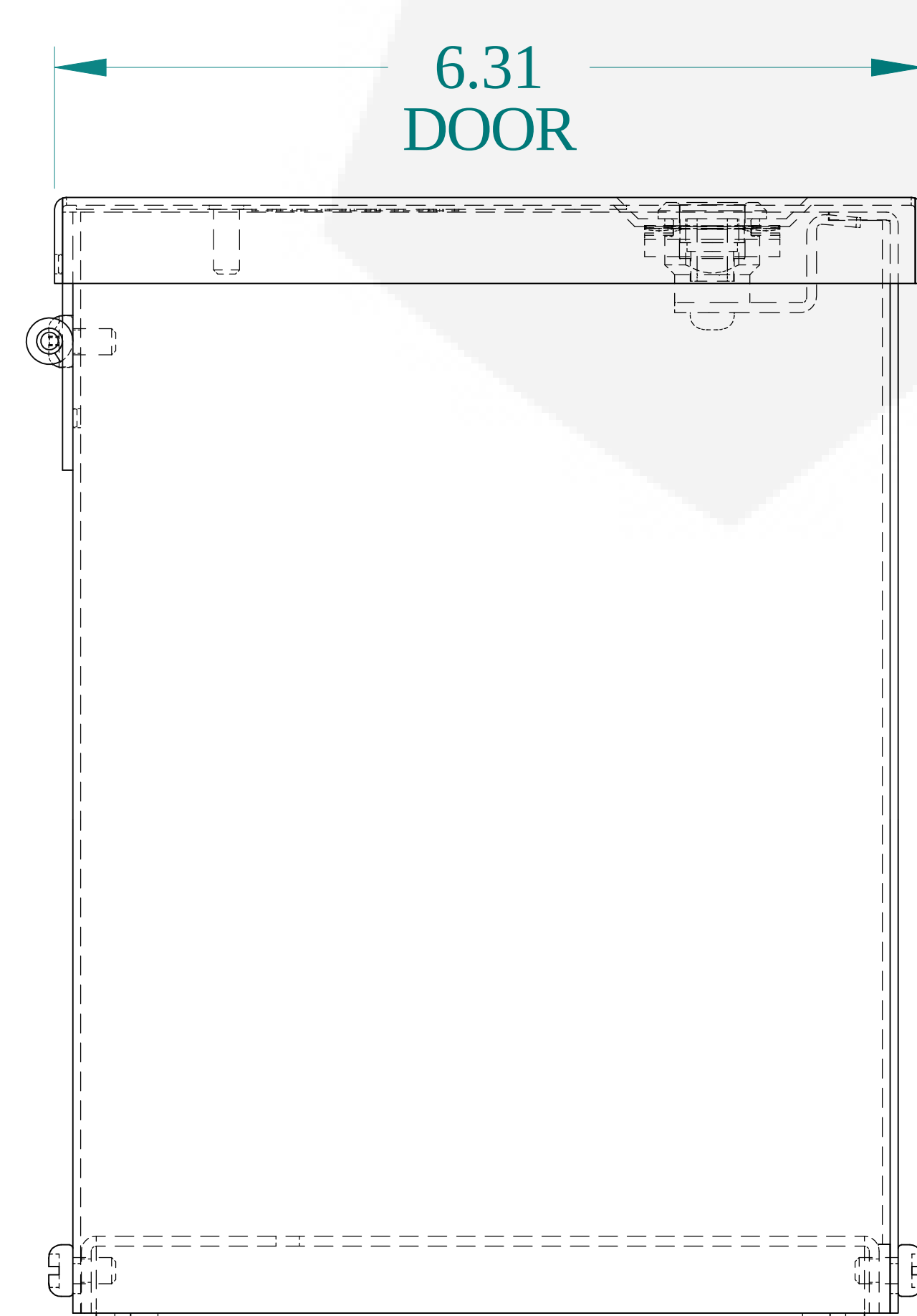
BOTTOM VIEW
