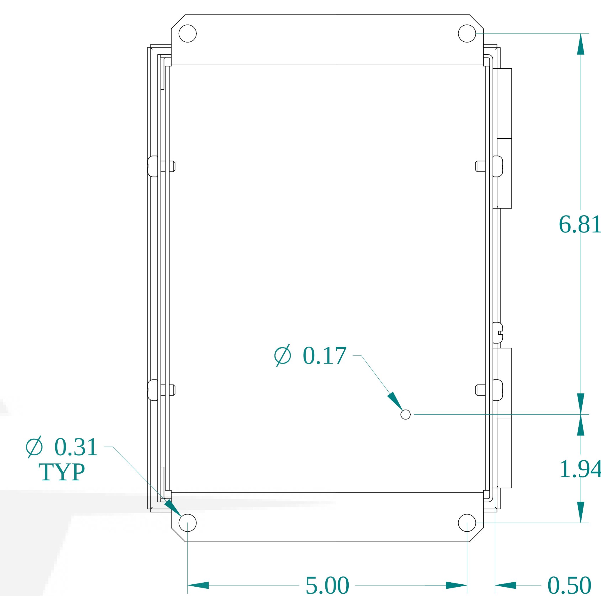
BACK VIEW
