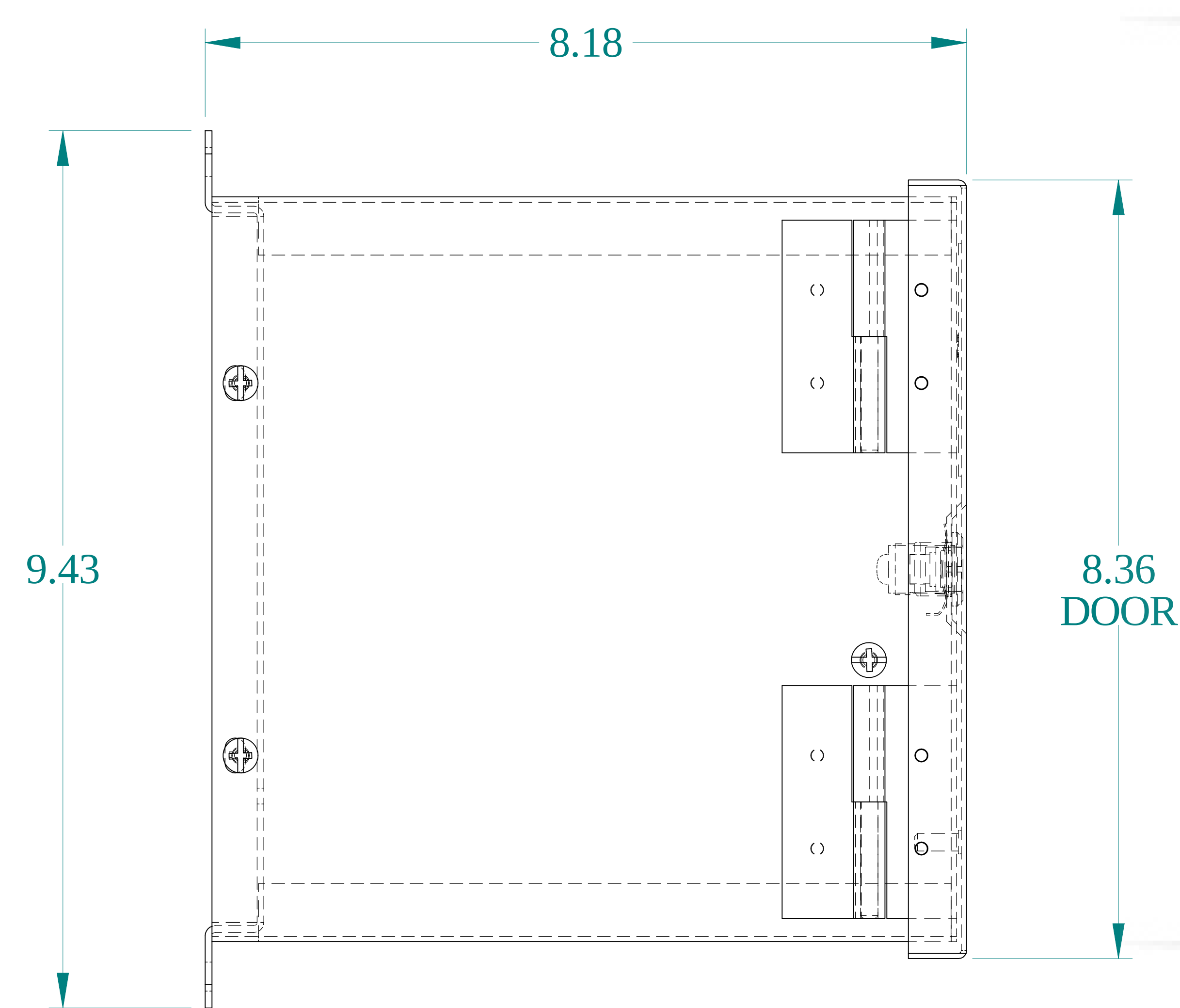
SIDE VIEW
