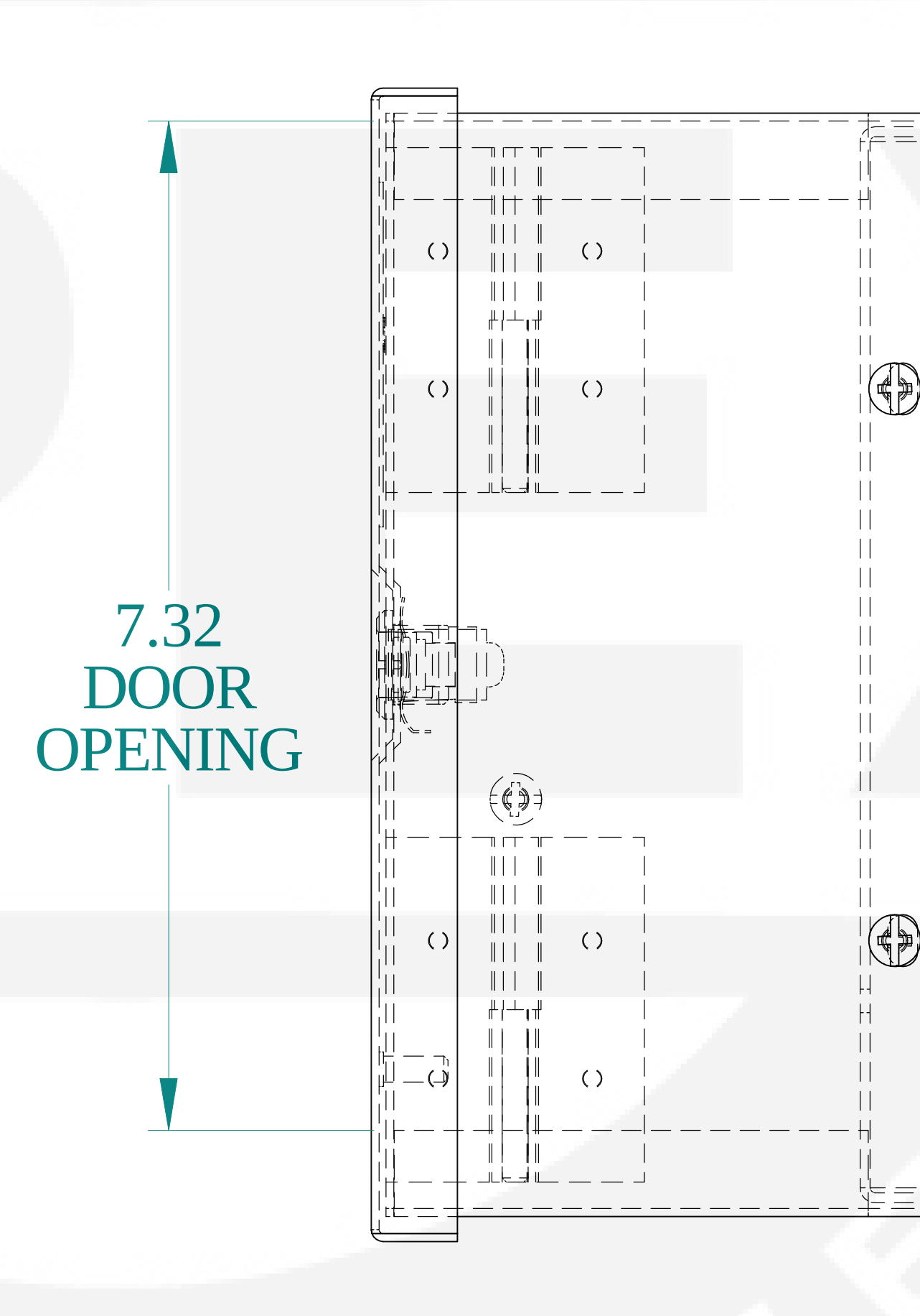
SIDE VIEW
