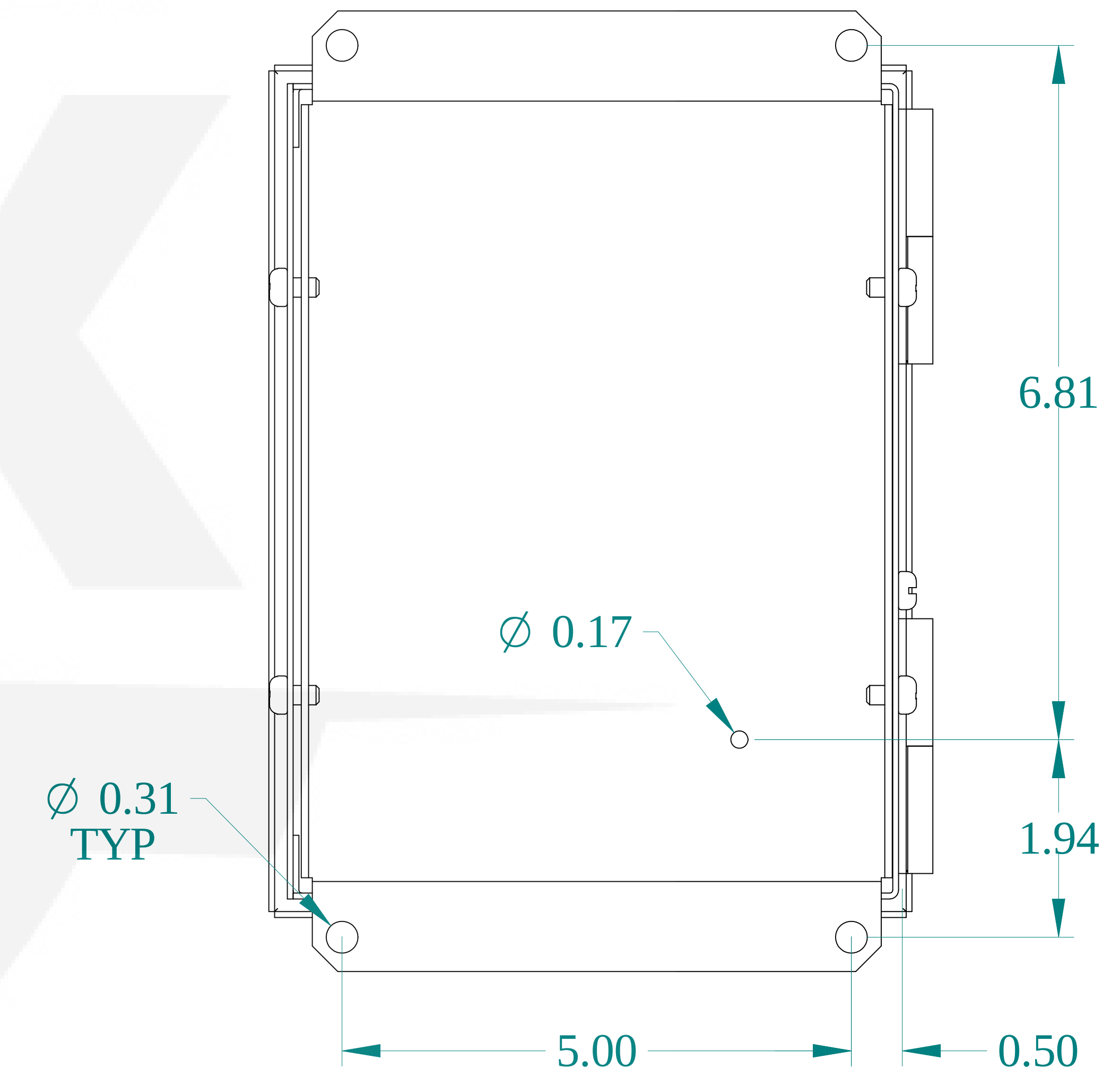
BACK VIEW
