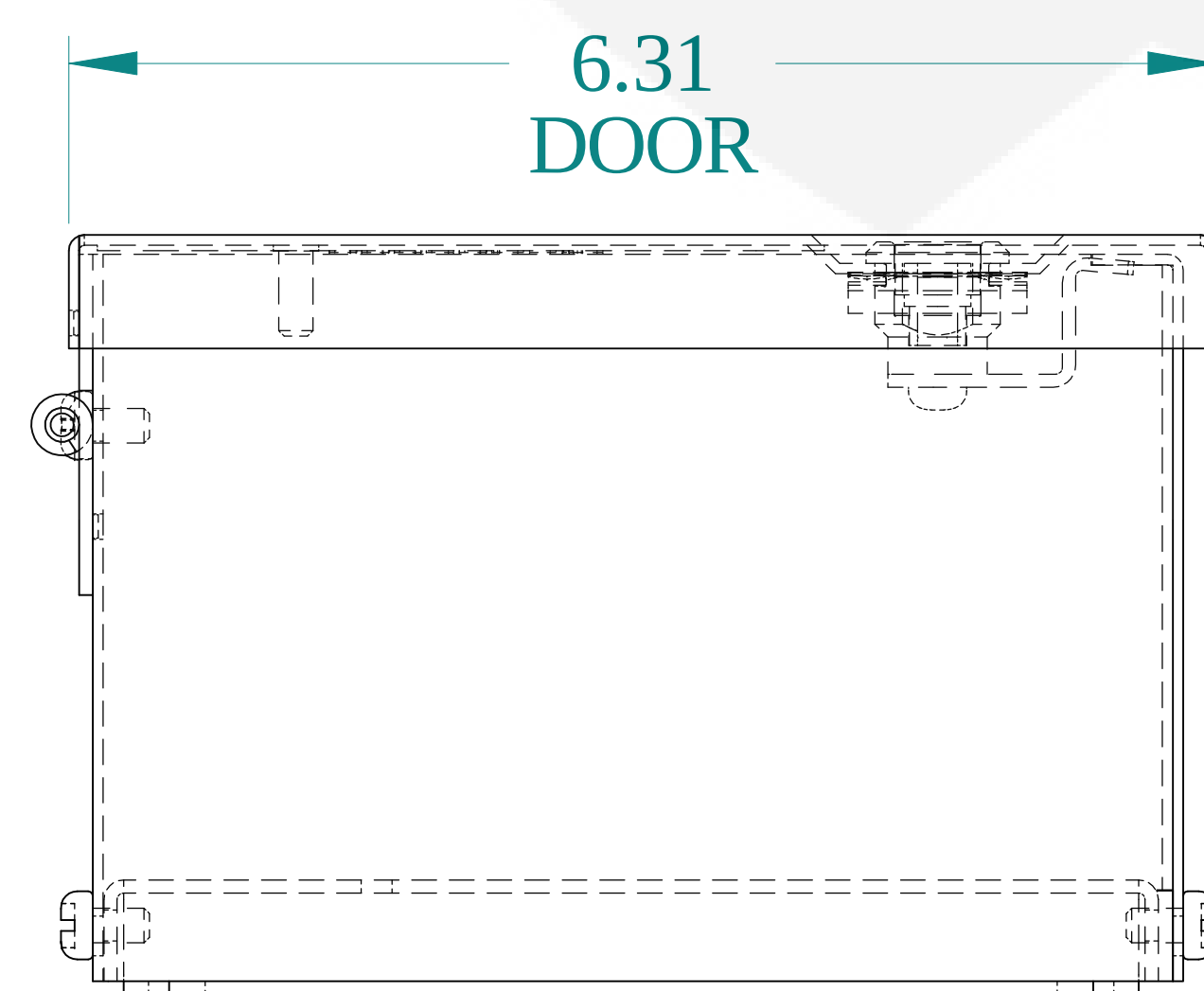
BOTTOM VIEW
