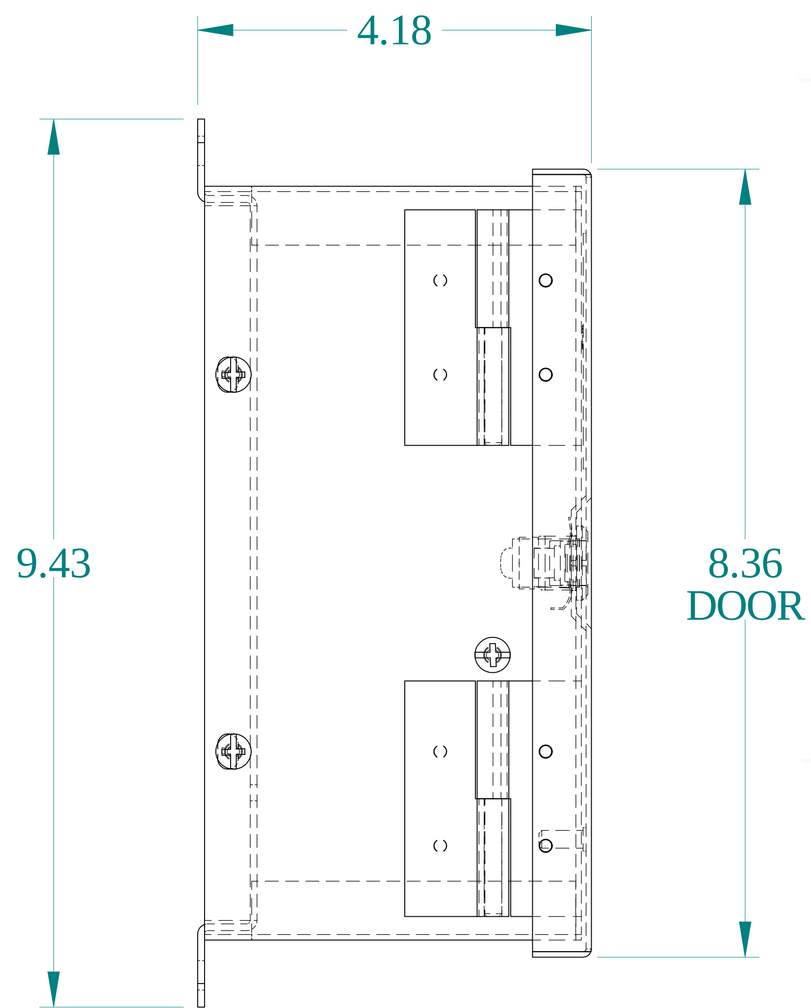
SIDE VIEW
