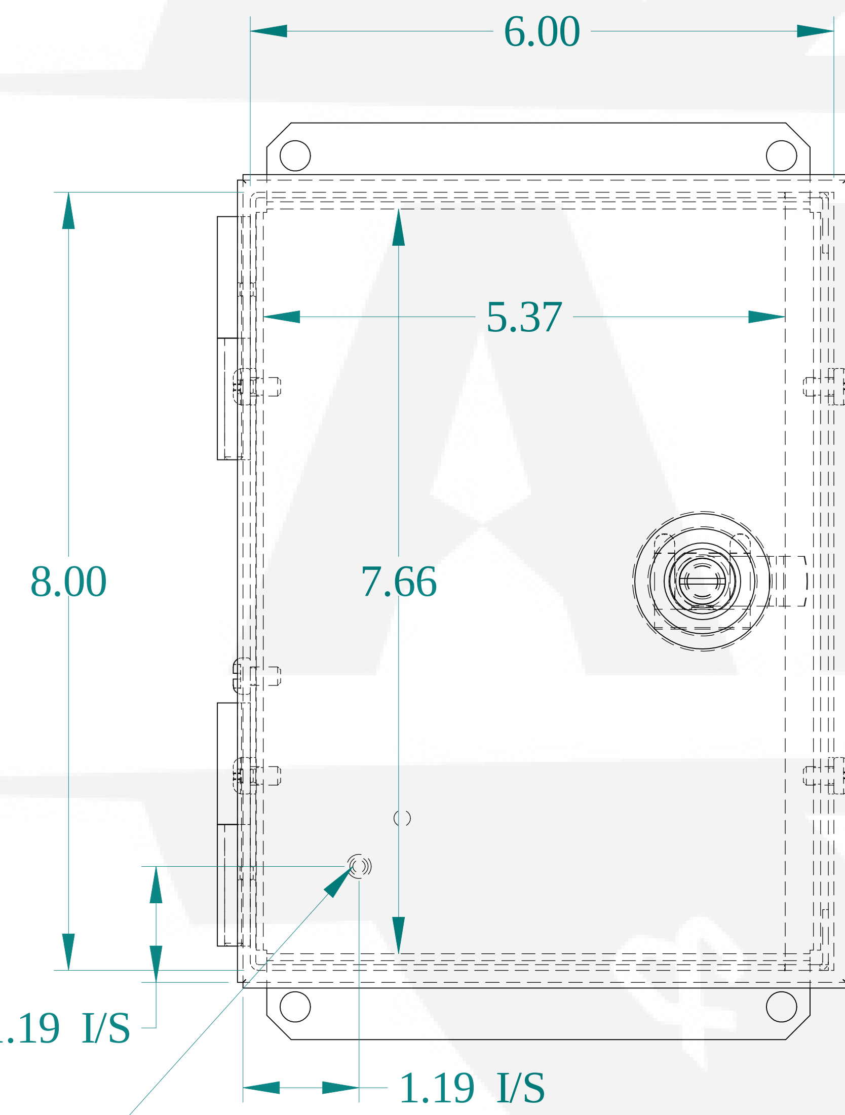
FRONT VIEW
