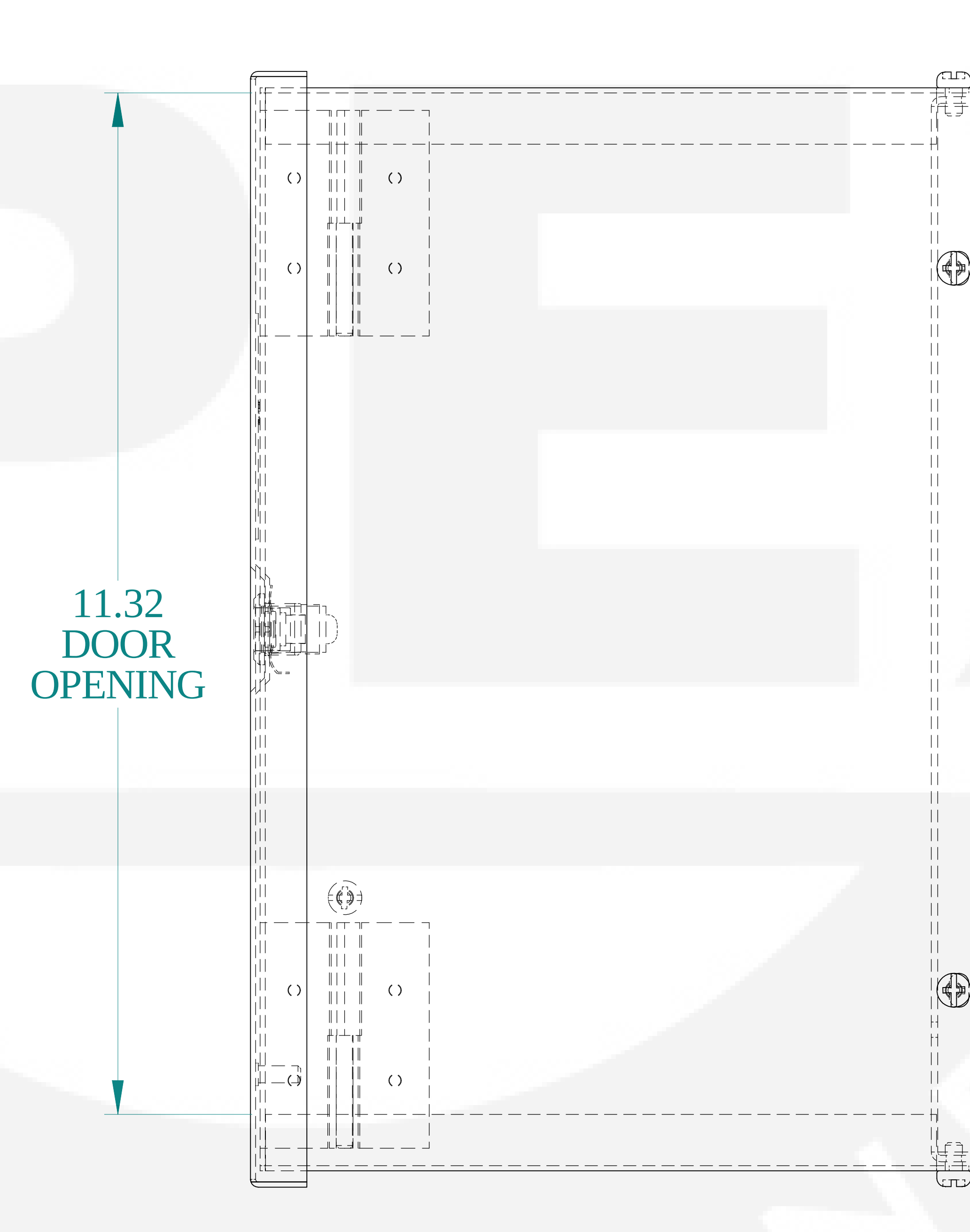
SIDE VIEW
