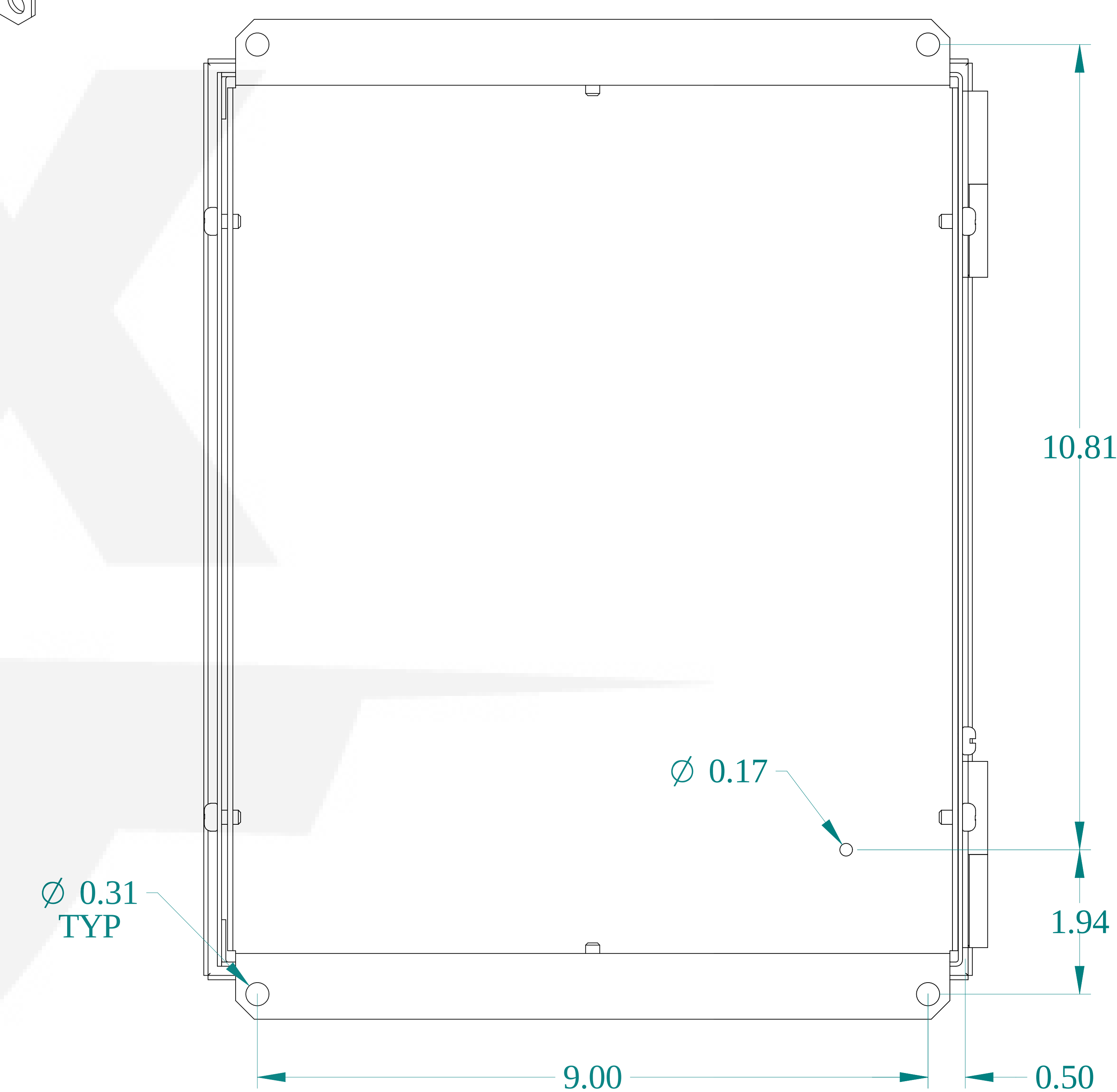
BACK VIEW
