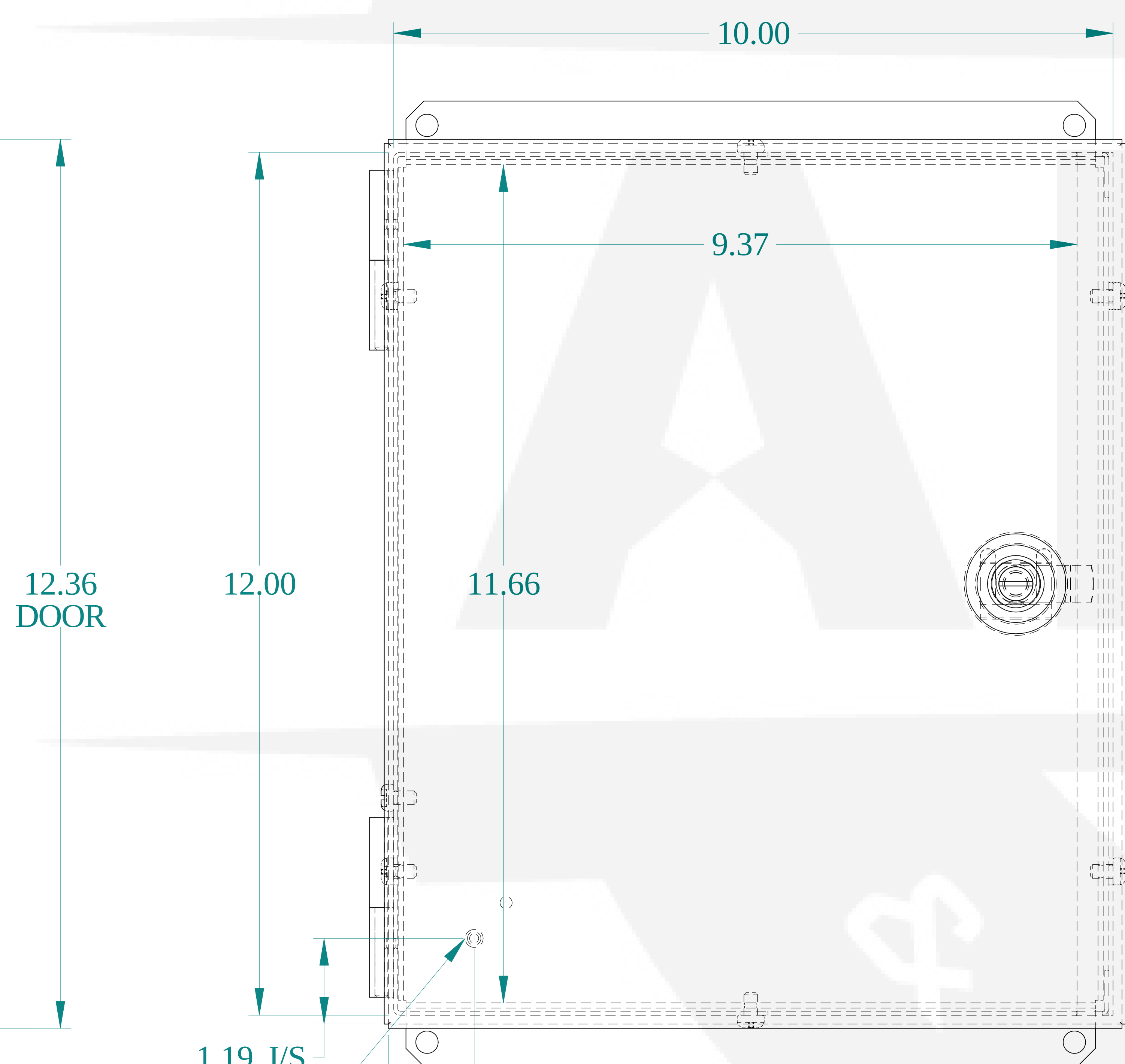
FRONT VIEW
