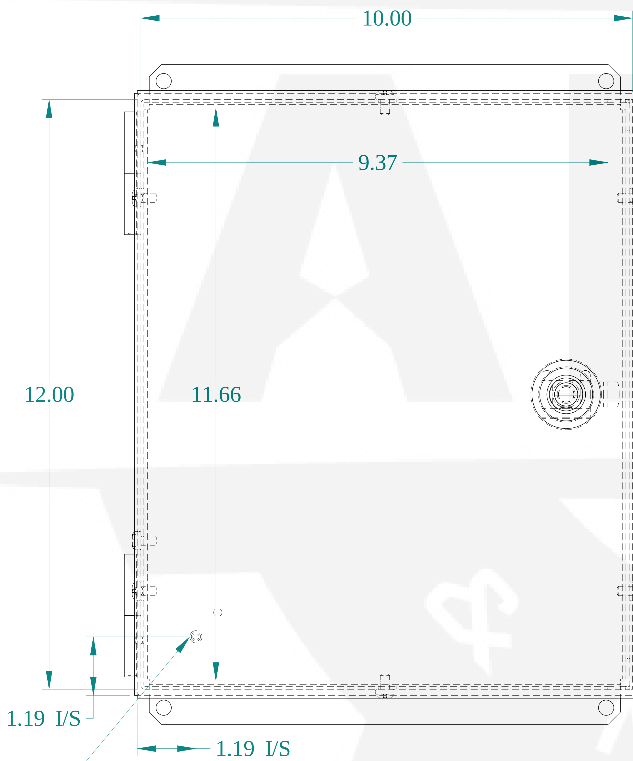
FRONT VIEW
