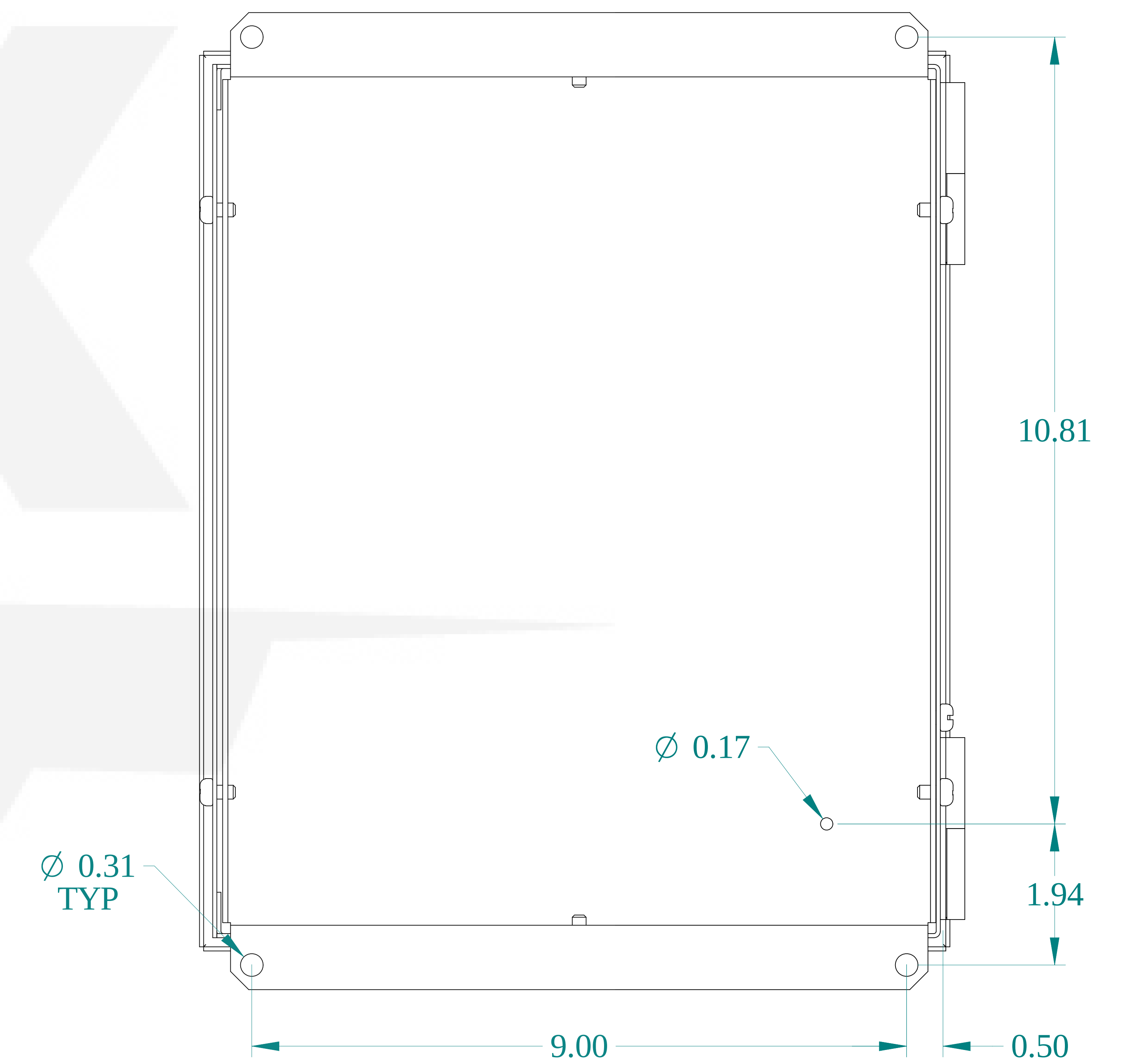
BACK VIEW
