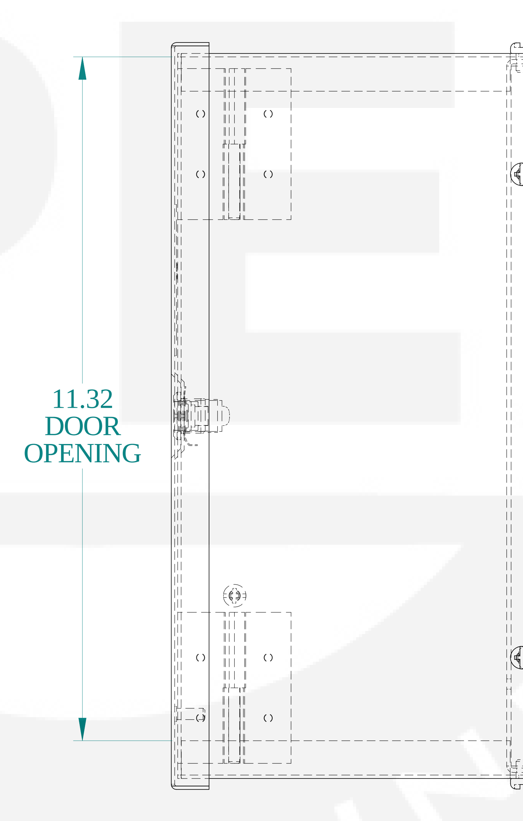
SIDE VIEW
