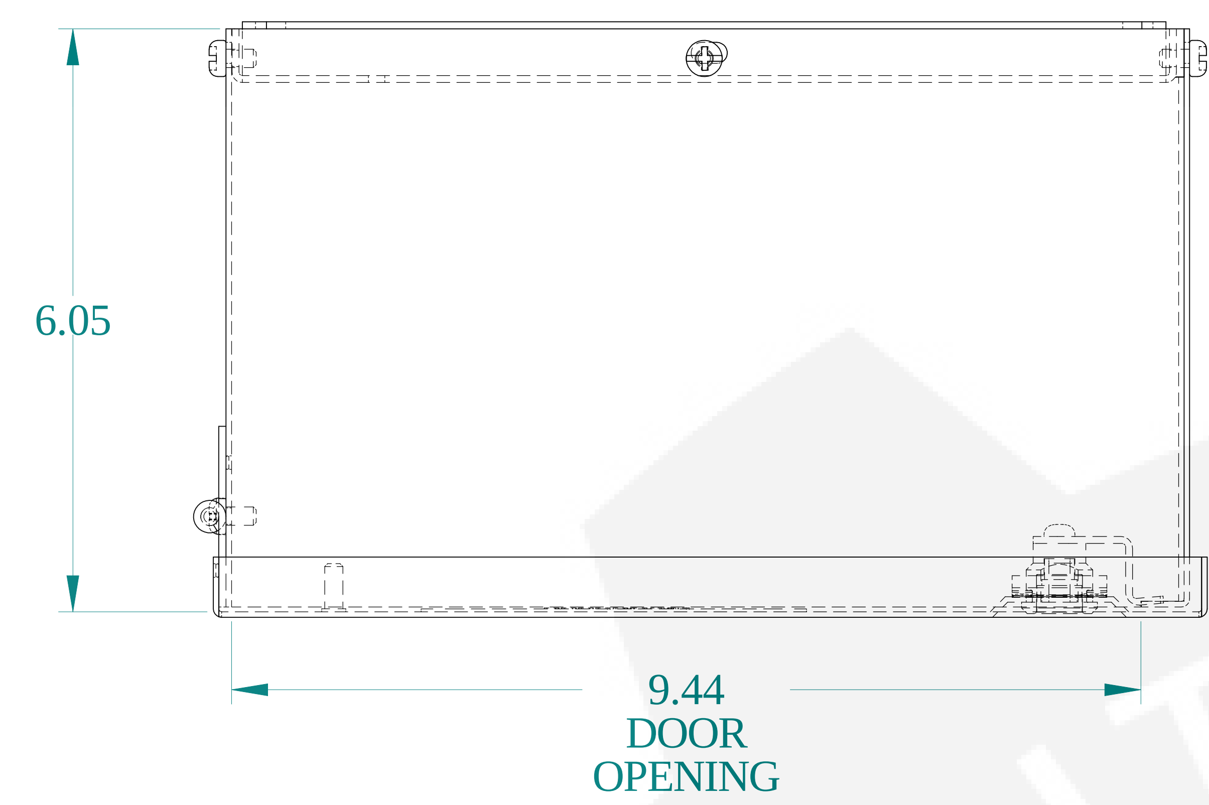
TOP VIEW
