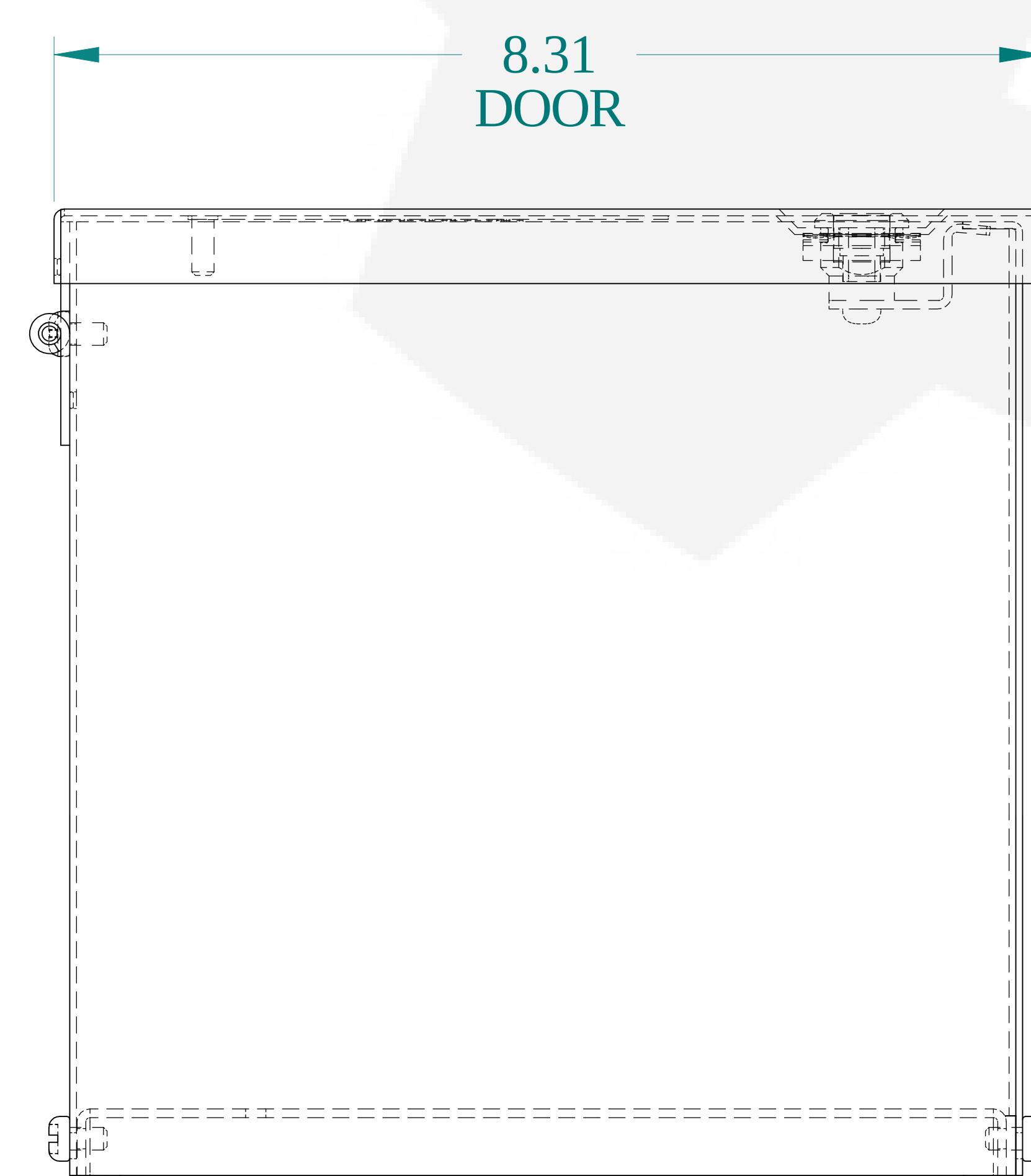
BOTTOM VIEW
