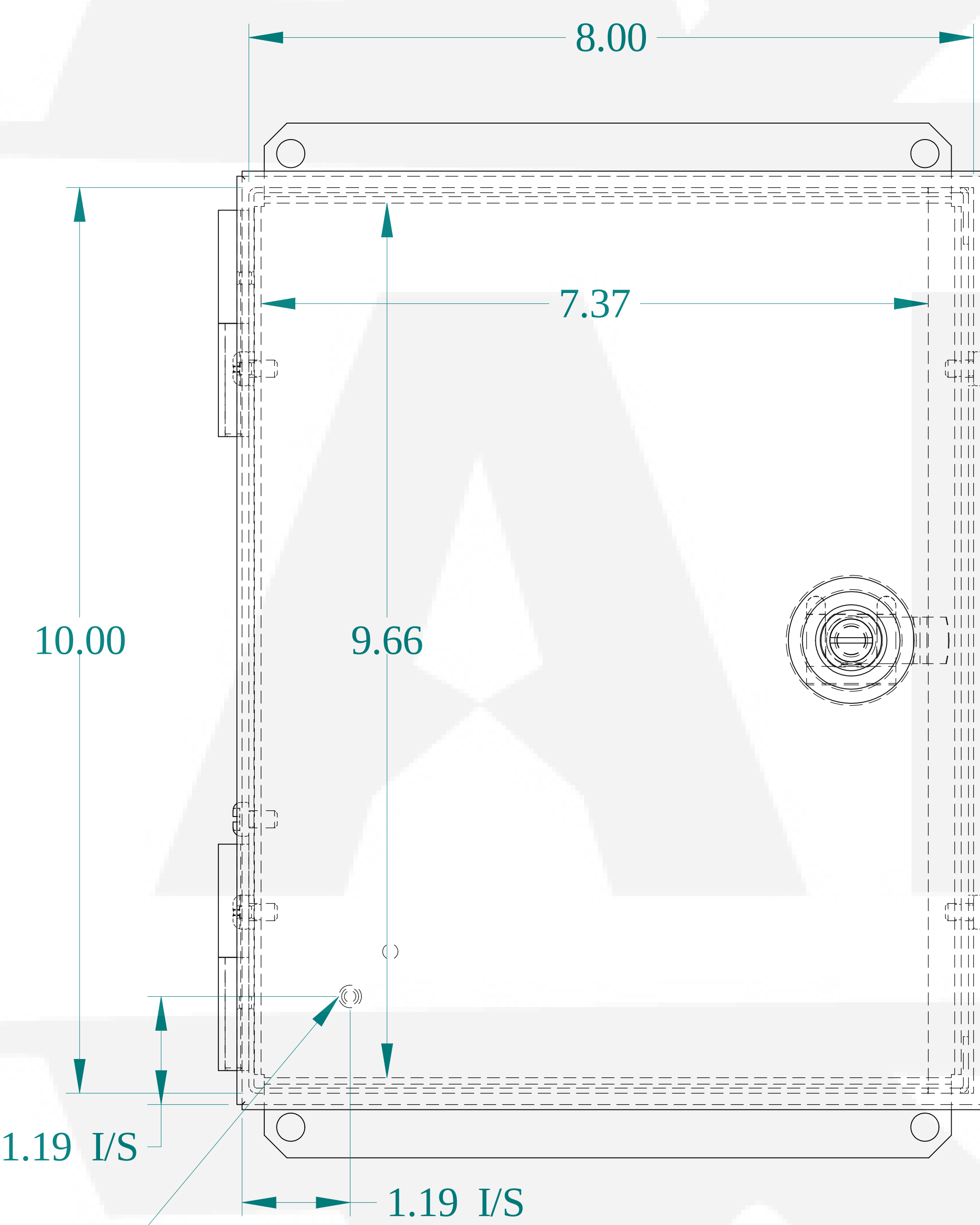
FRONT VIEW
