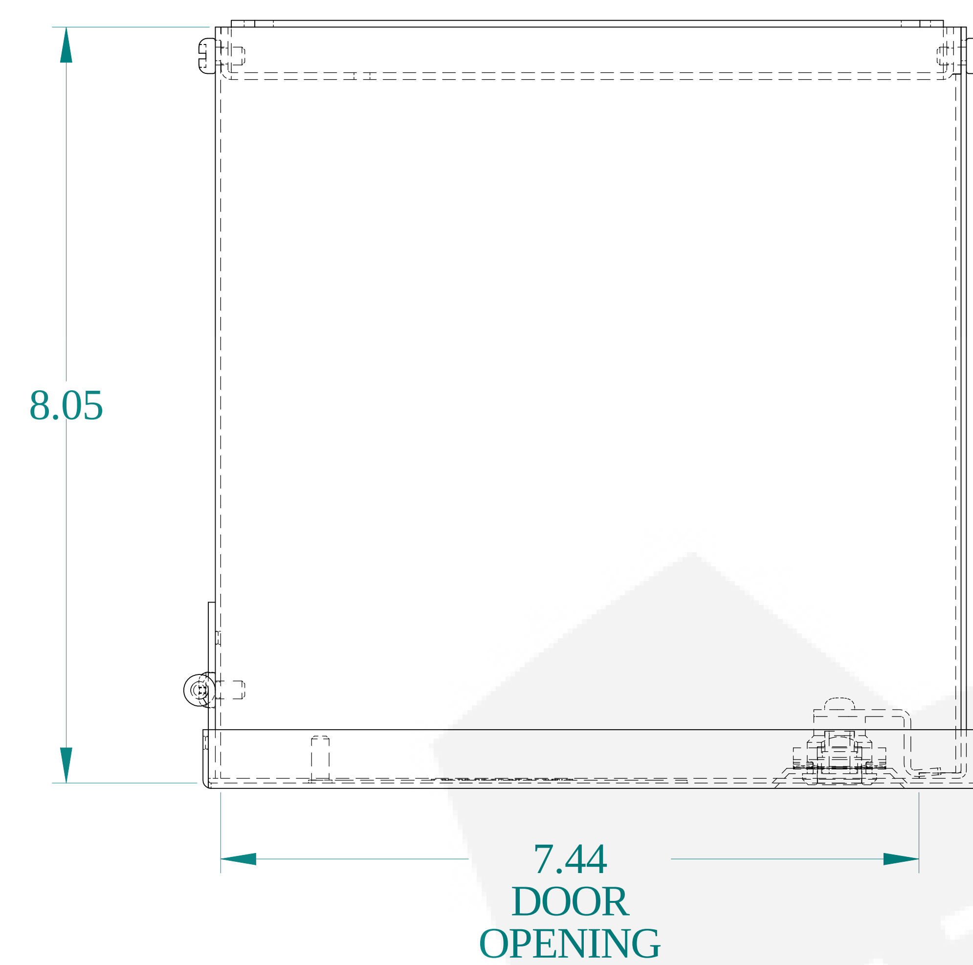
TOP VIEW
