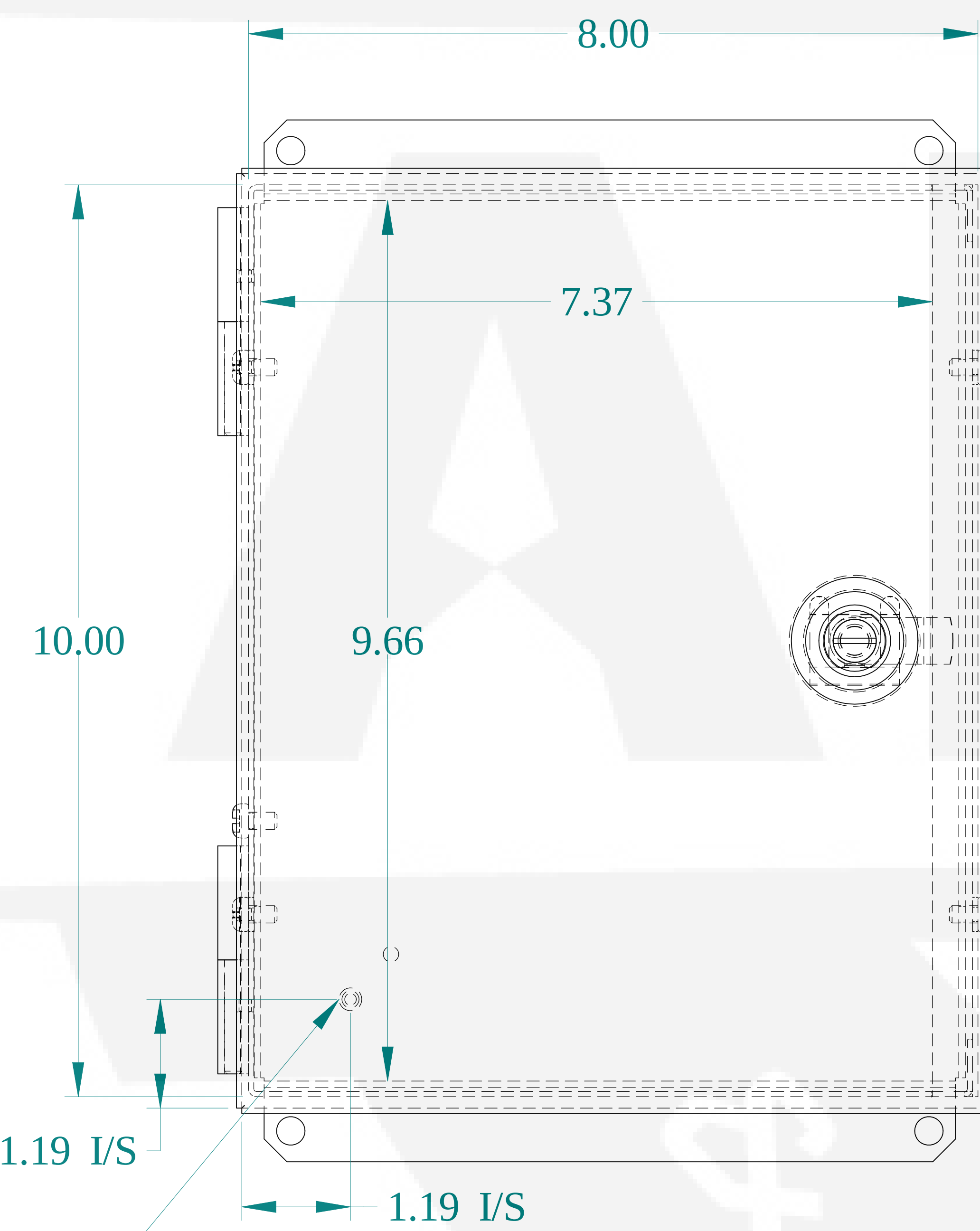
FRONT VIEW
