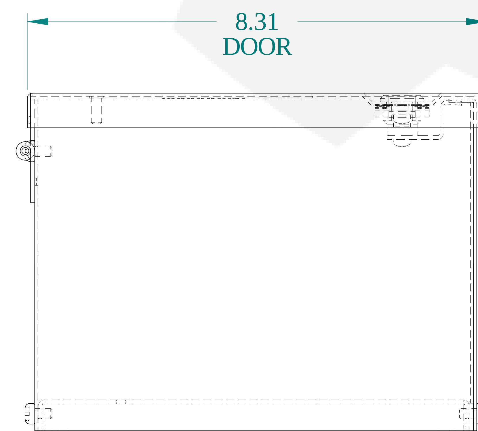
BOTTOM VIEW
