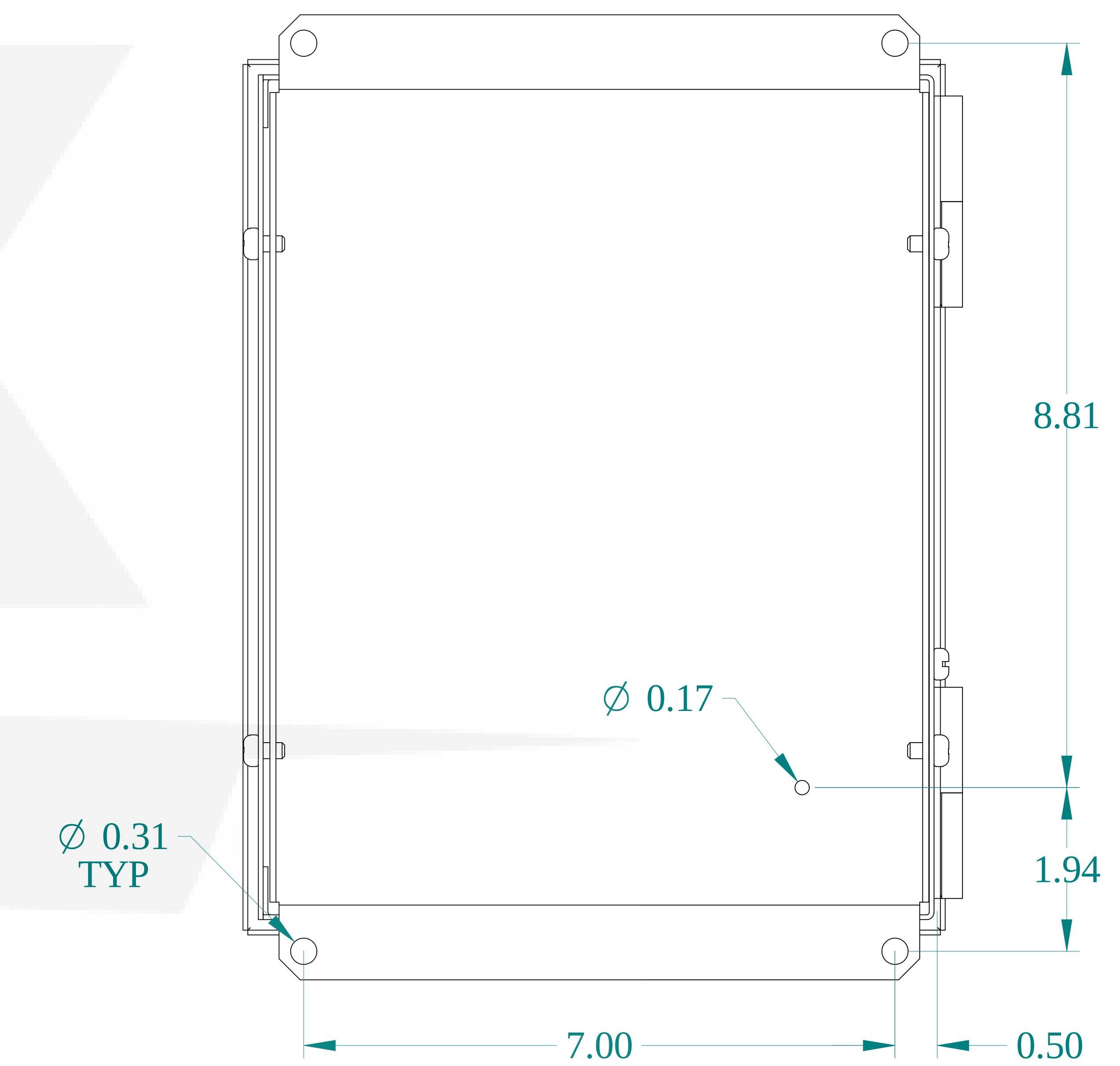
BACK VIEW
