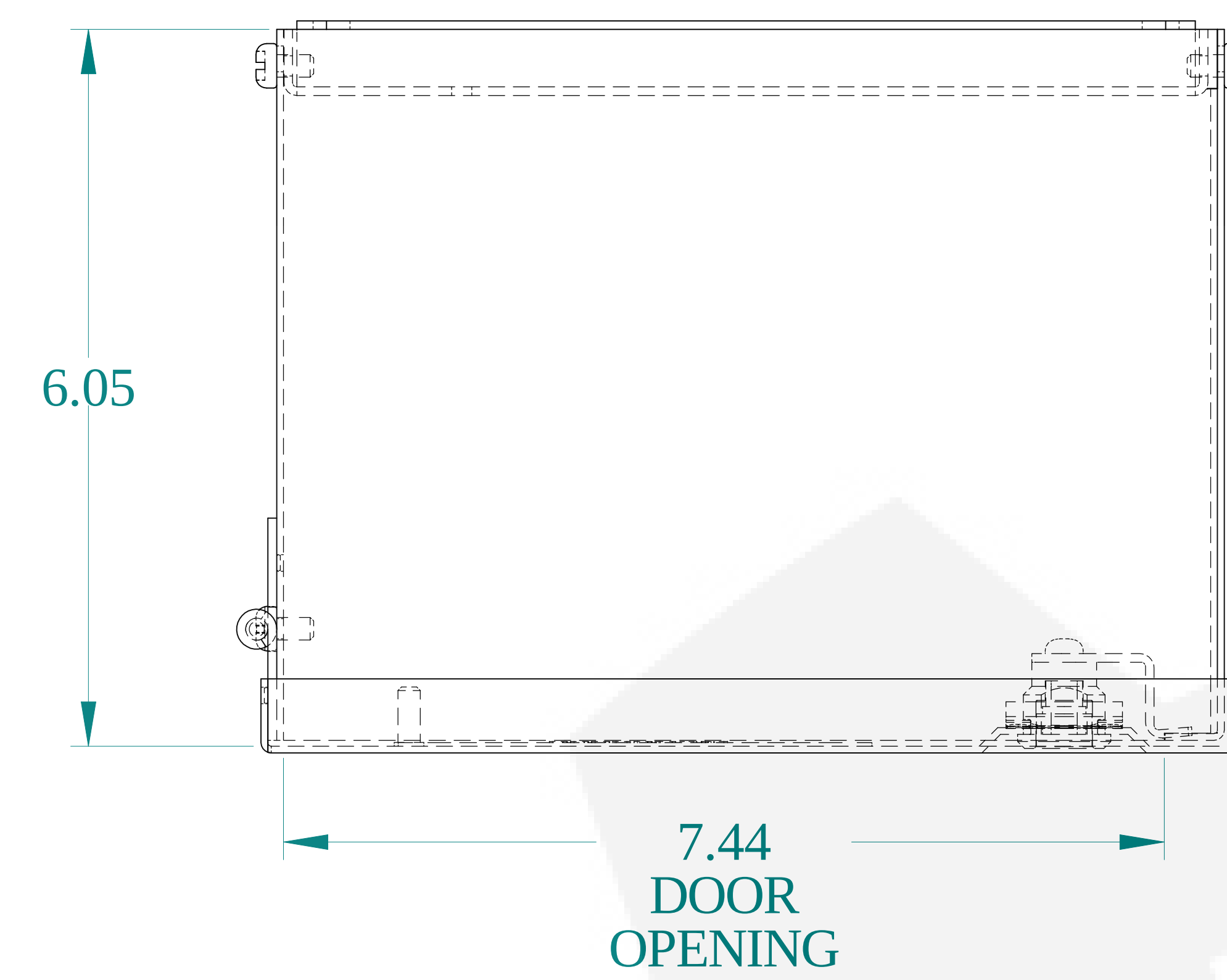
TOP VIEW
