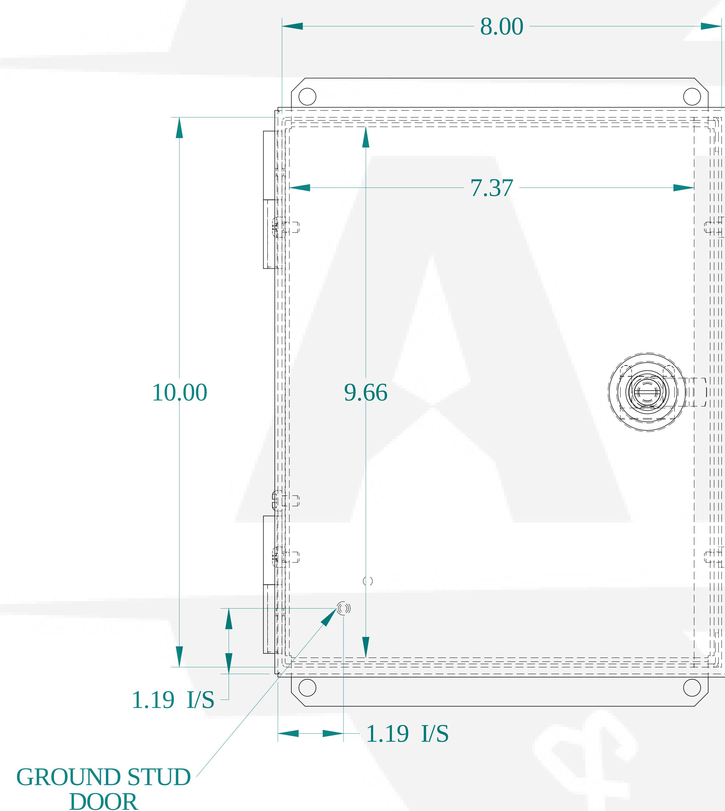
FRONT VIEW
