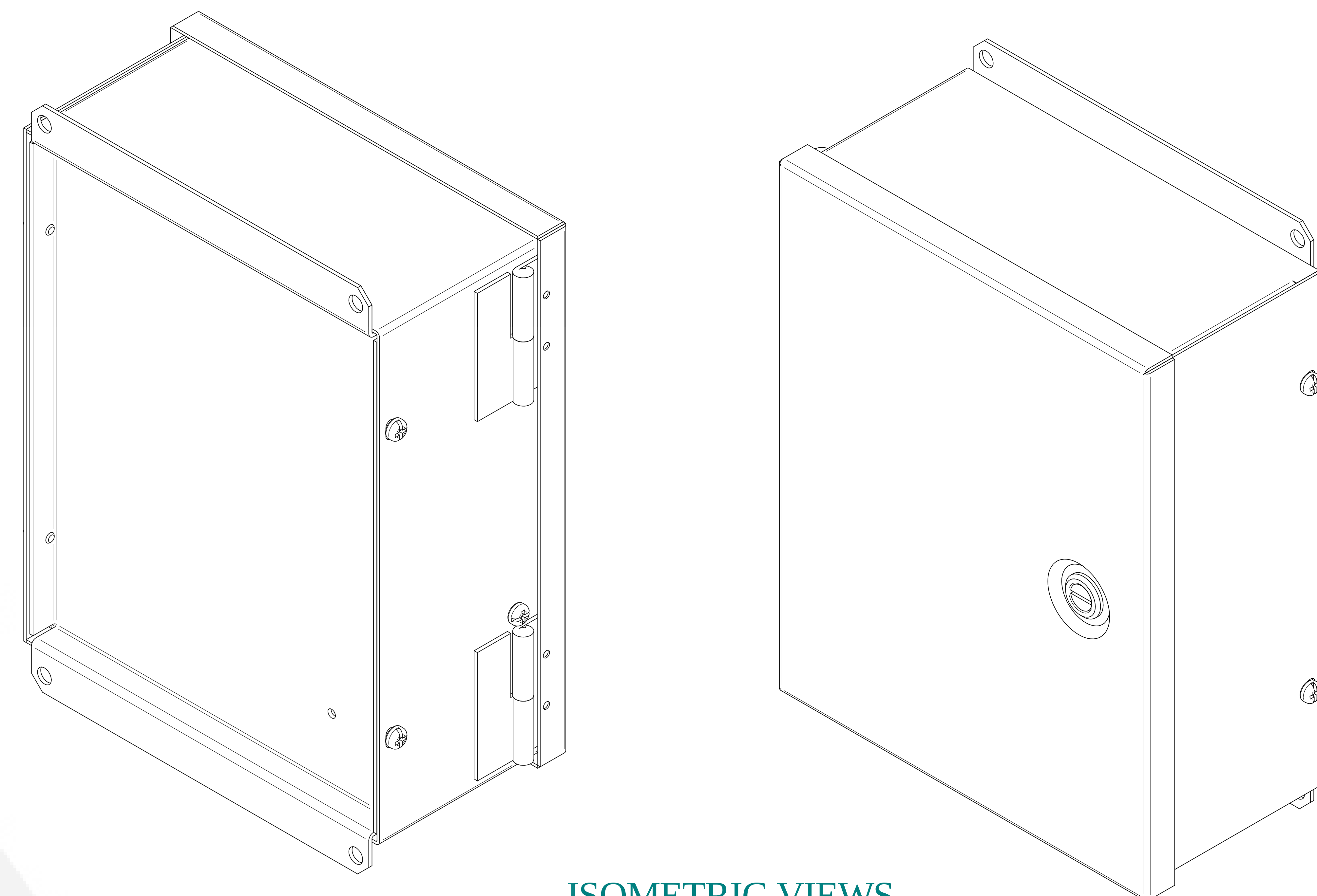
ISOMETRIC VIEWS
