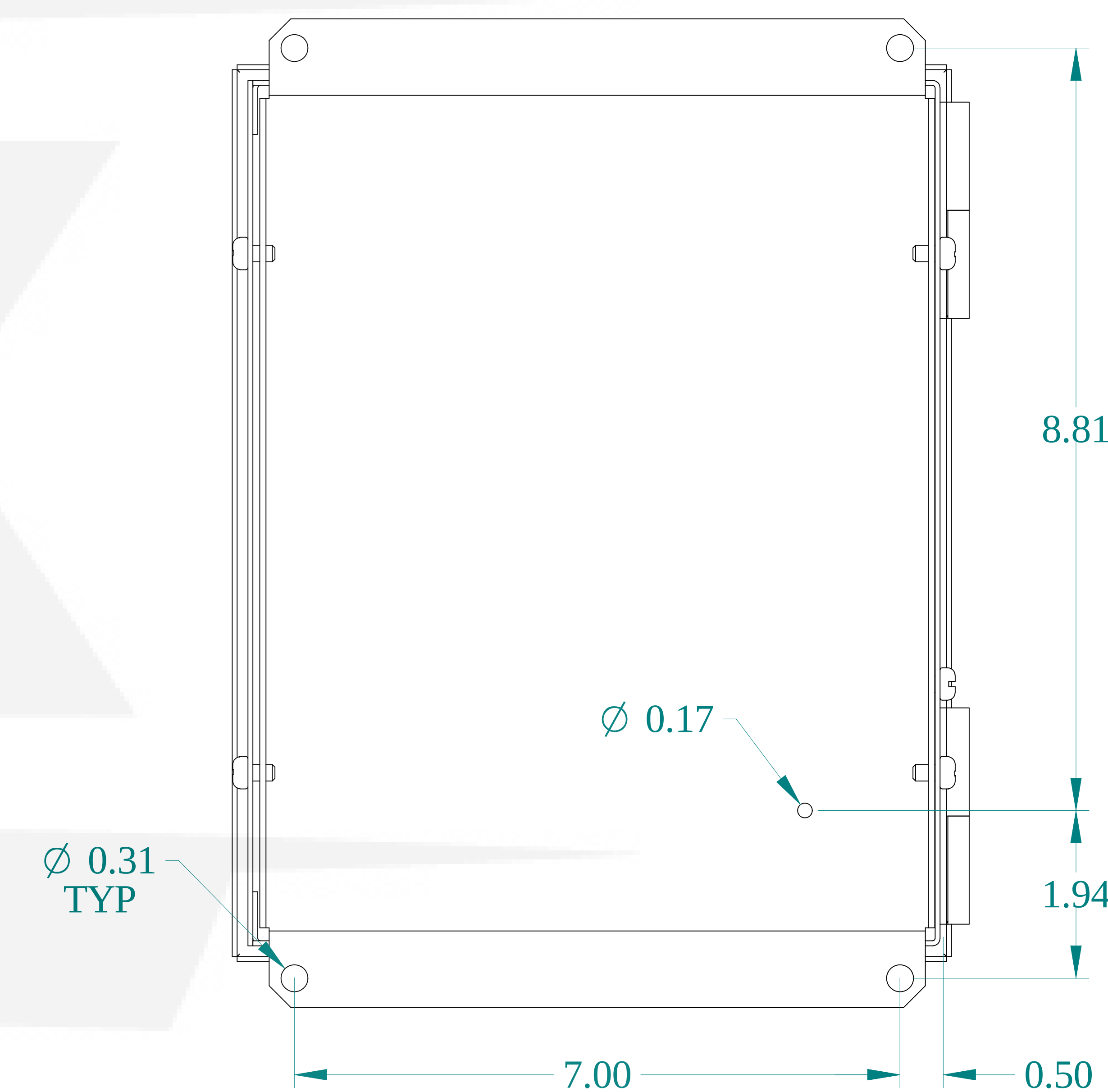
BACK VIEW
