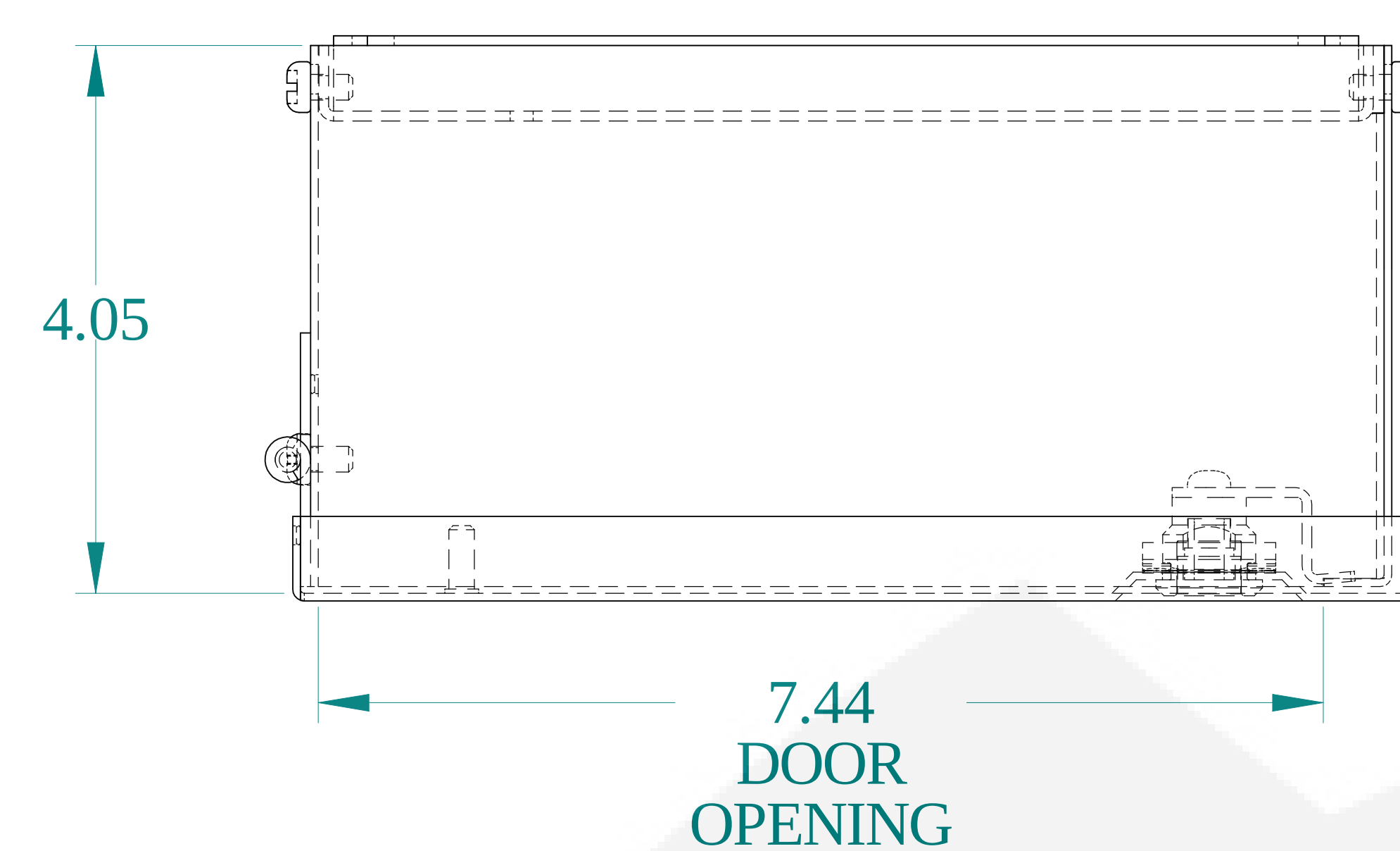
TOP VIEW
