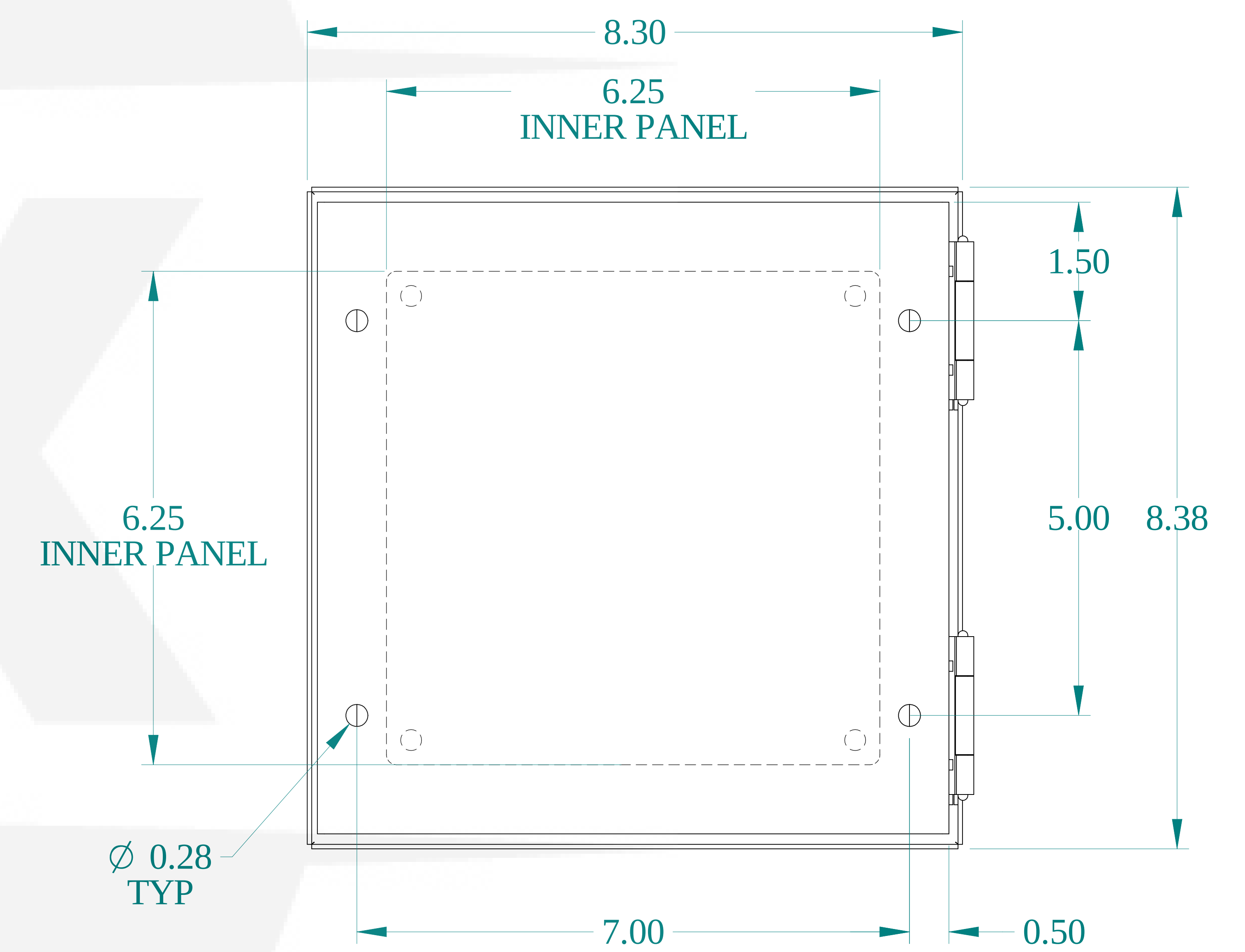
BACK VIEW
