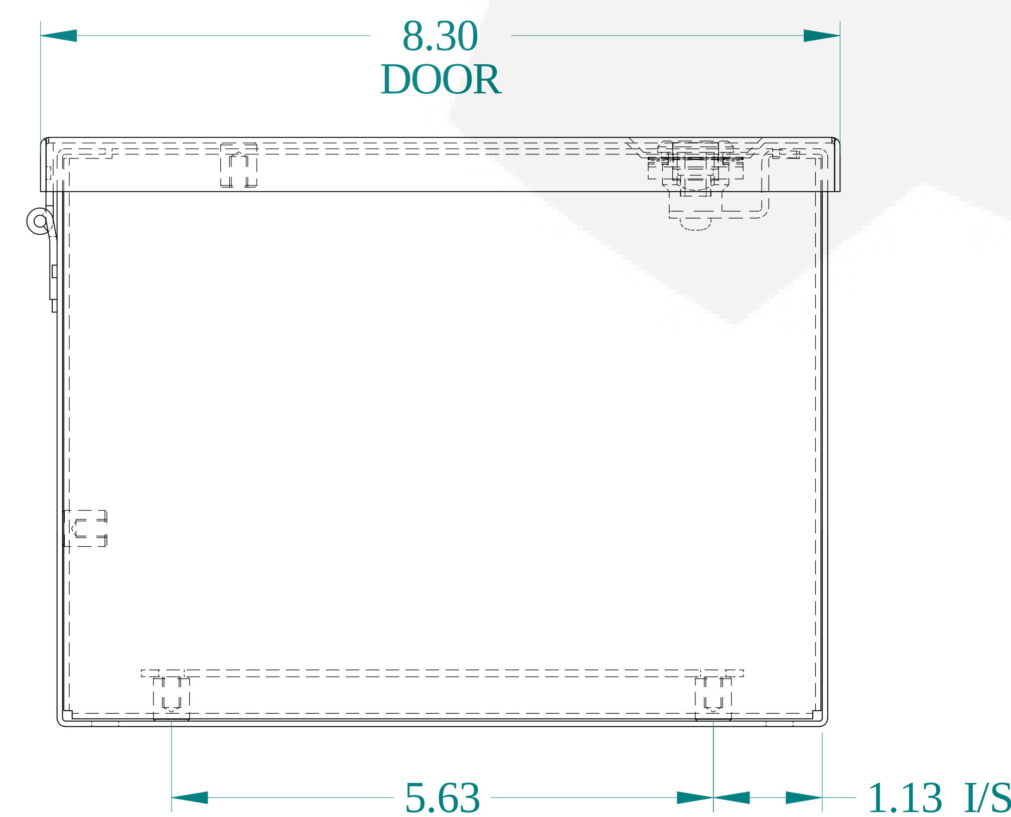
BOTTOM VIEW
