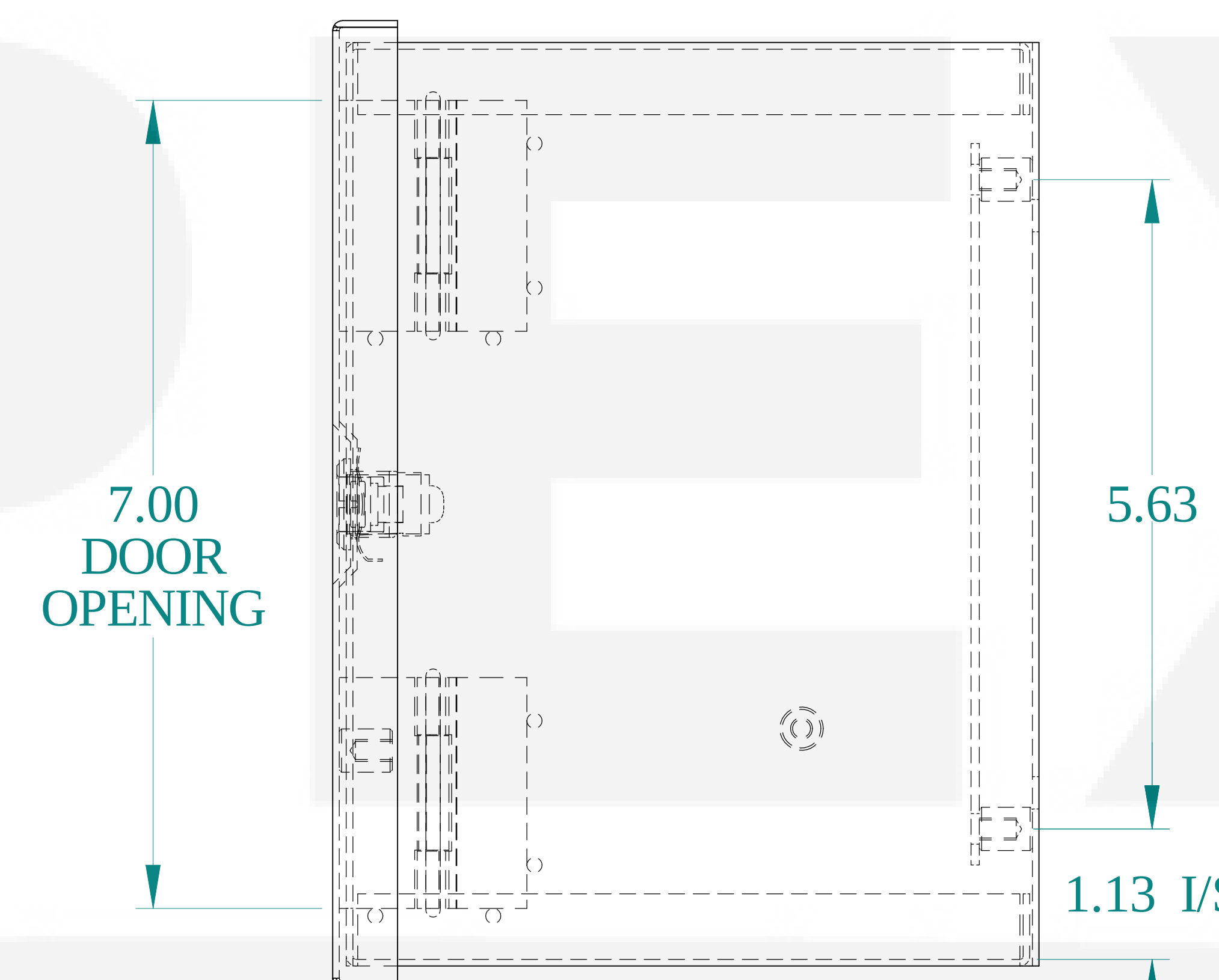
SIDE VIEW
