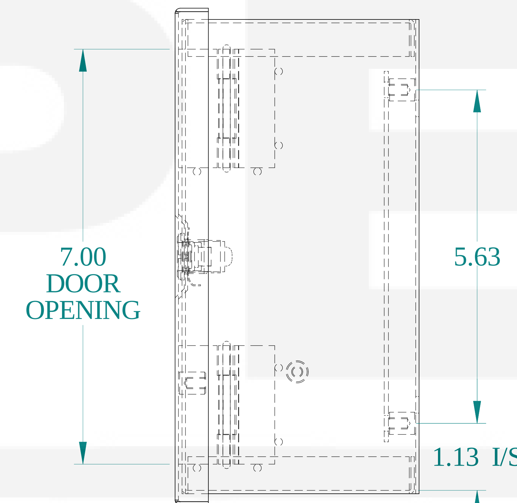
SIDE VIEW
