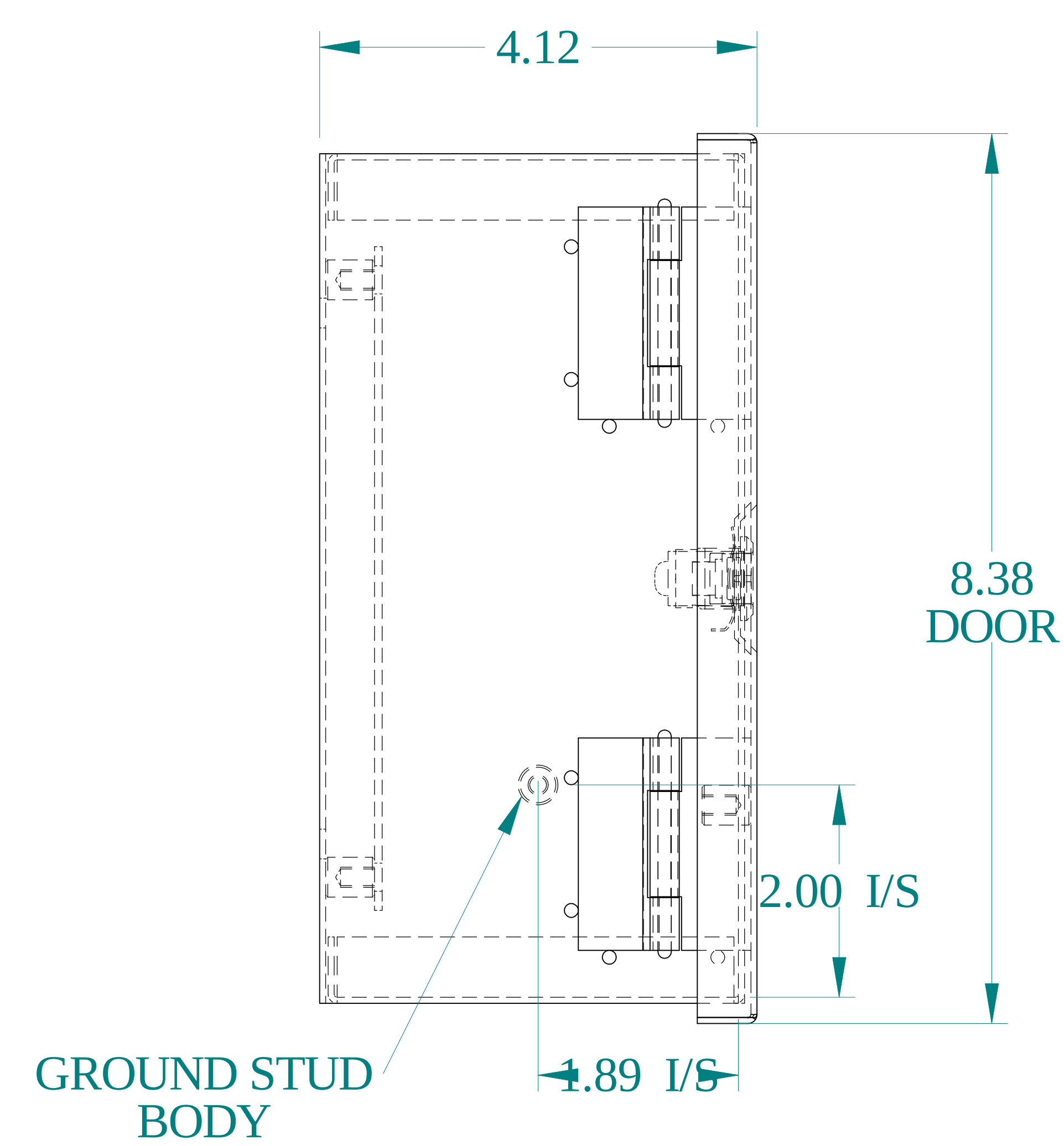
SIDE VIEW
