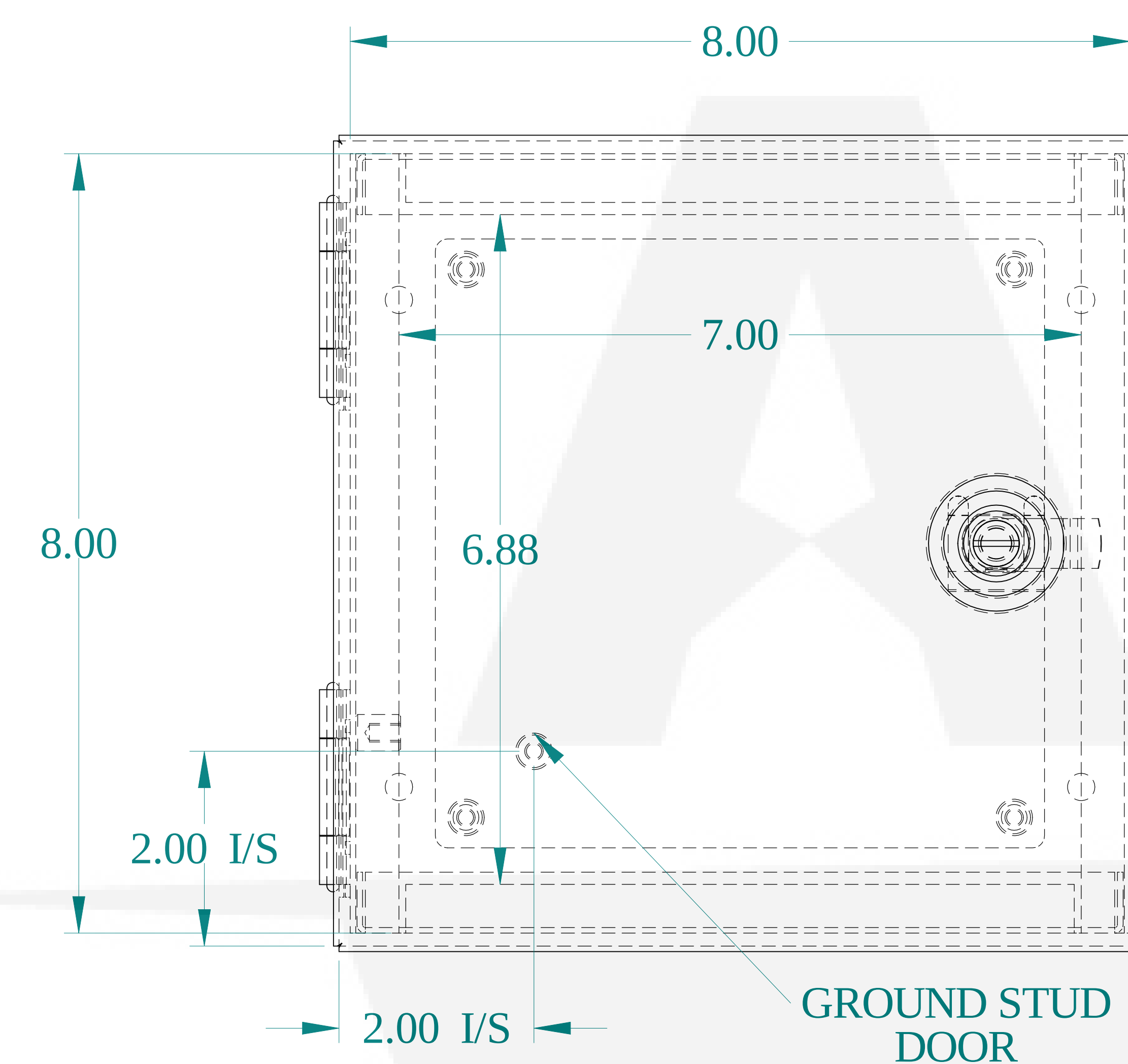
FRONT VIEW
