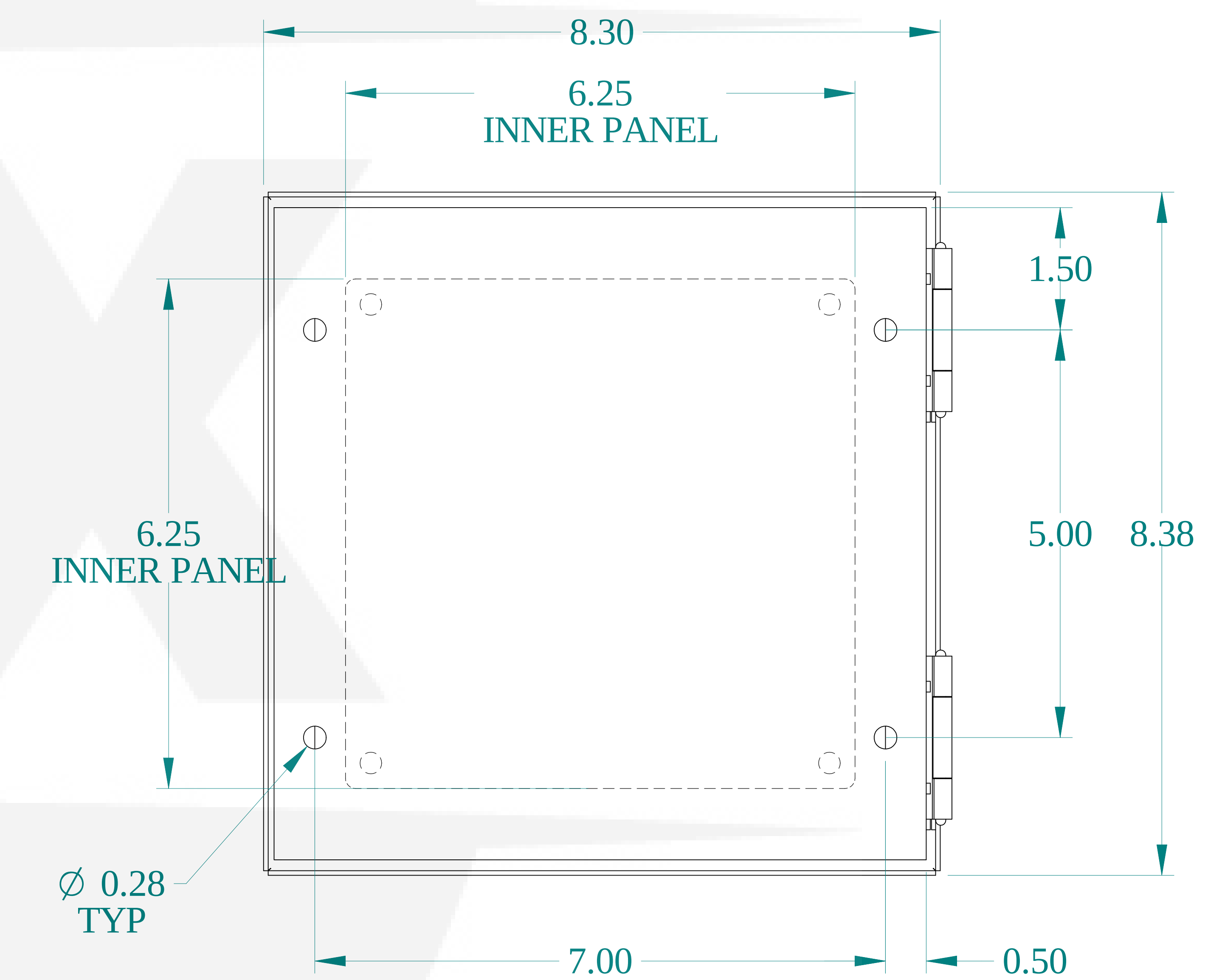
BACK VIEW
