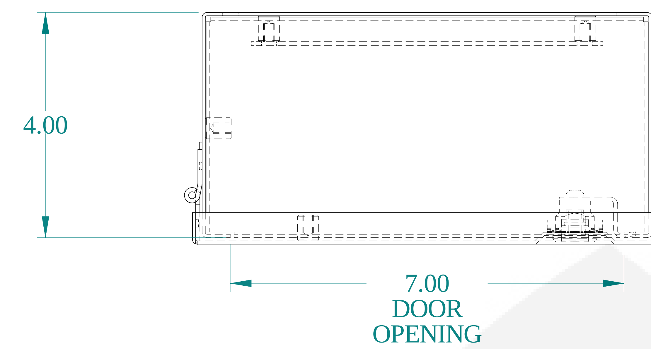
TOP VIEW
