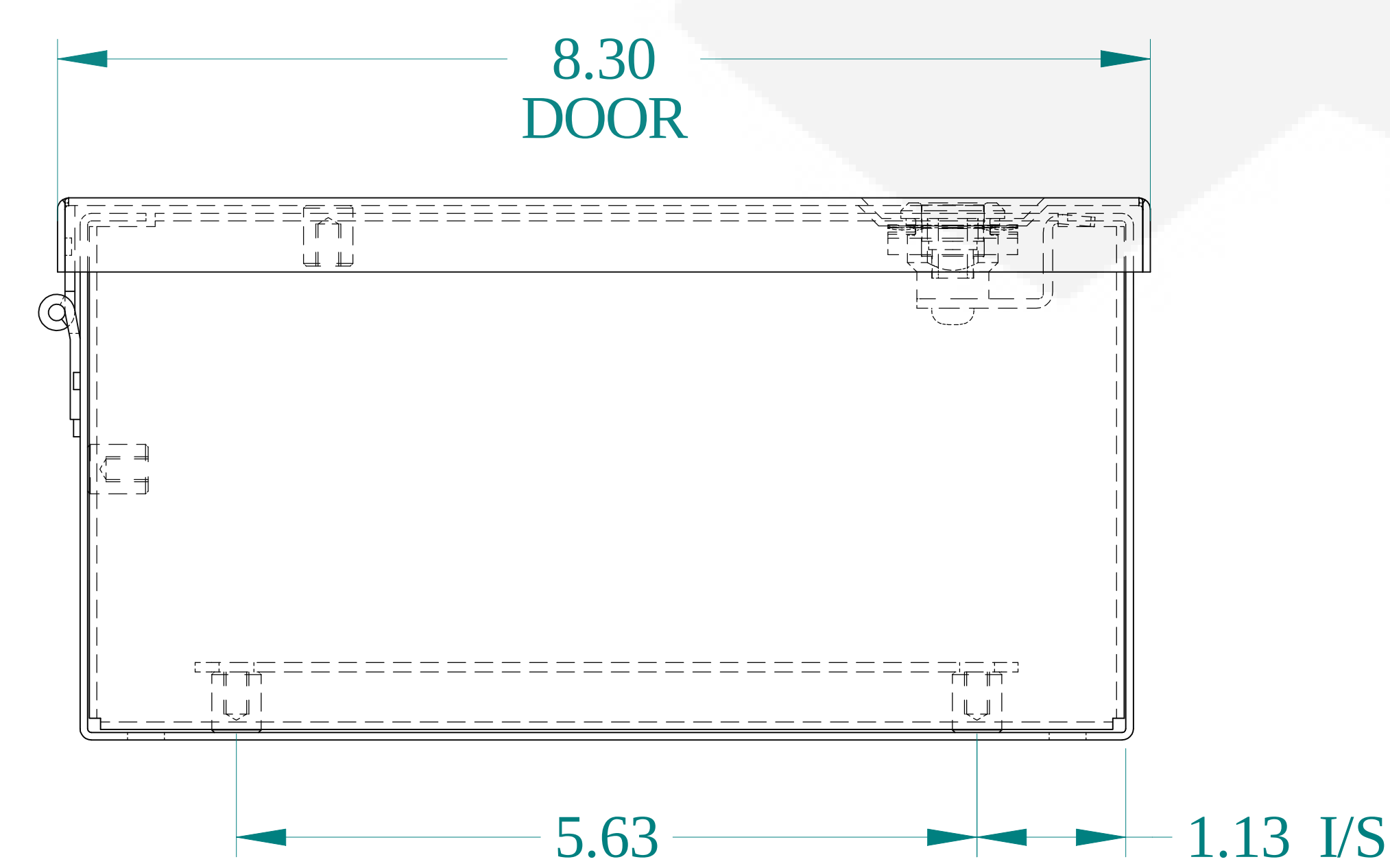
BOTTOM VIEW
