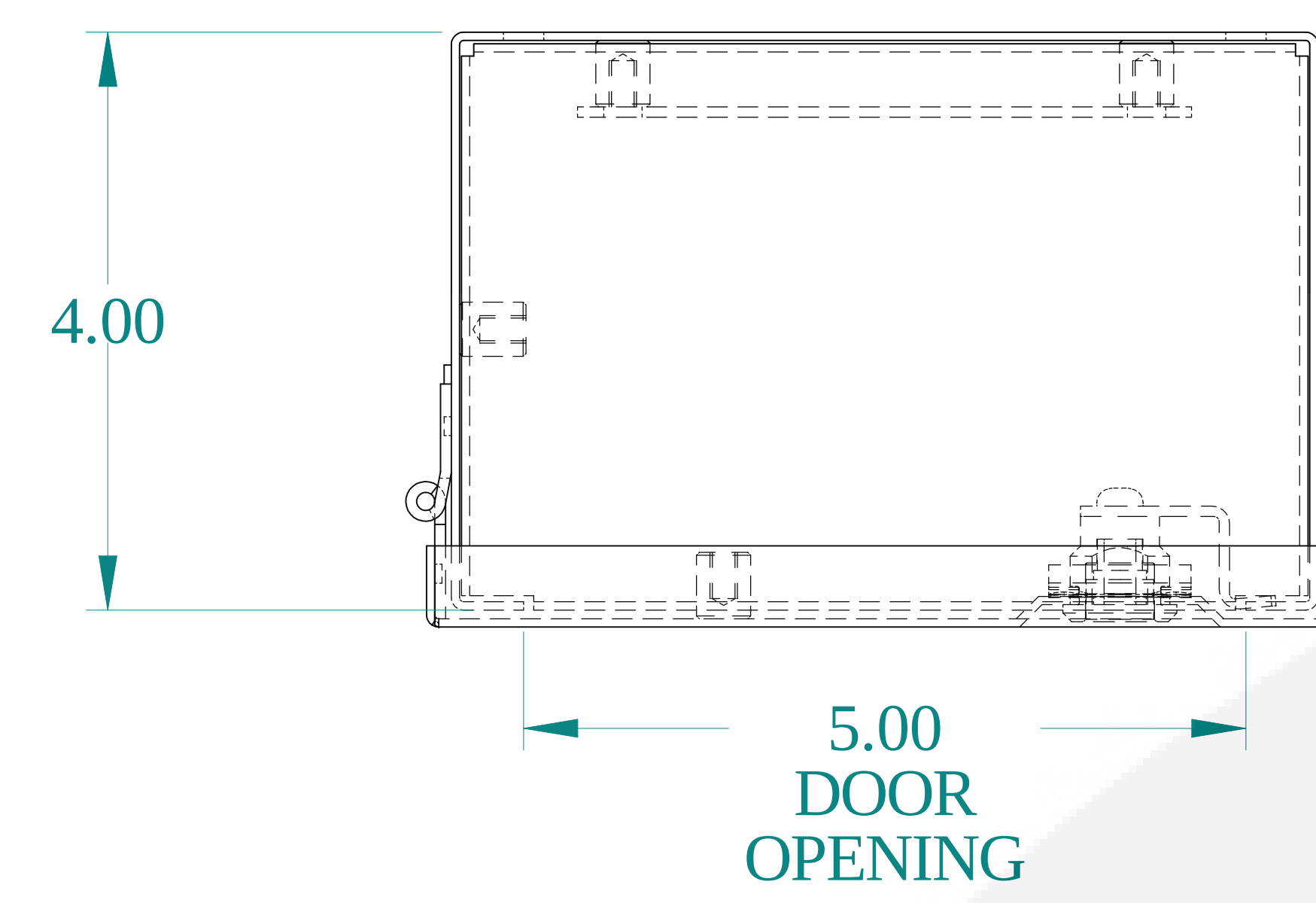
TOP VIEW
