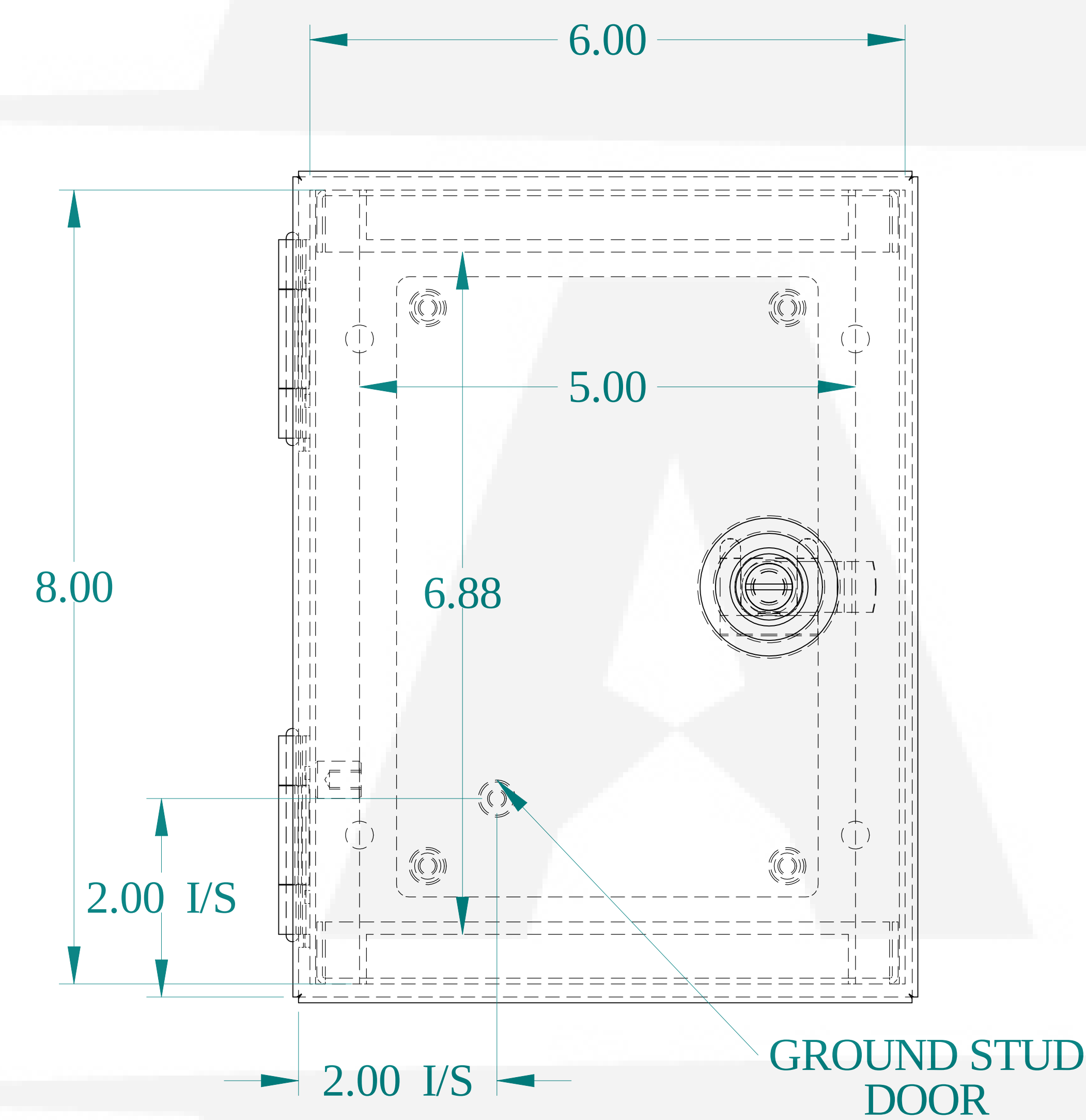
FRONT VIEW
