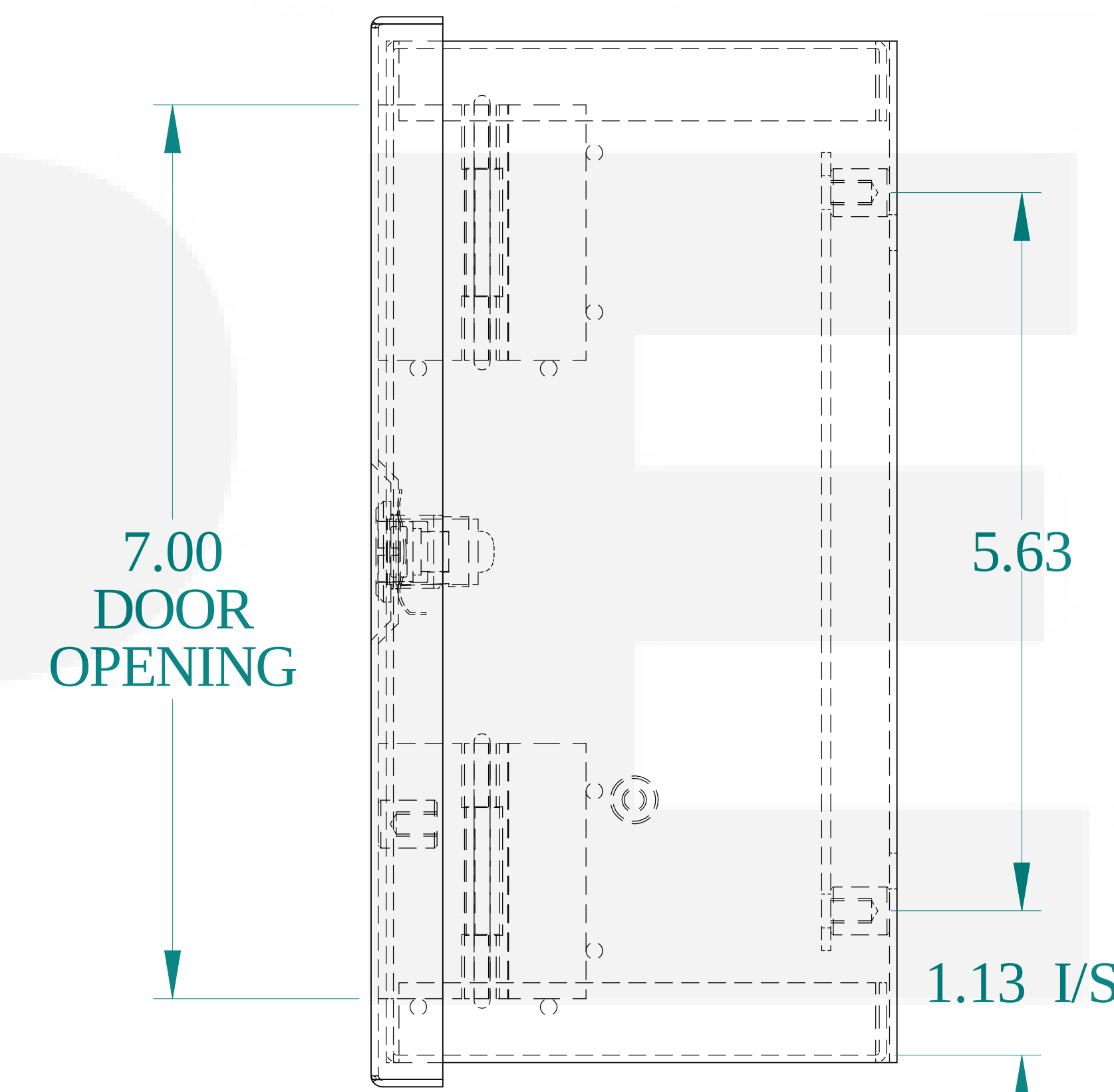
SIDE VIEW
