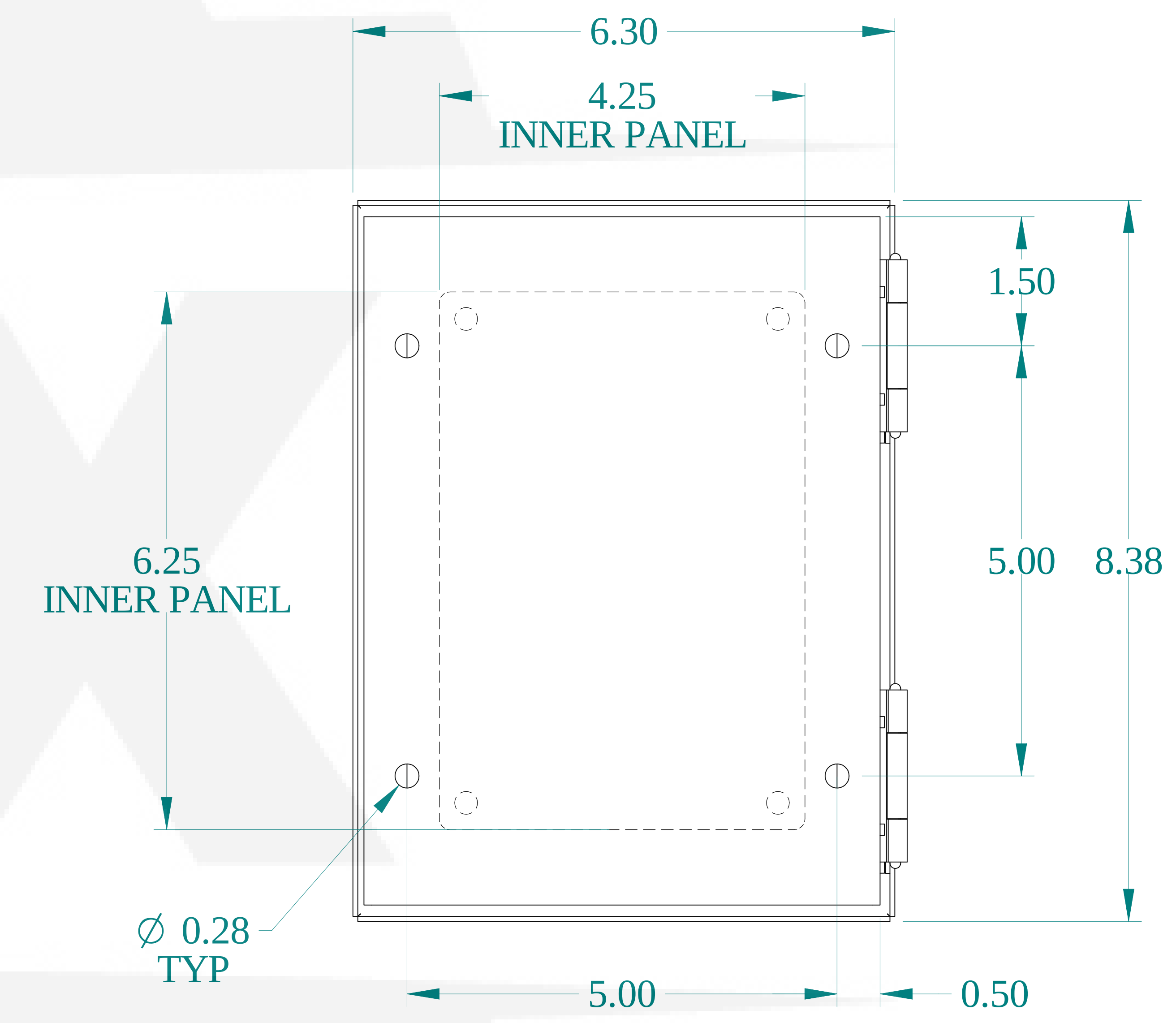
BACK VIEW
