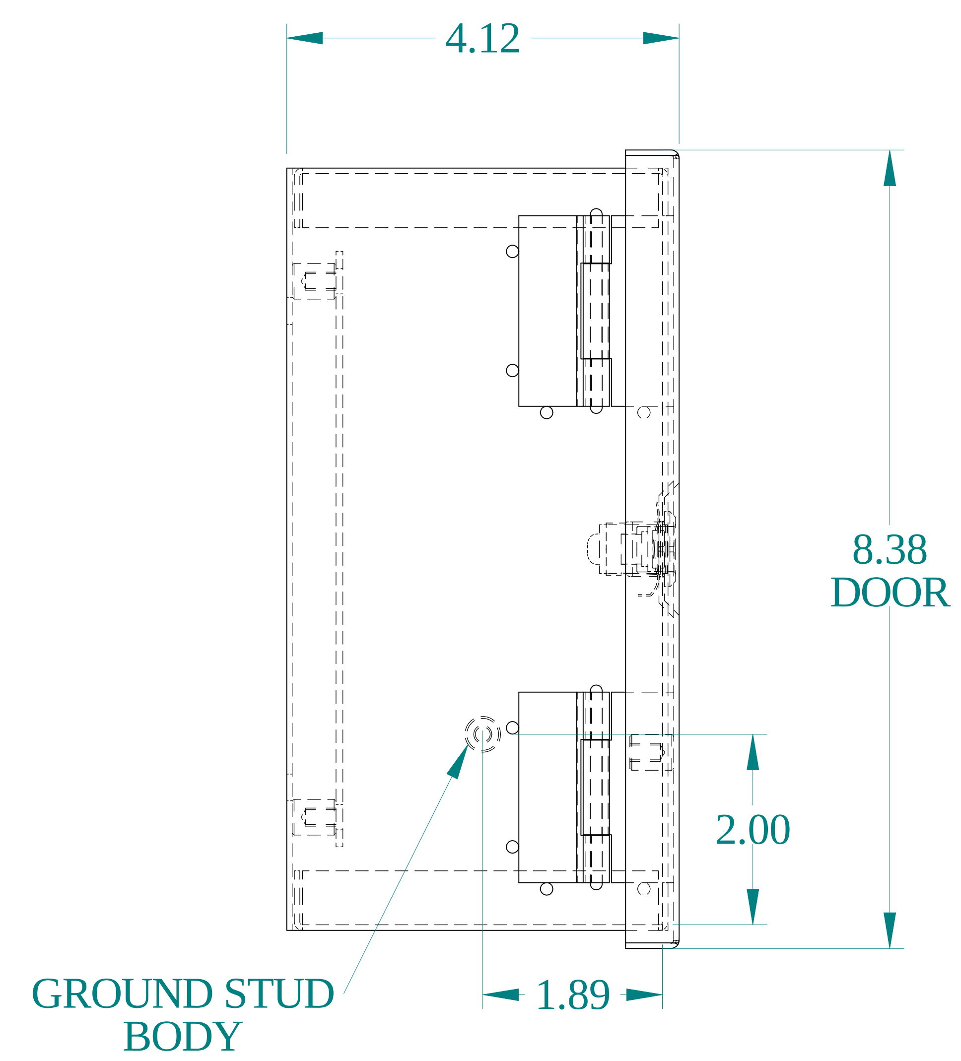
SIDE VIEW
