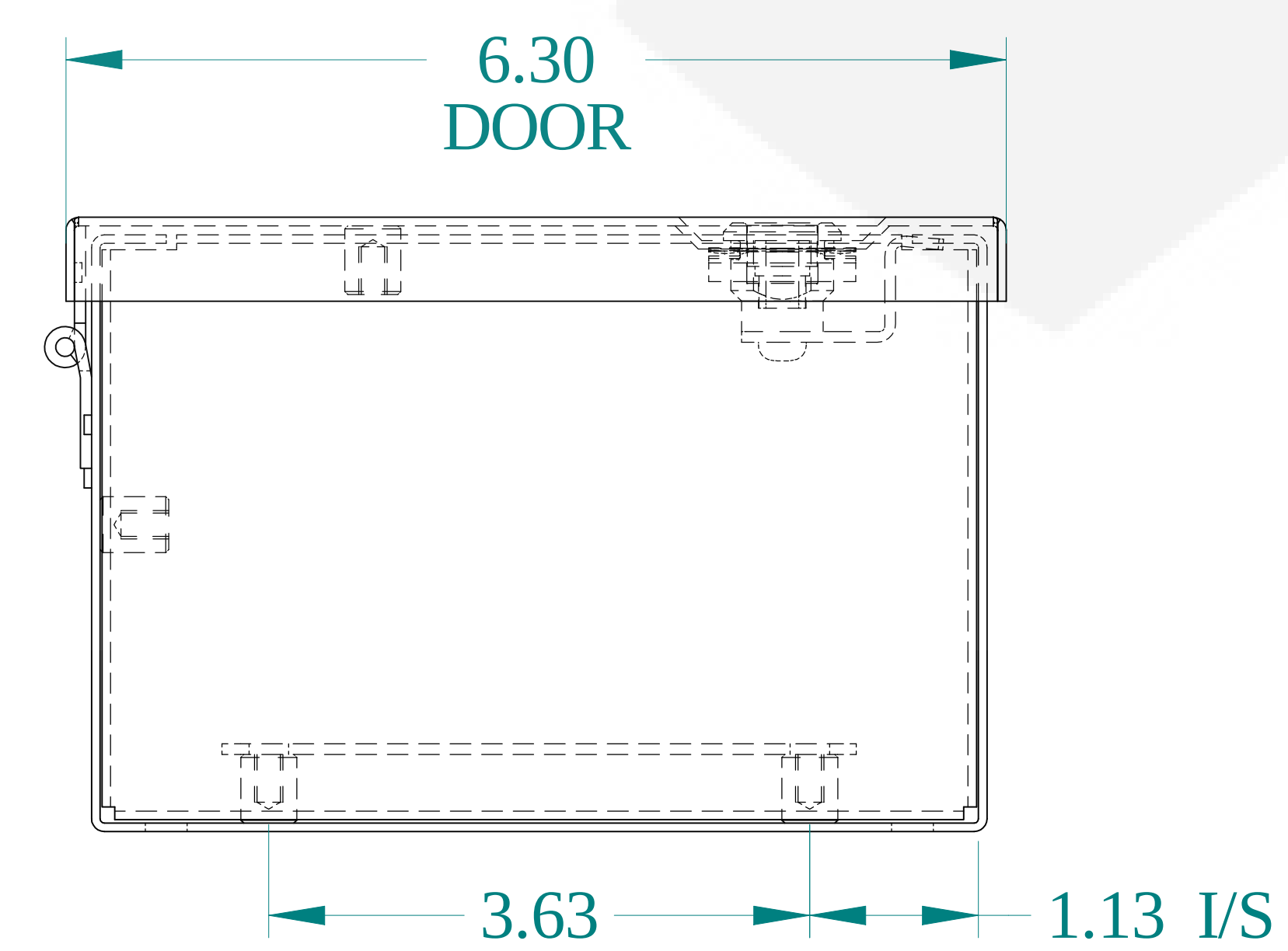
BOTTOM VIEW
