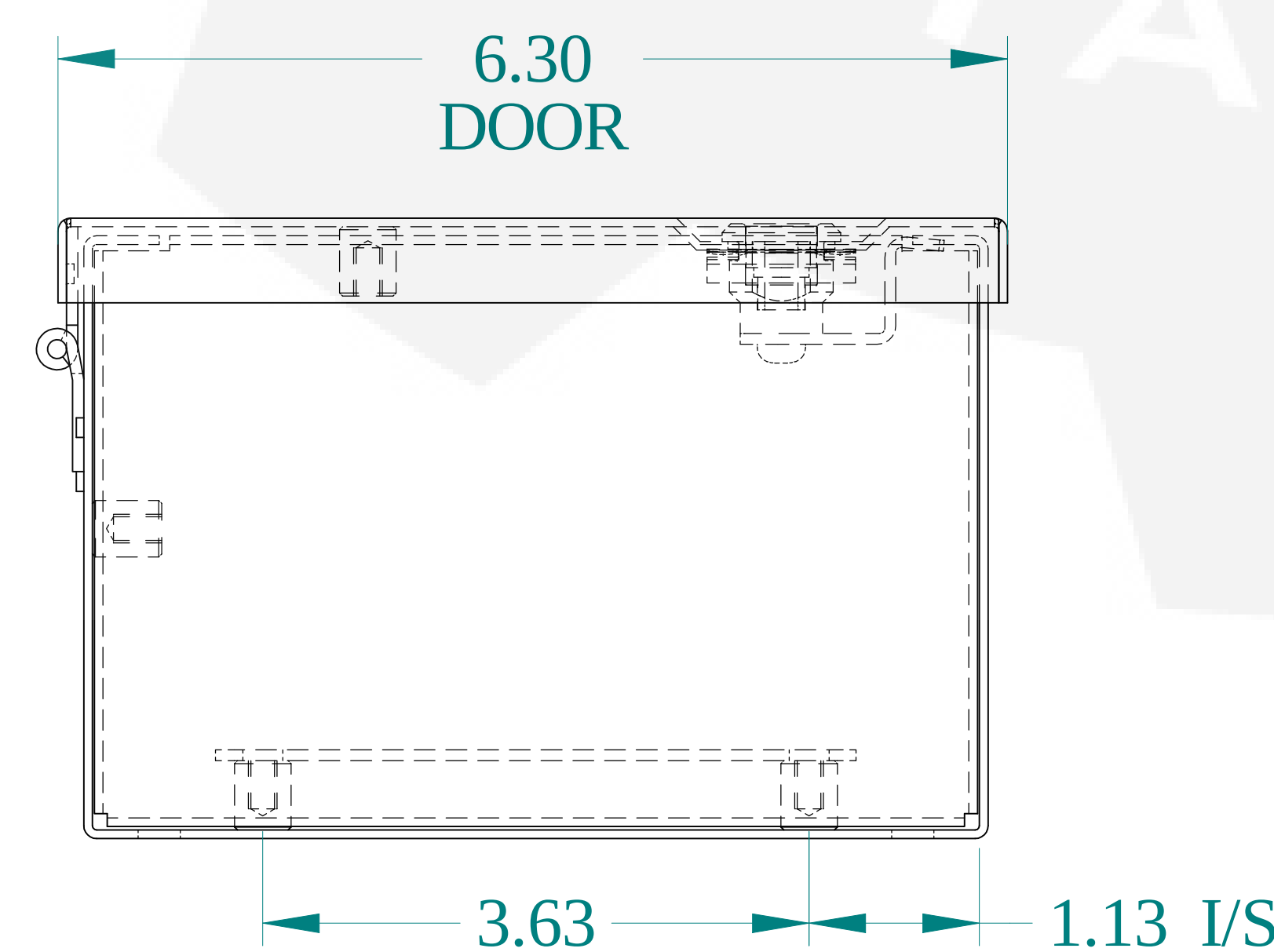
BOTTOM VIEW
