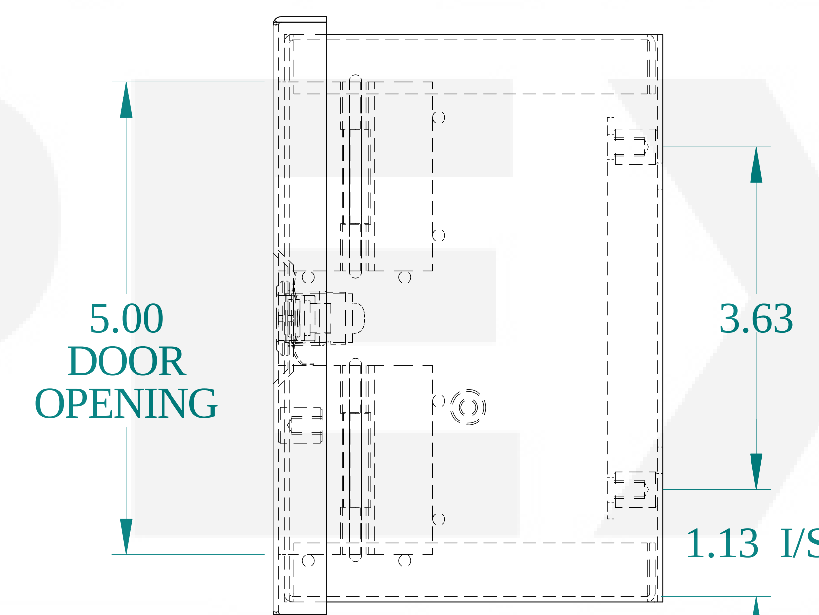
SIDE VIEW
