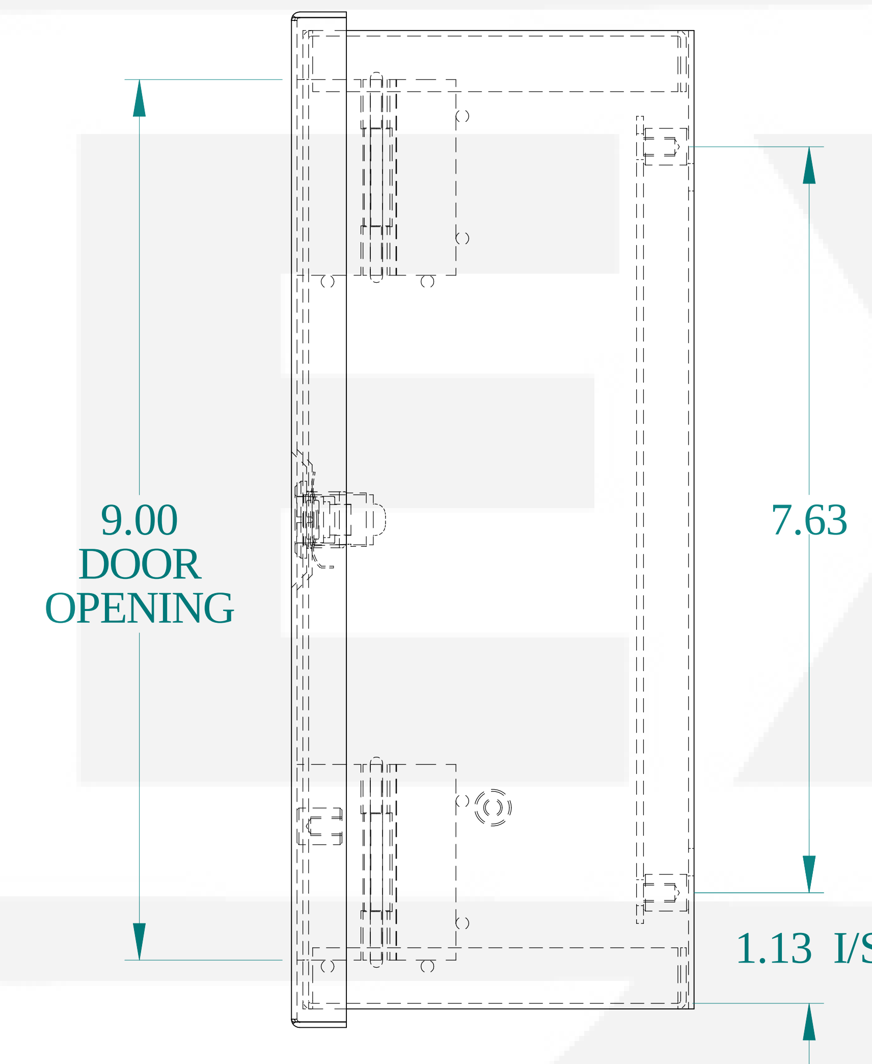
SIDE VIEW
