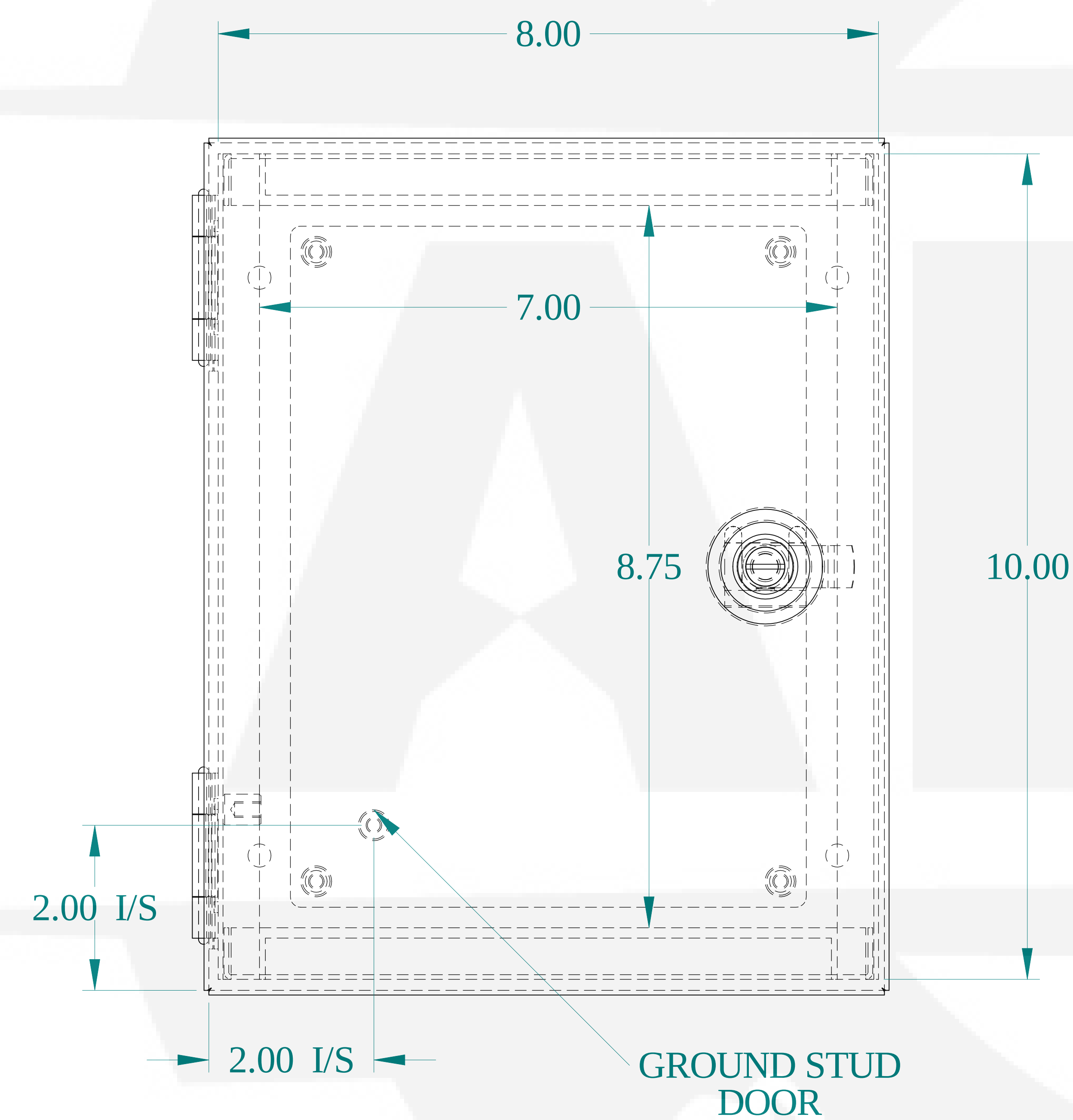
FRONT VIEW
