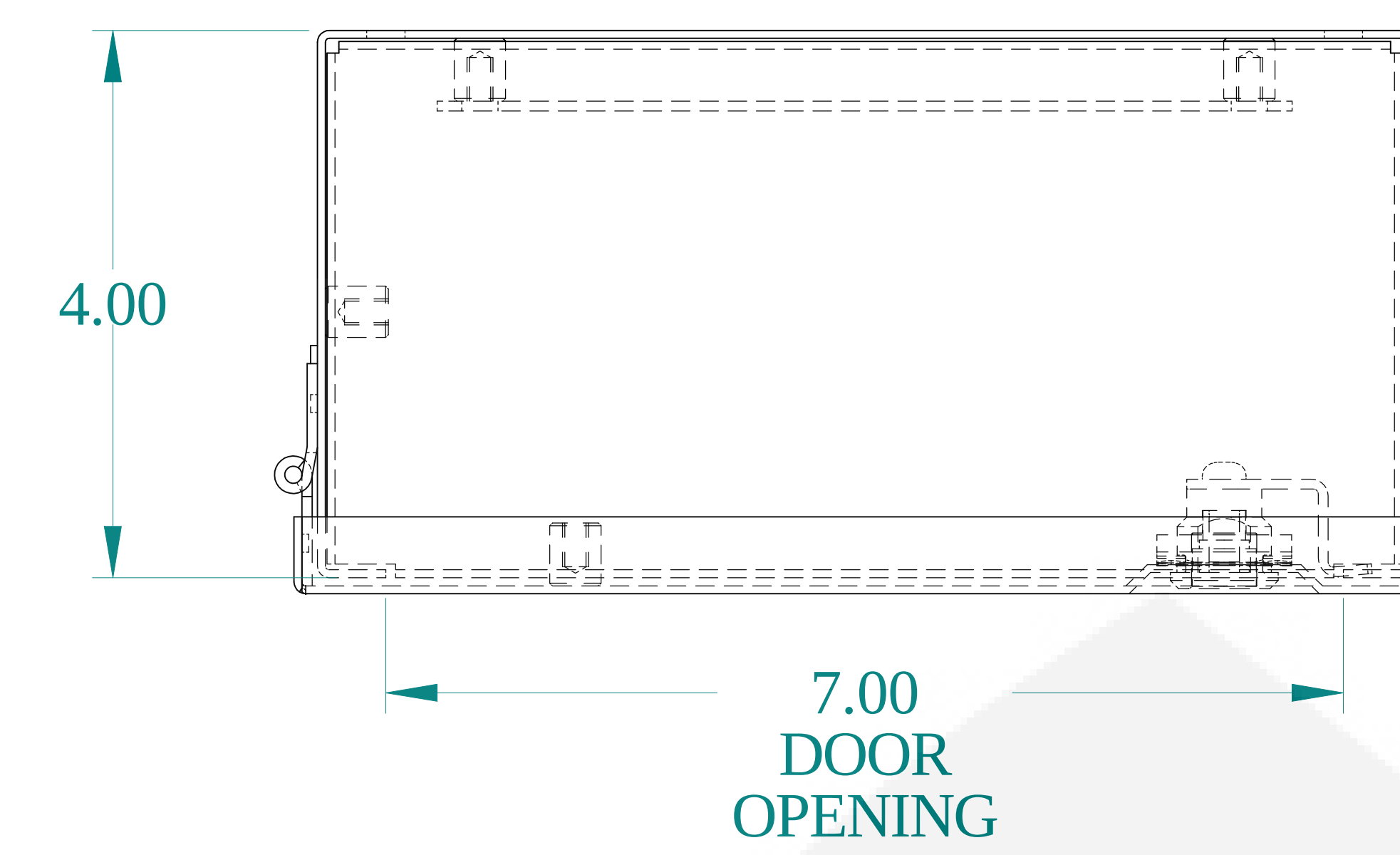
TOP VIEW
