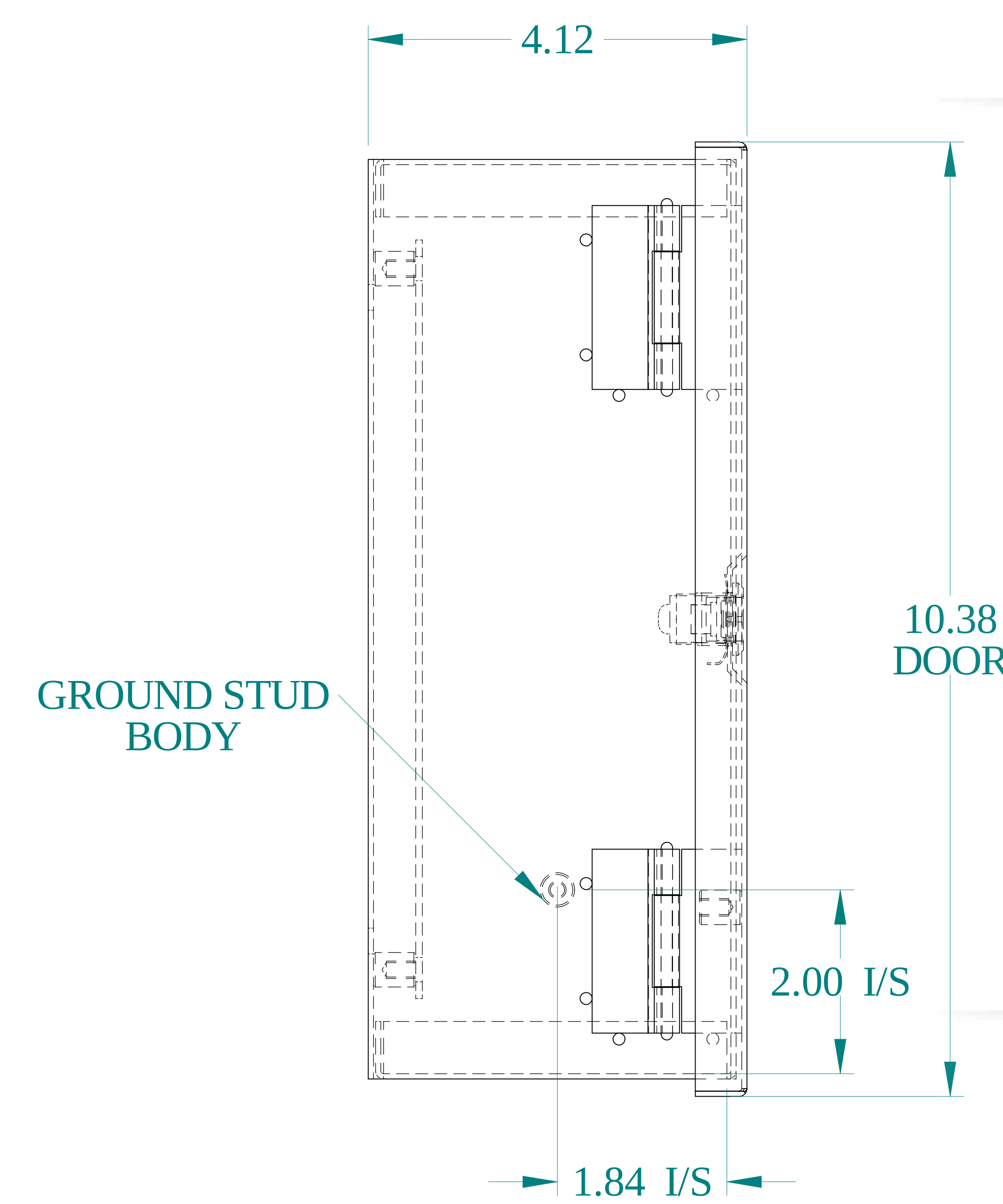
SIDE VIEW
