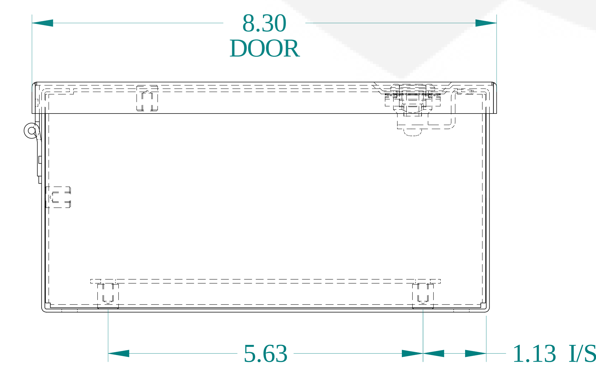
BOTTOM VIEW
