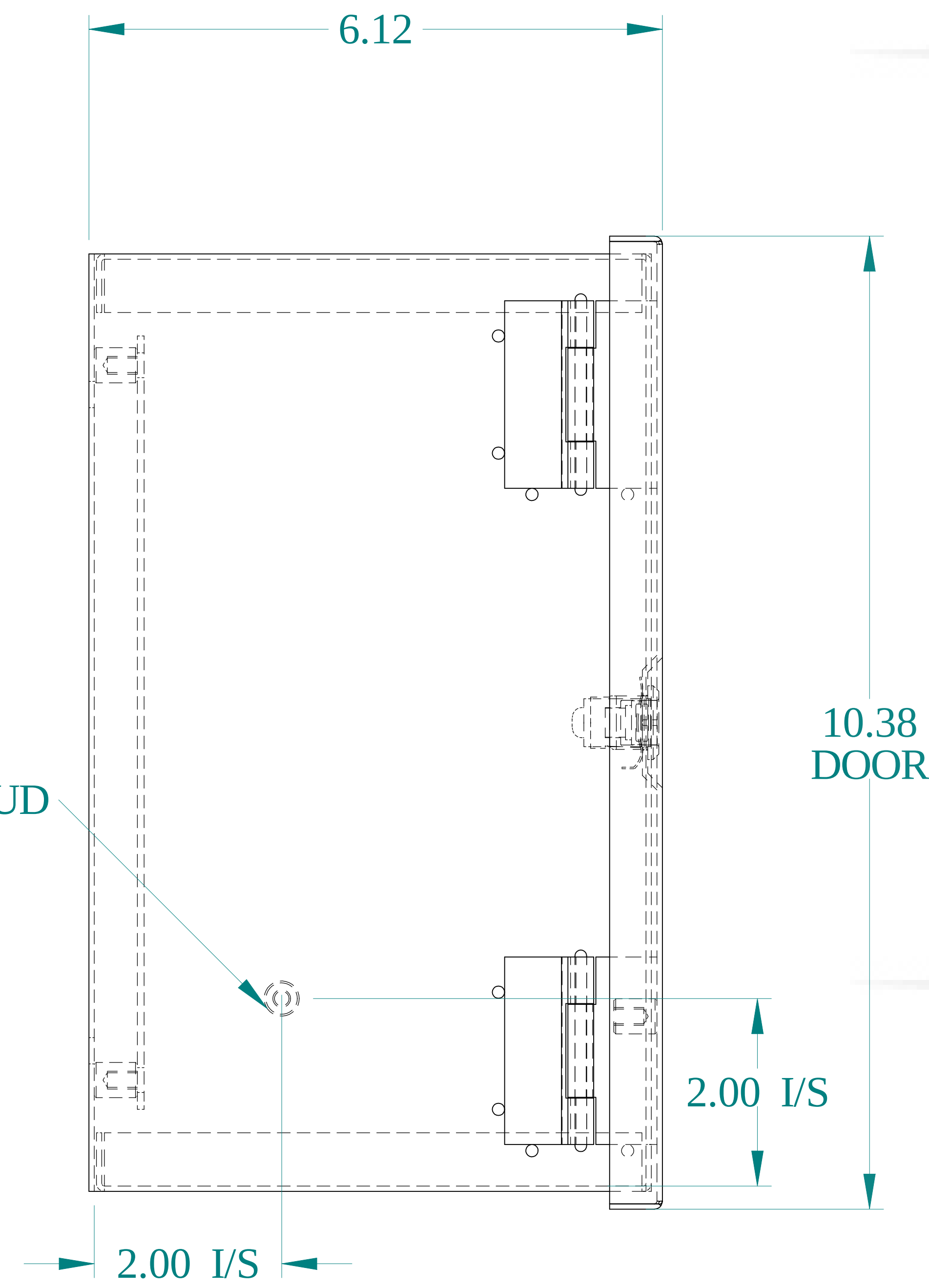
SIDE VIEW
