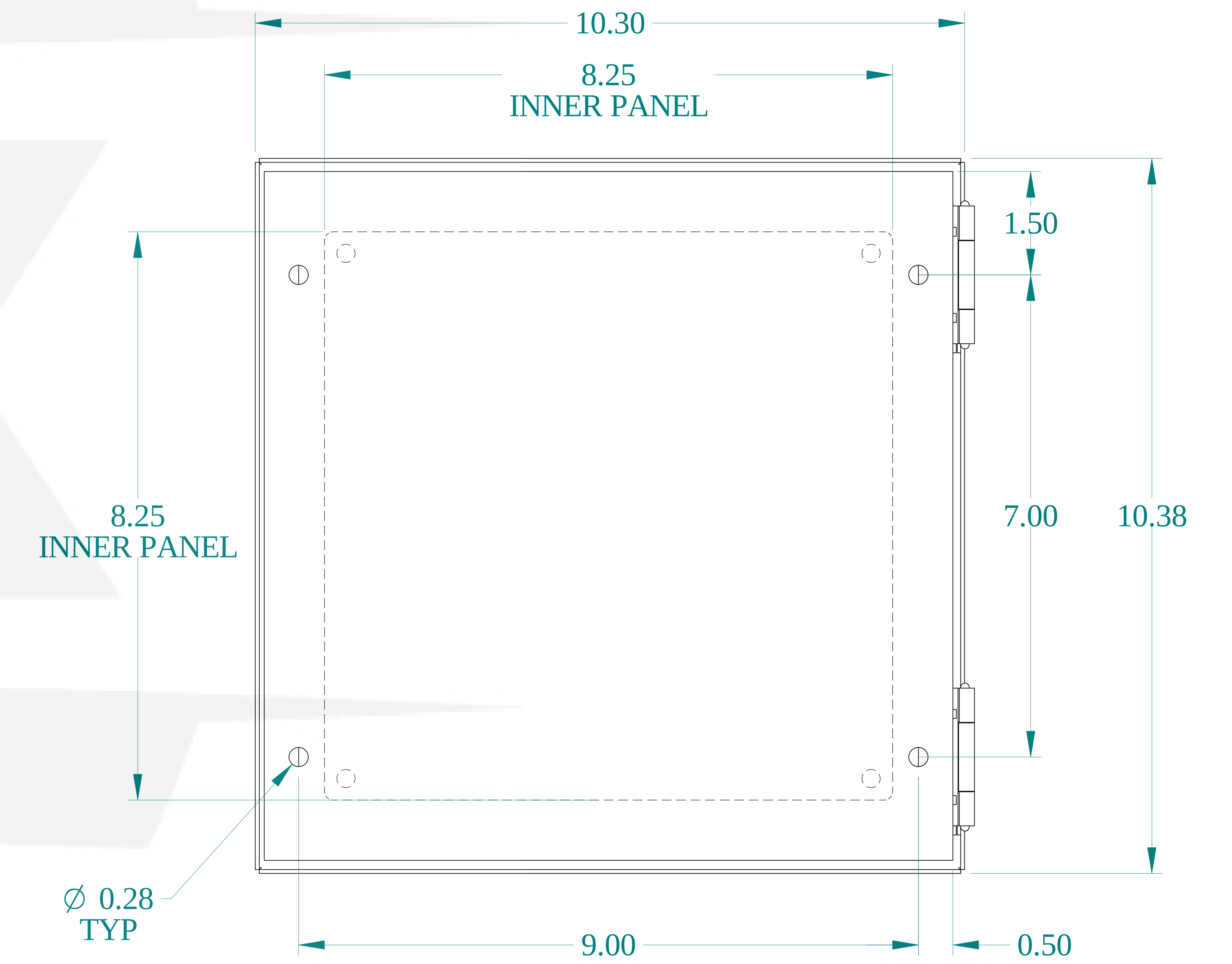
BACK VIEW
