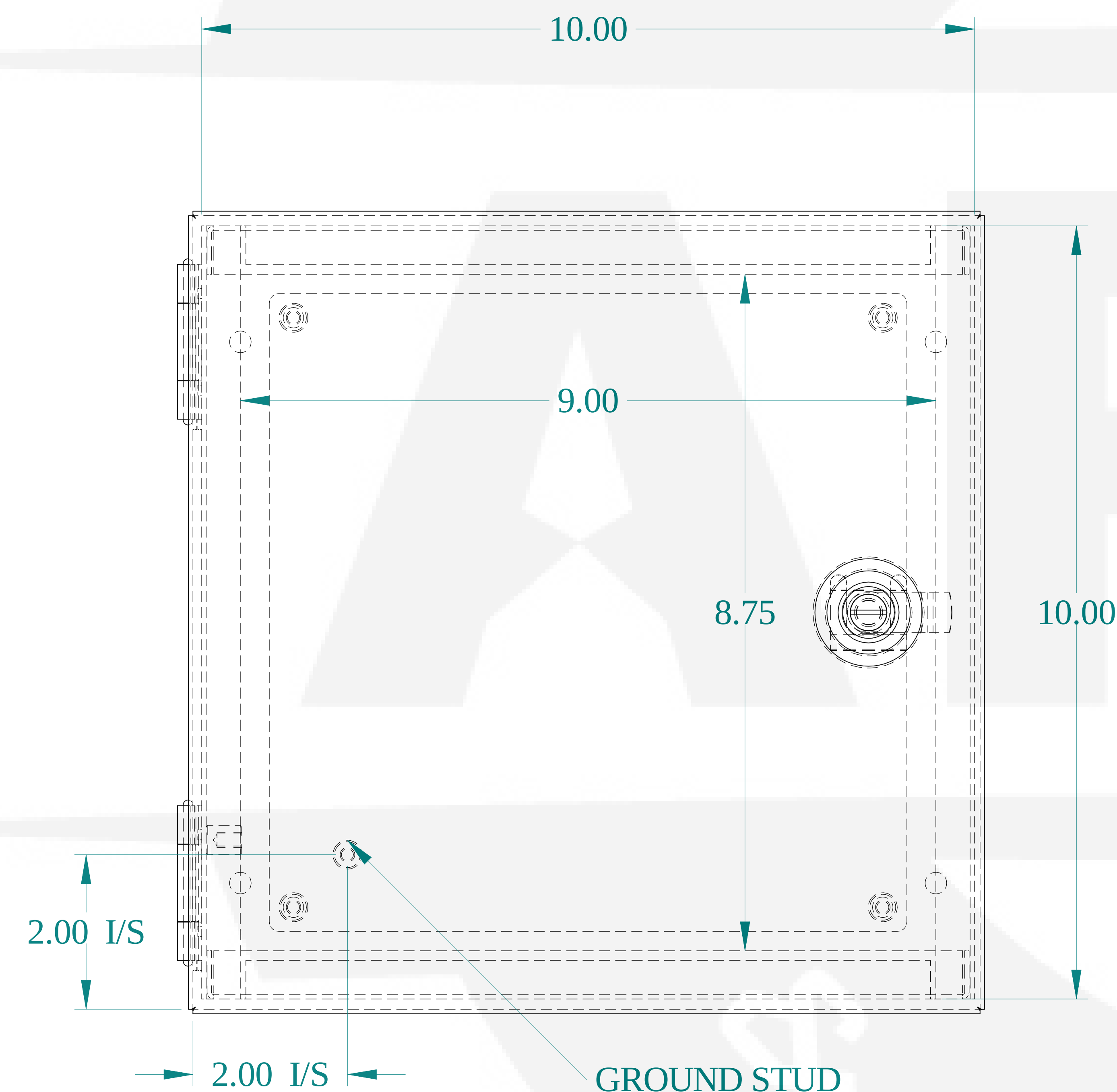
FRONT VIEW
