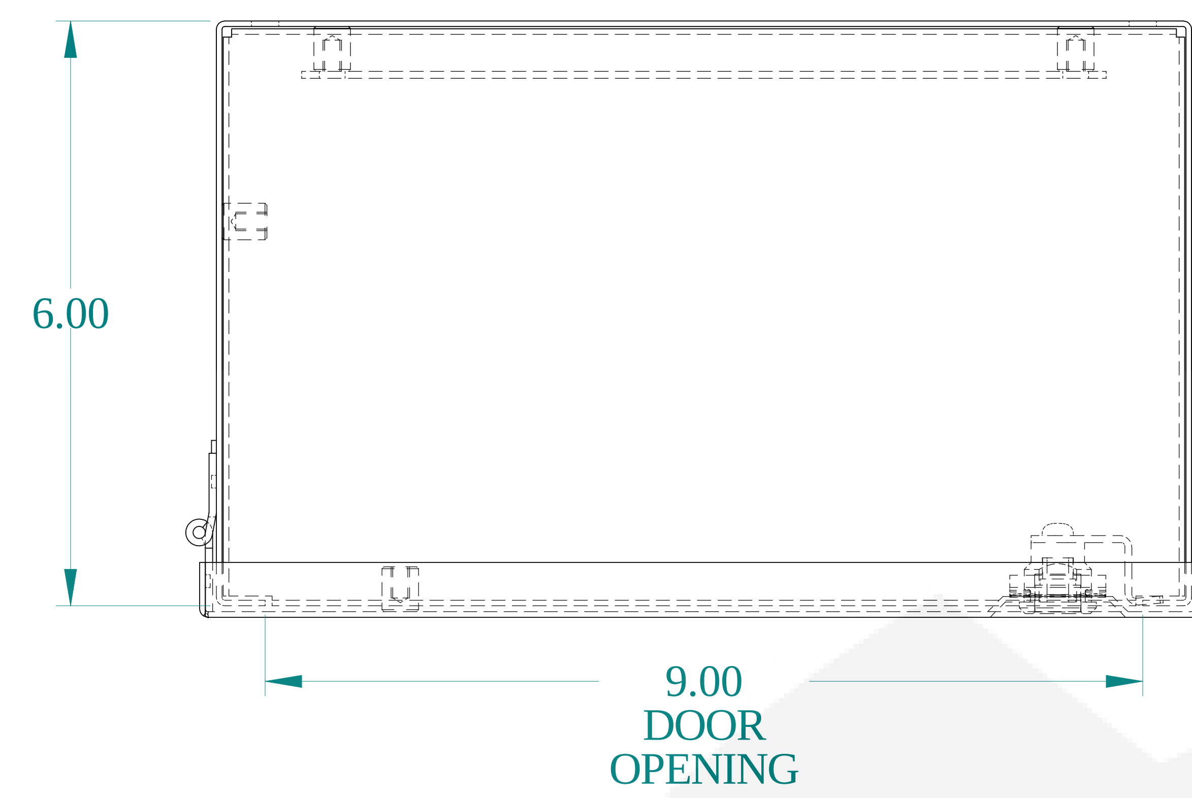
TOP VIEW
