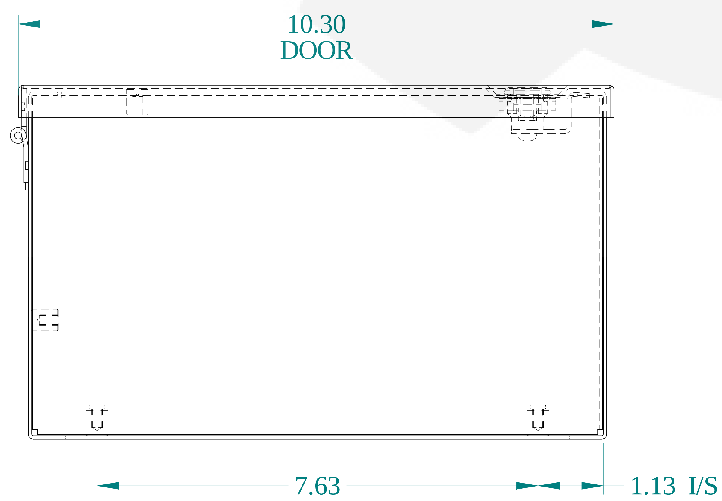
BOTTOM VIEW
