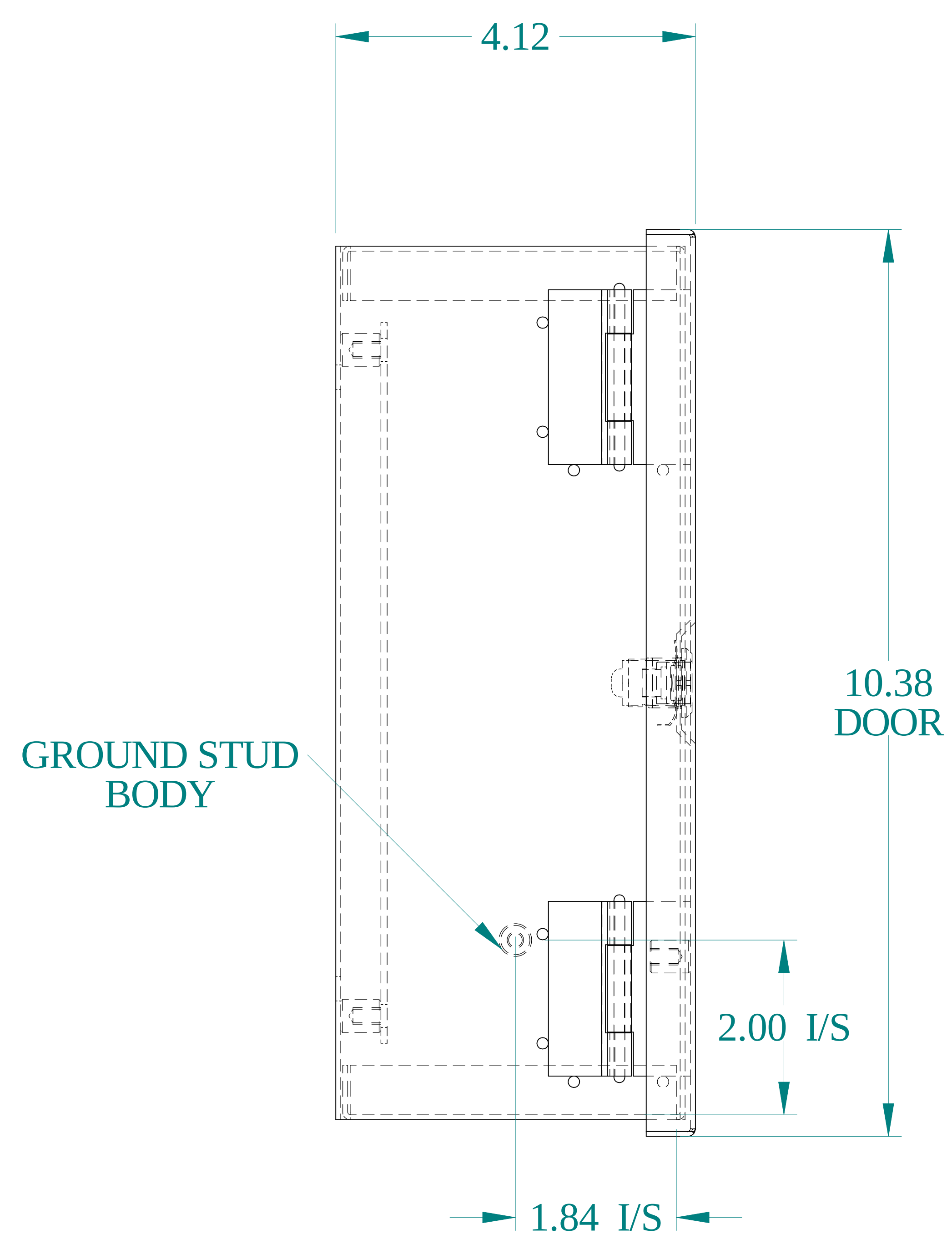
SIDE VIEW
