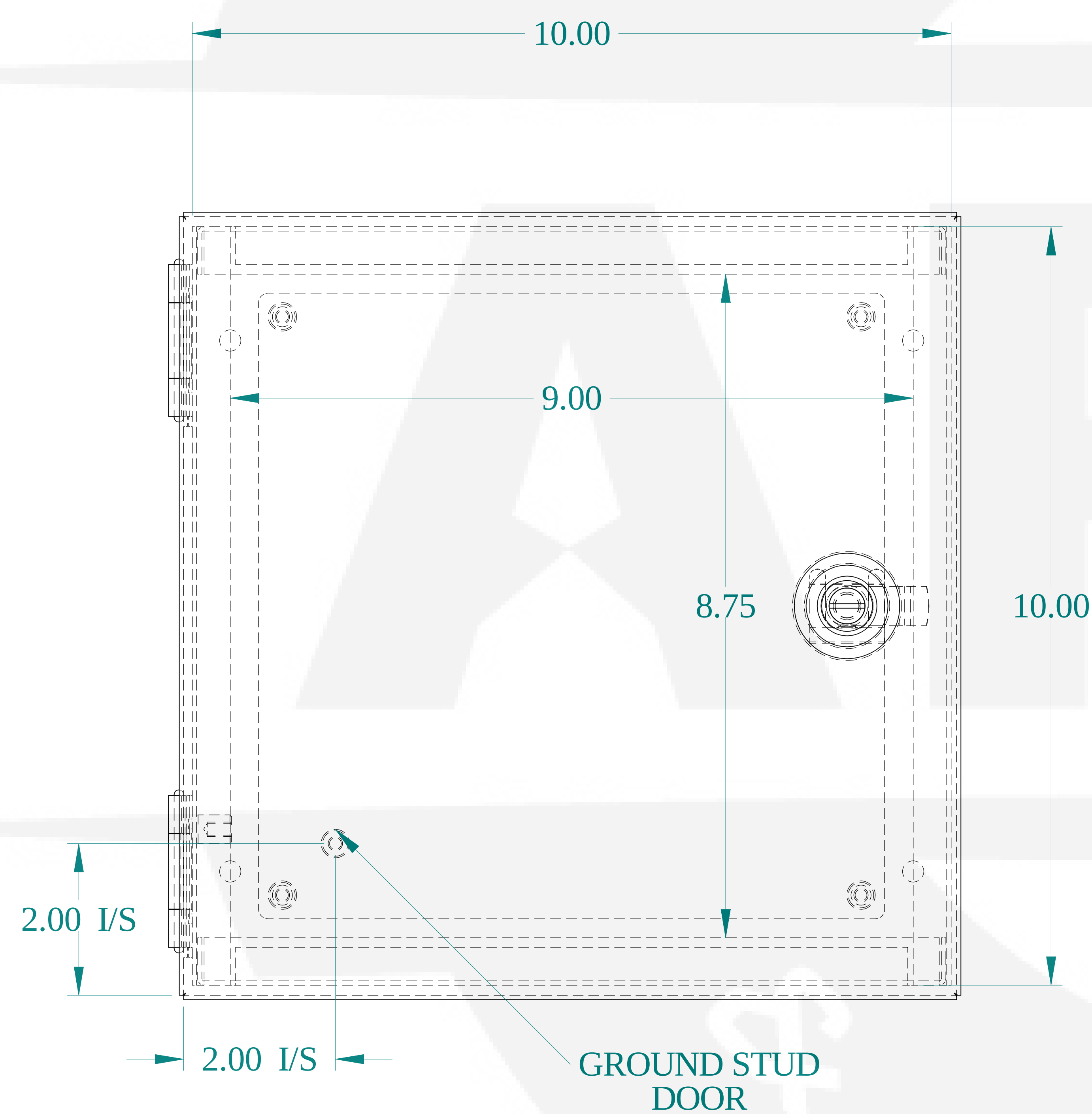
FRONT VIEW
