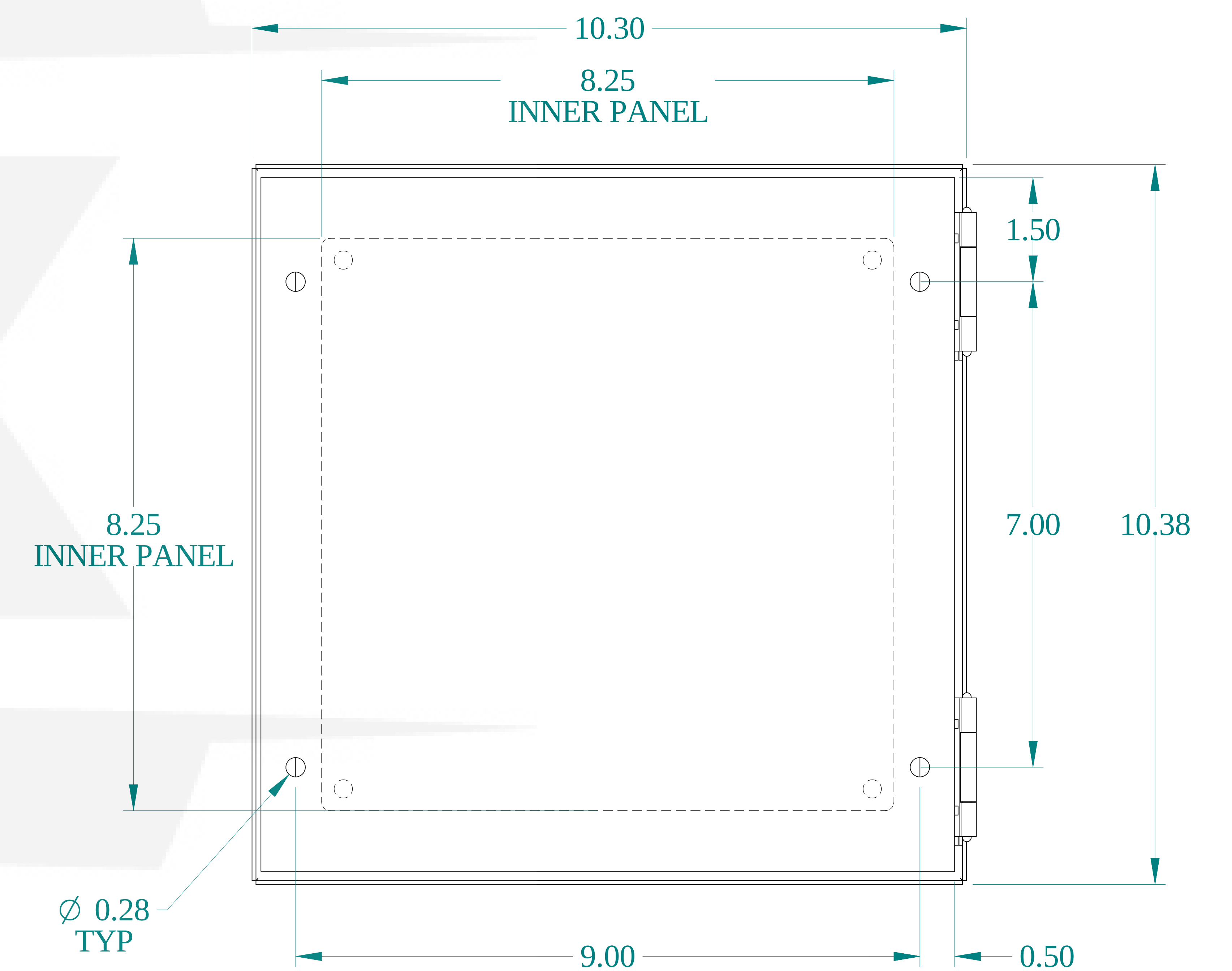
BACK VIEW
