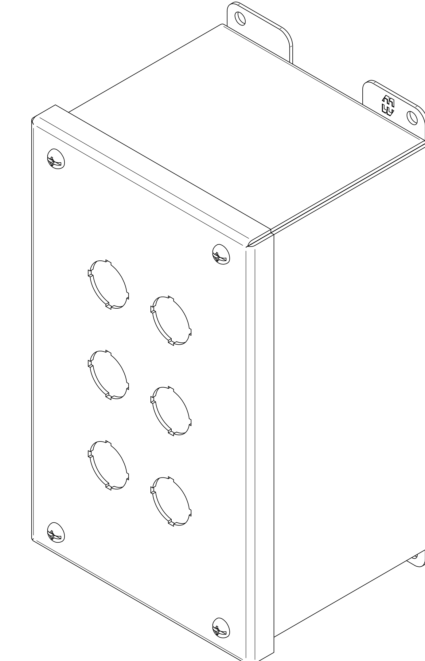
ISOMETRIC VIEWS
