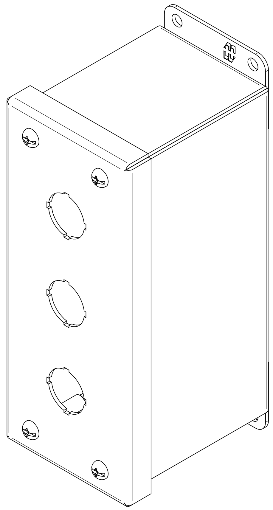
ISOMETRIC VIEWS
