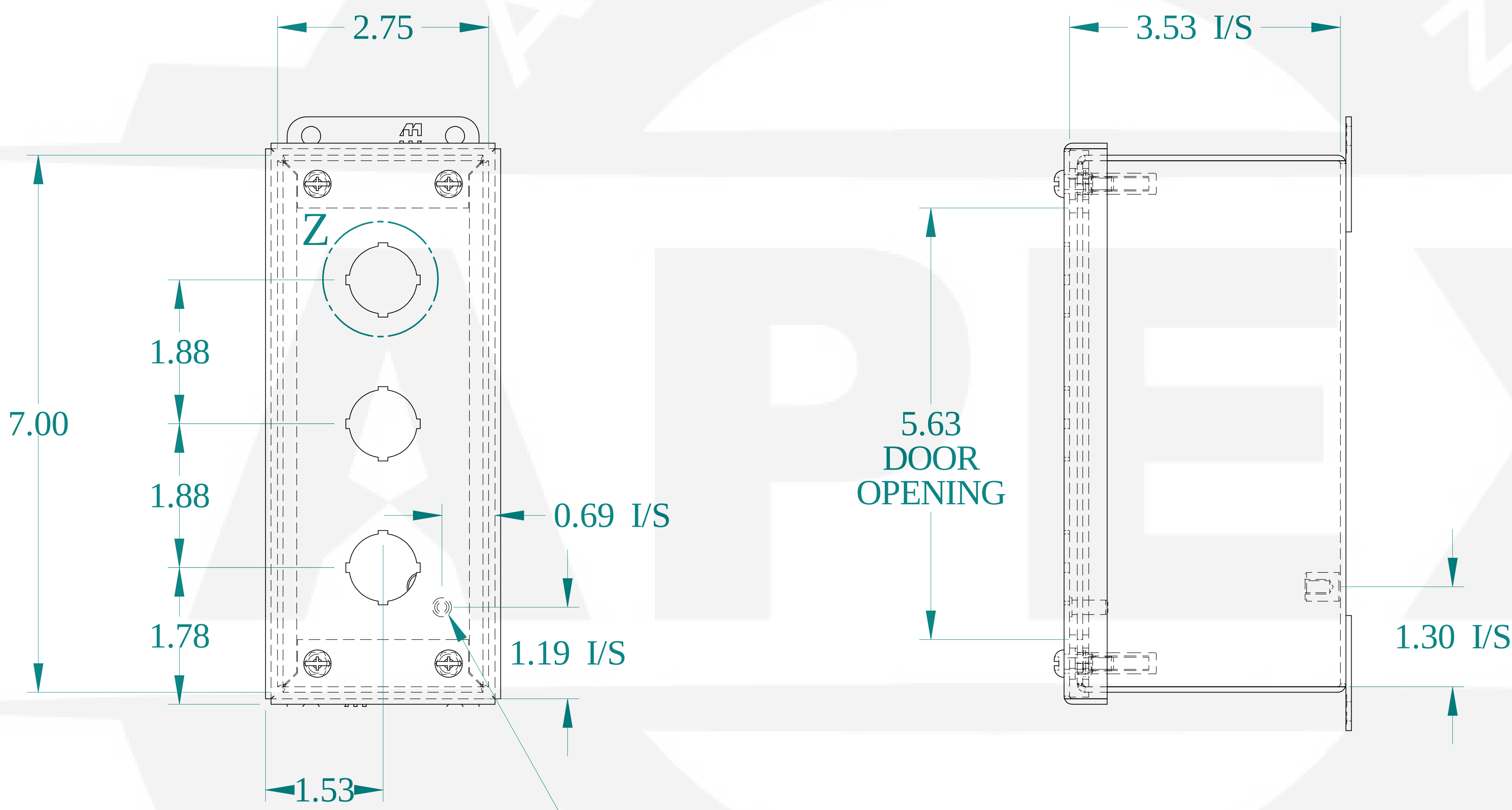
FRONT VIEW
