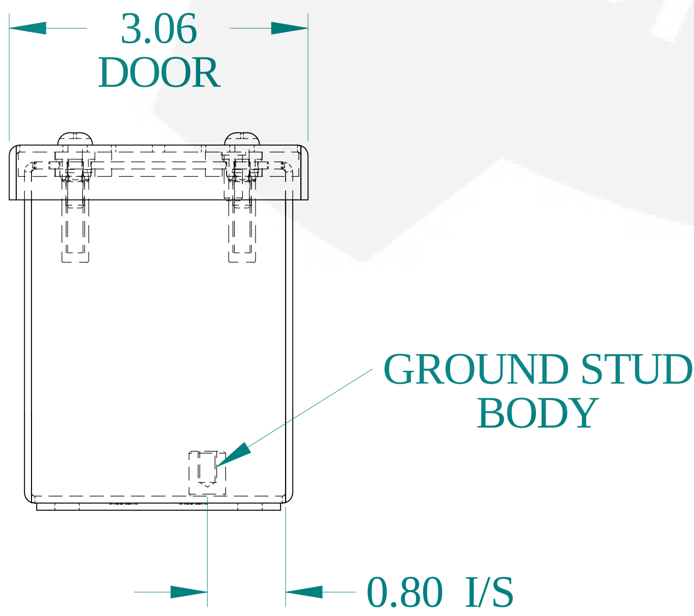
BOTTOM VIEW
