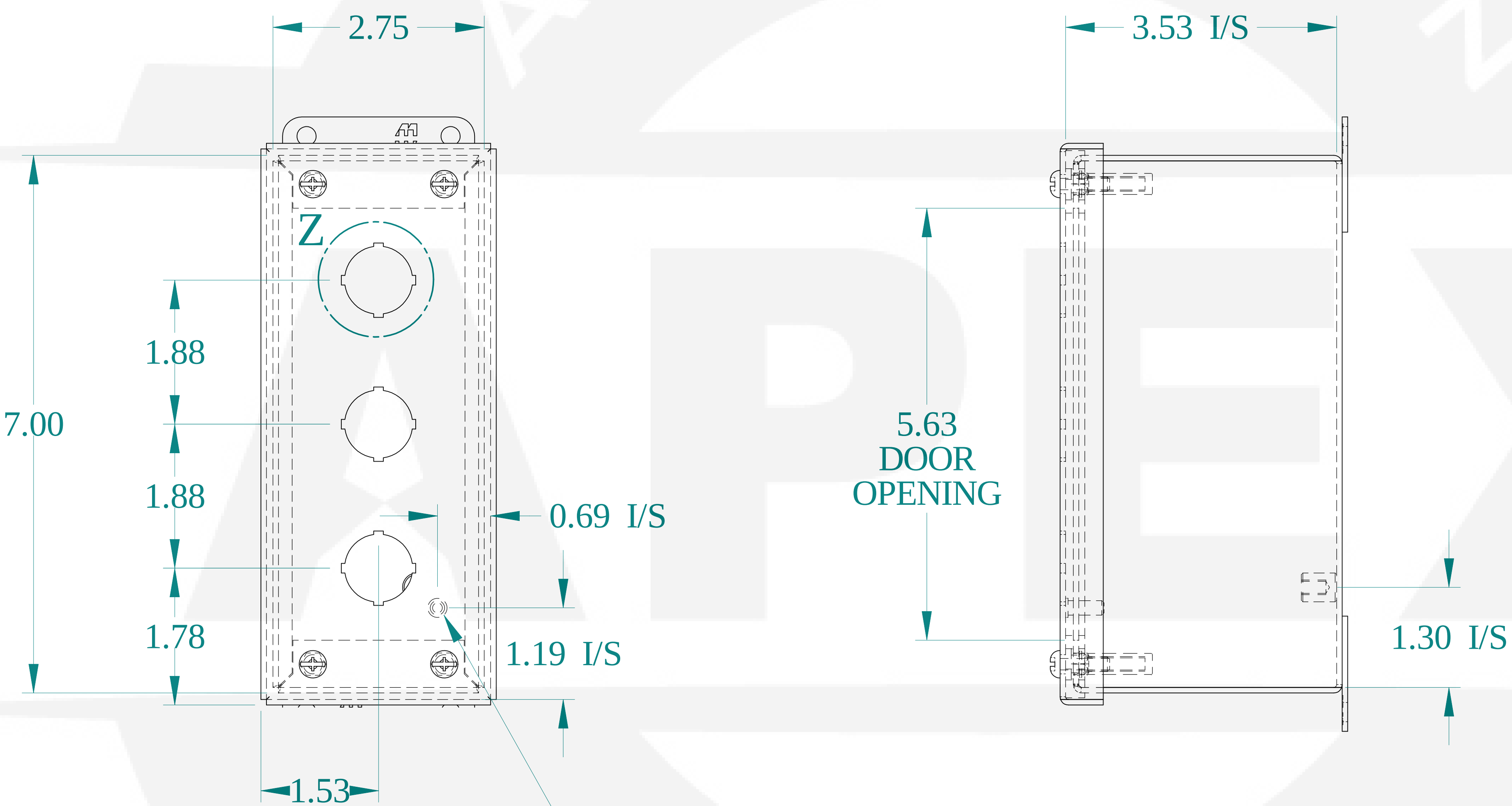
FRONT VIEW
