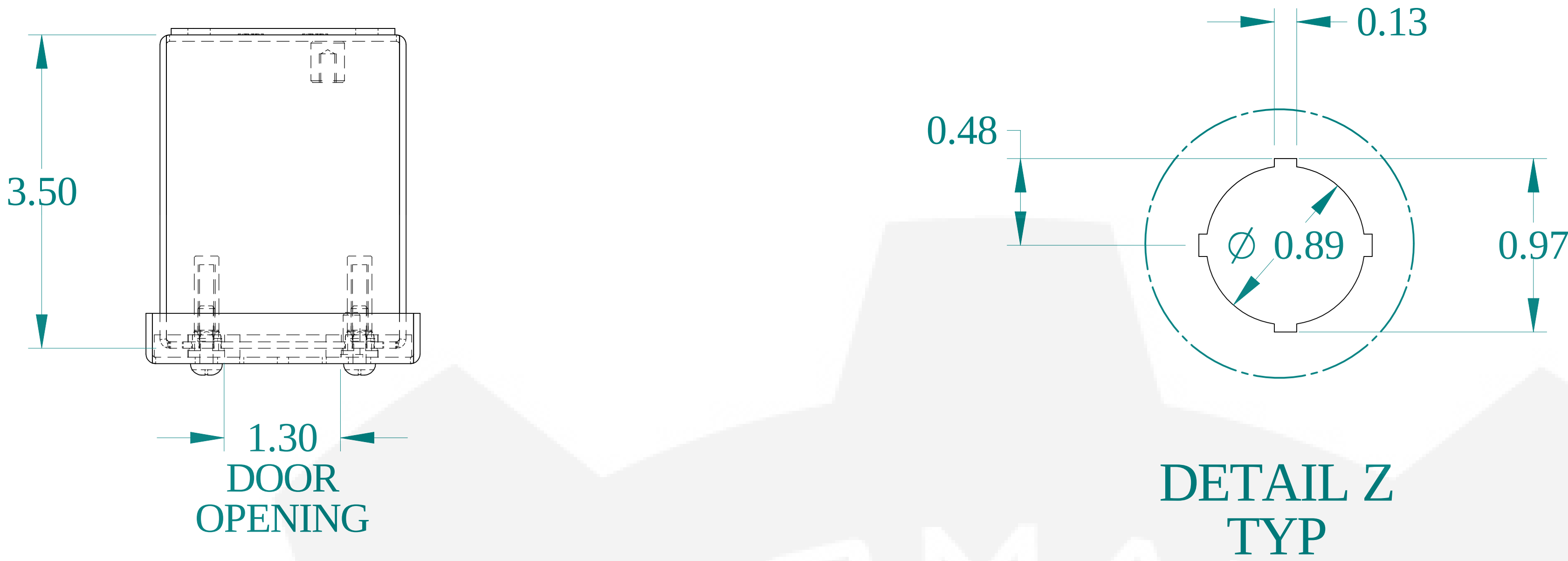
TOP VIEW
