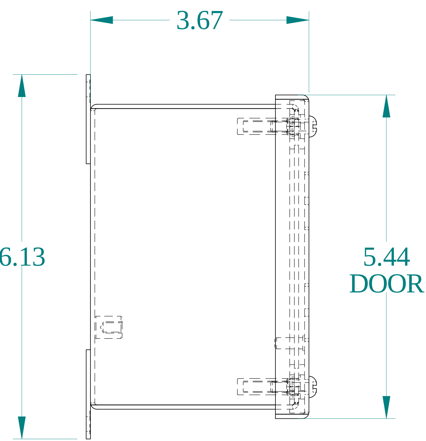
SIDE VIEW
