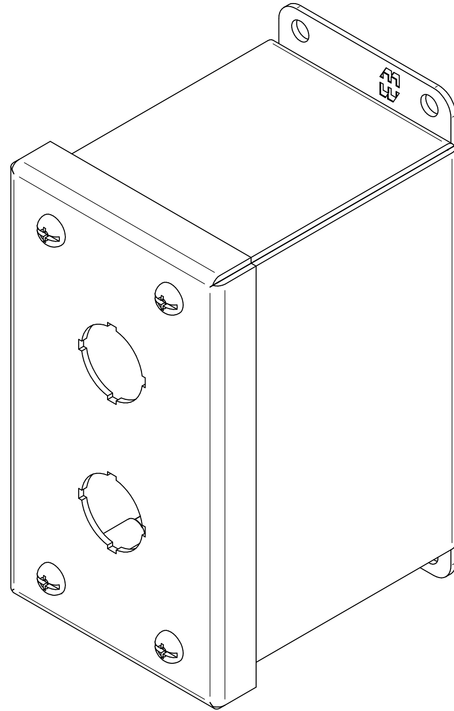
ISOMETRIC VIEWS
