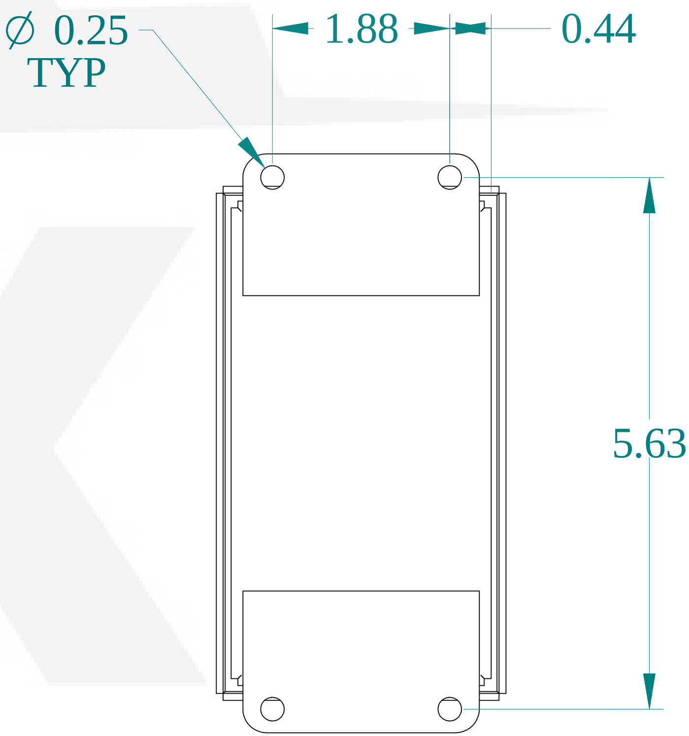
BACK VIEW
