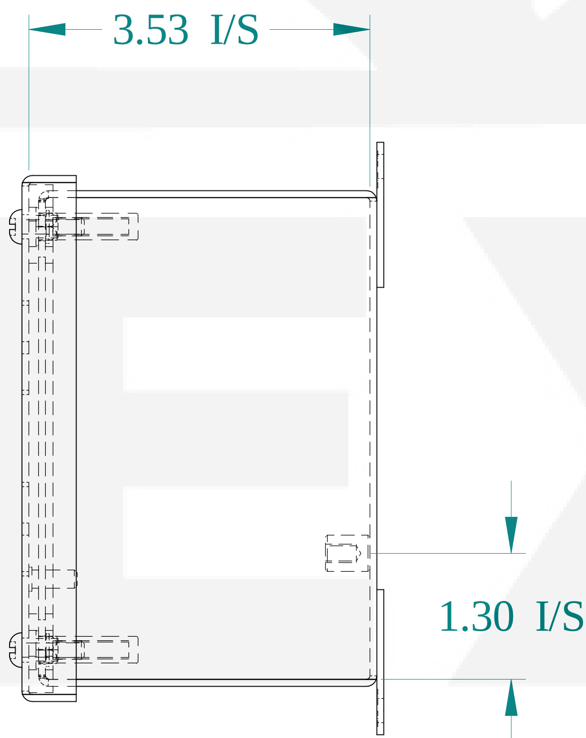
SIDE VIEW
