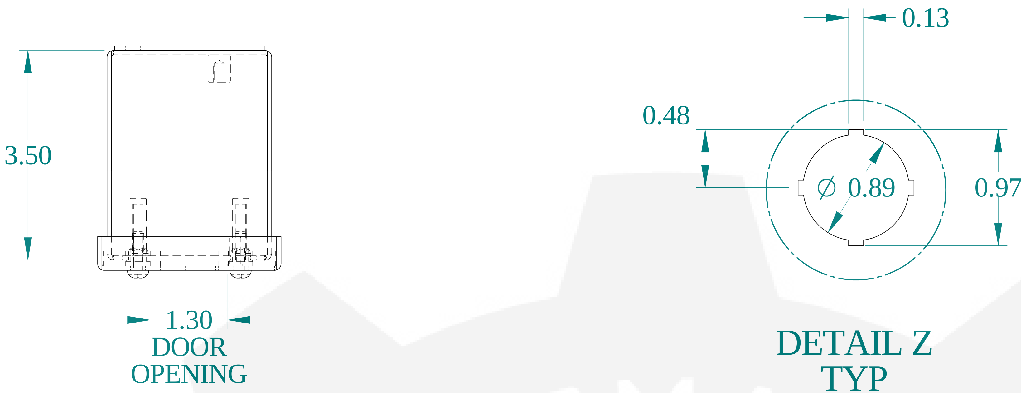
TOP VIEW
