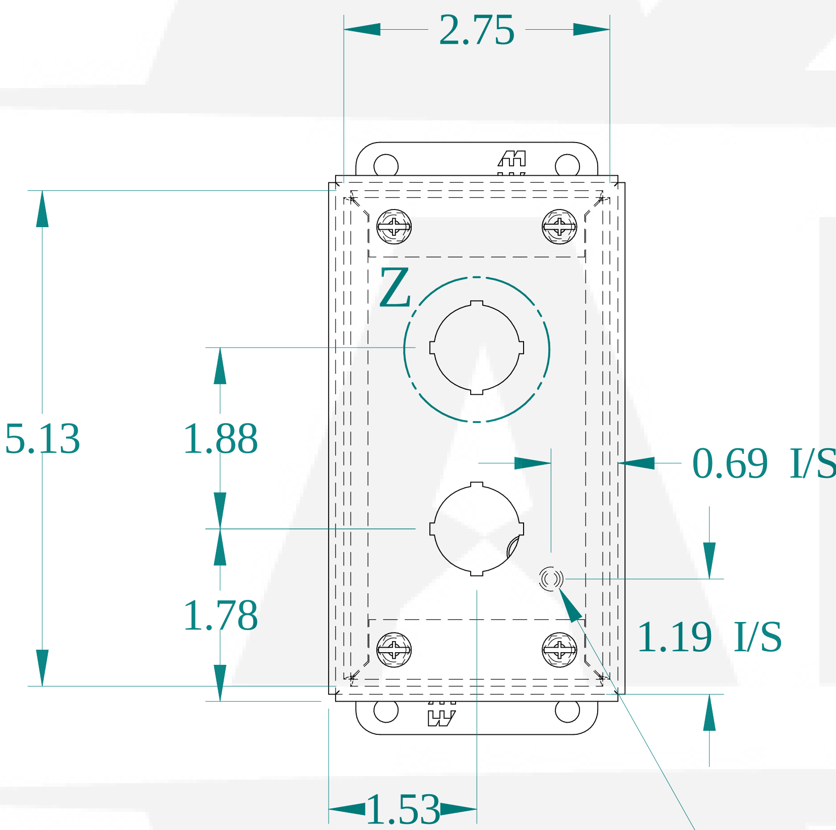
FRONT VIEW
