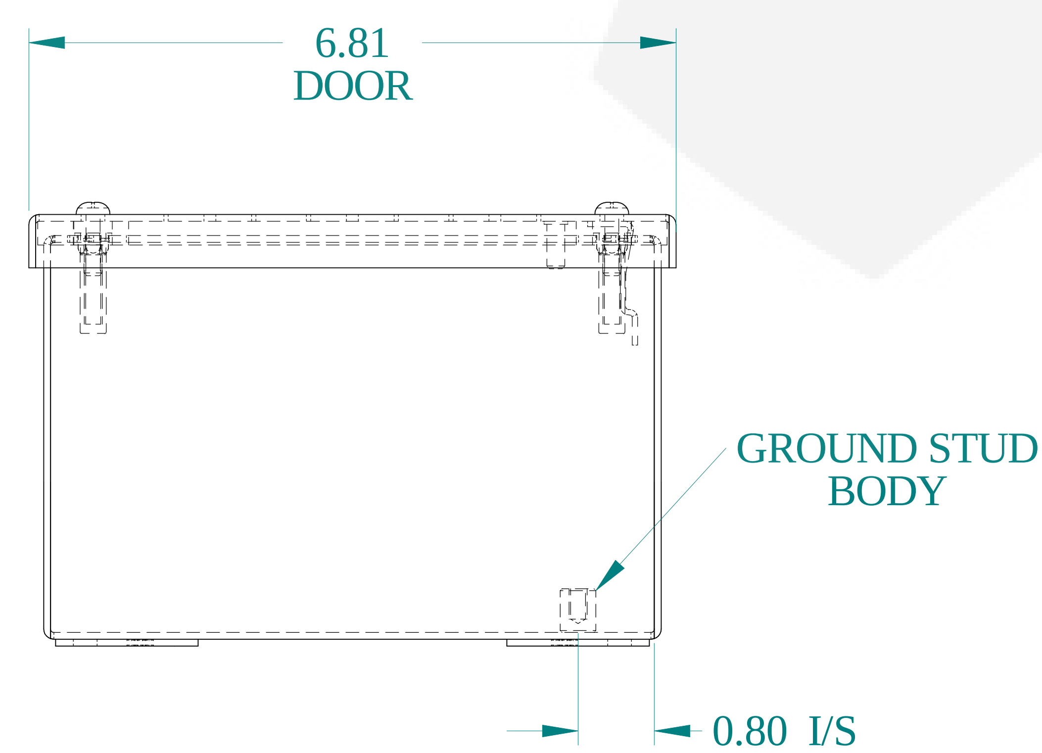
BOTTOM VIEW
