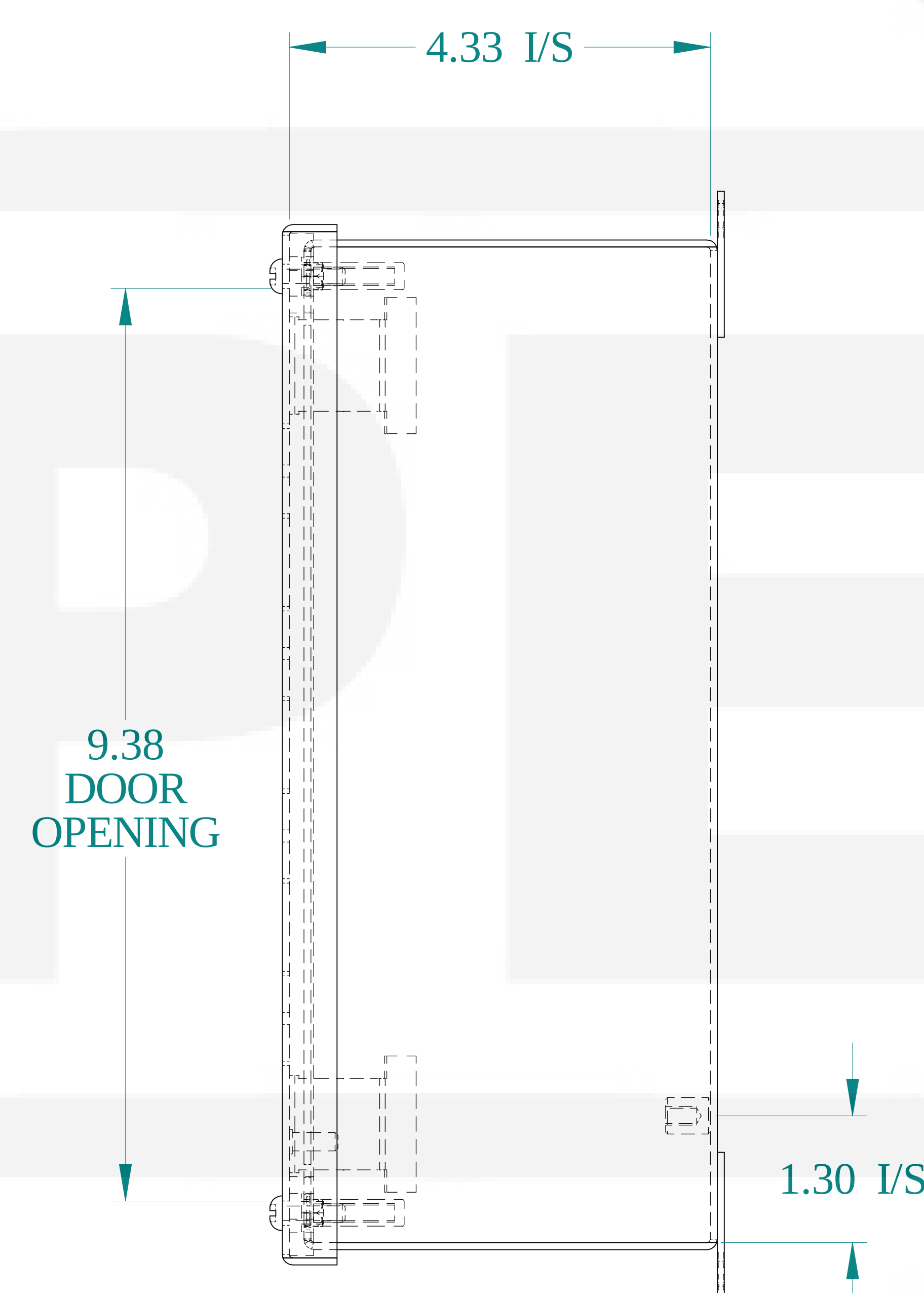
SIDE VIEW
