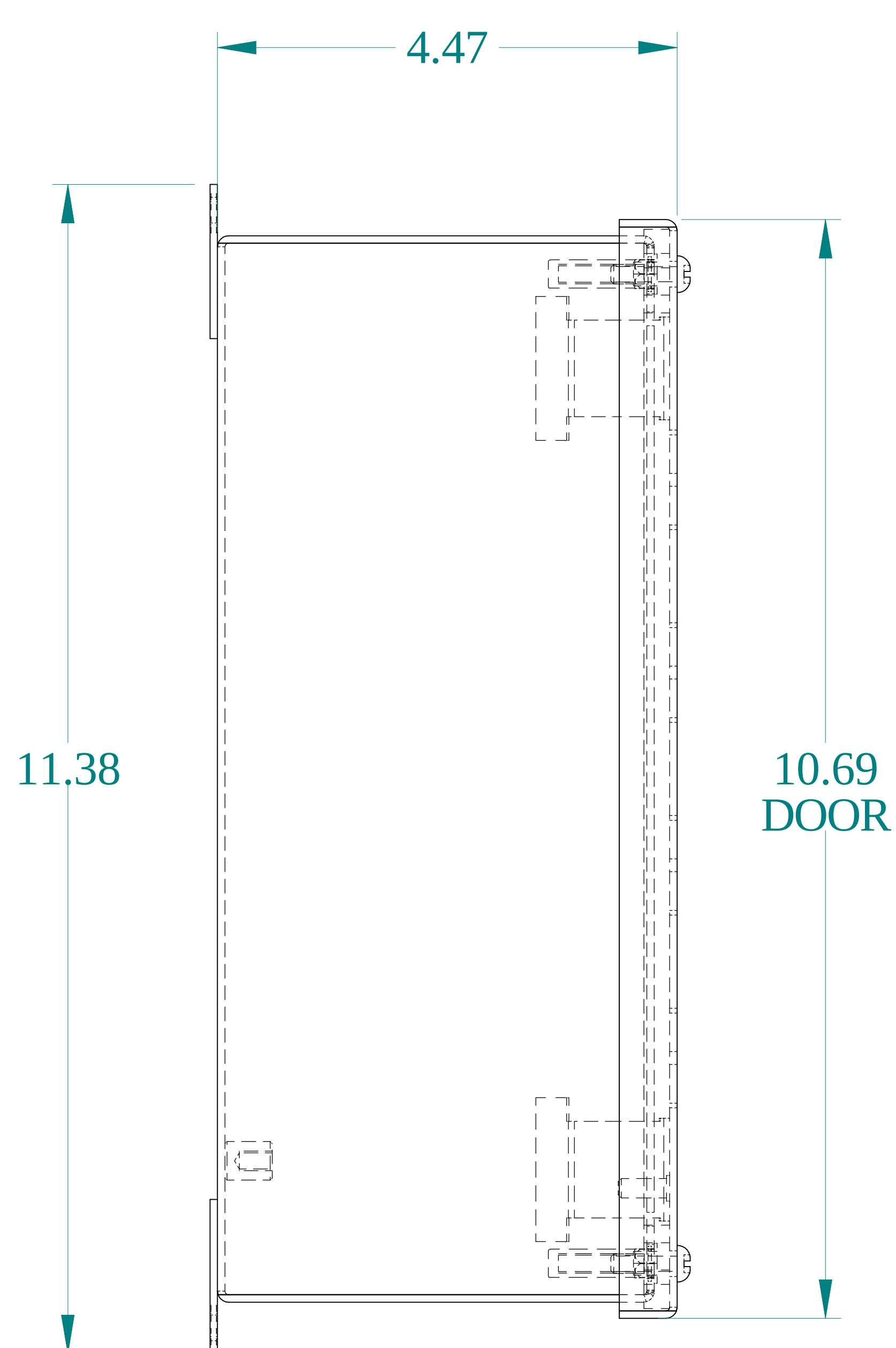
SIDE VIEW
