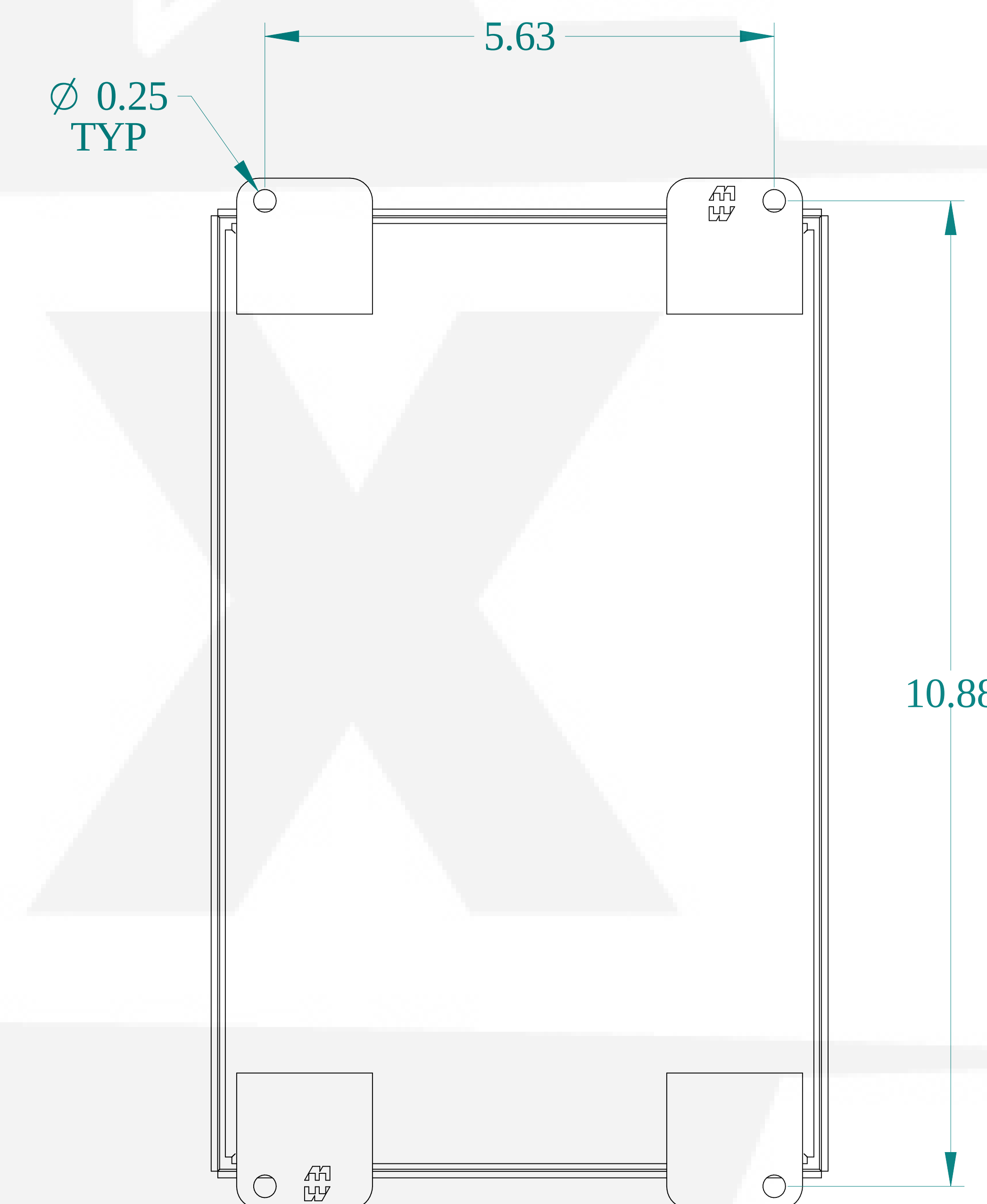
BACK VIEW
