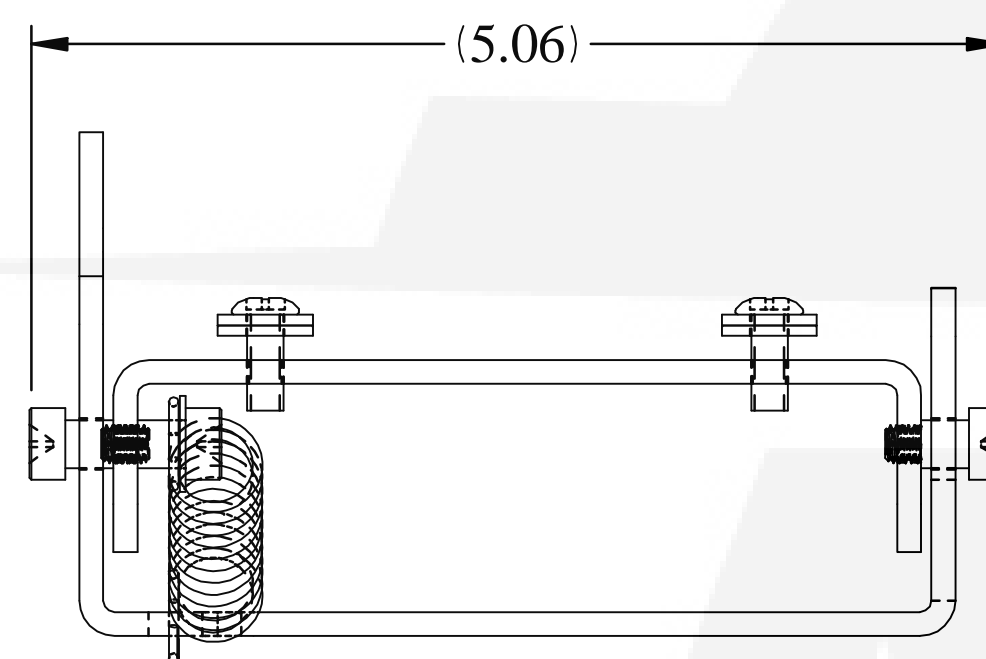
TOP VIEW
