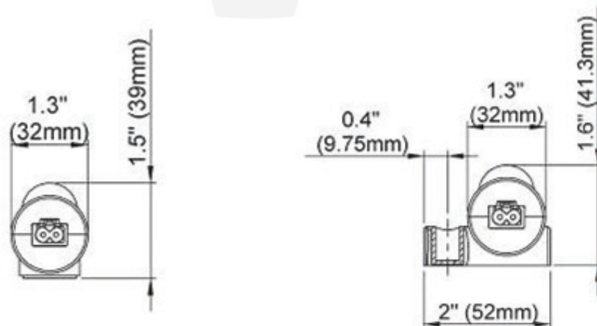
Magnet mount end view
