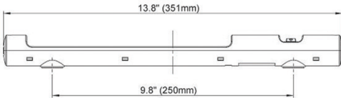
On/off switch light w/magnet mount
