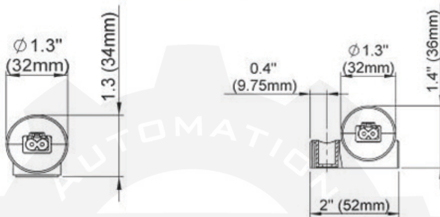
Magnet mount end view
