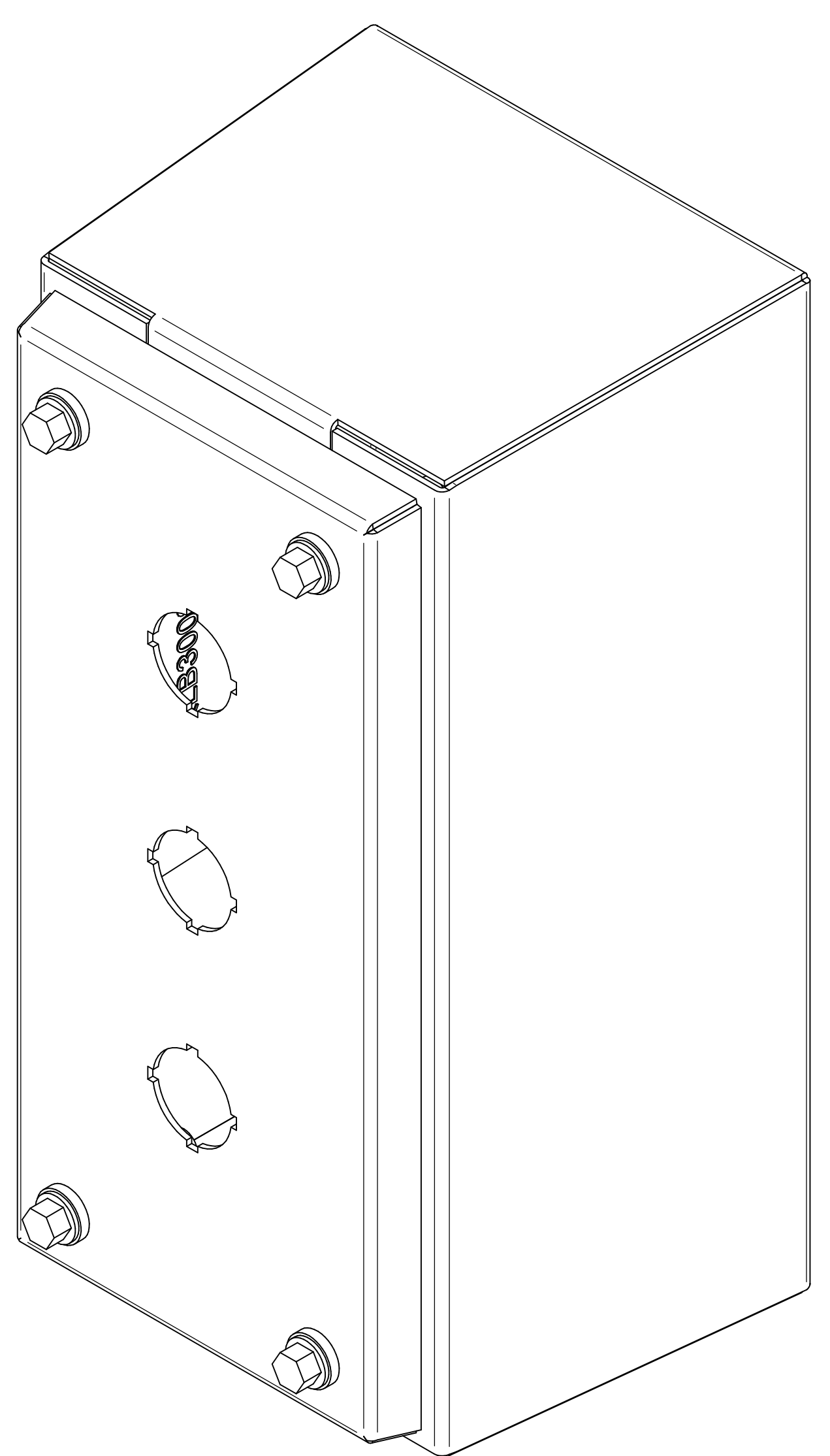
ISOMETRIC VIEWS
