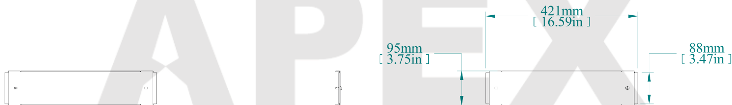
REAR VIEW
