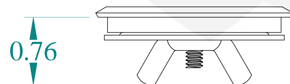
BOTTOM VIEW
