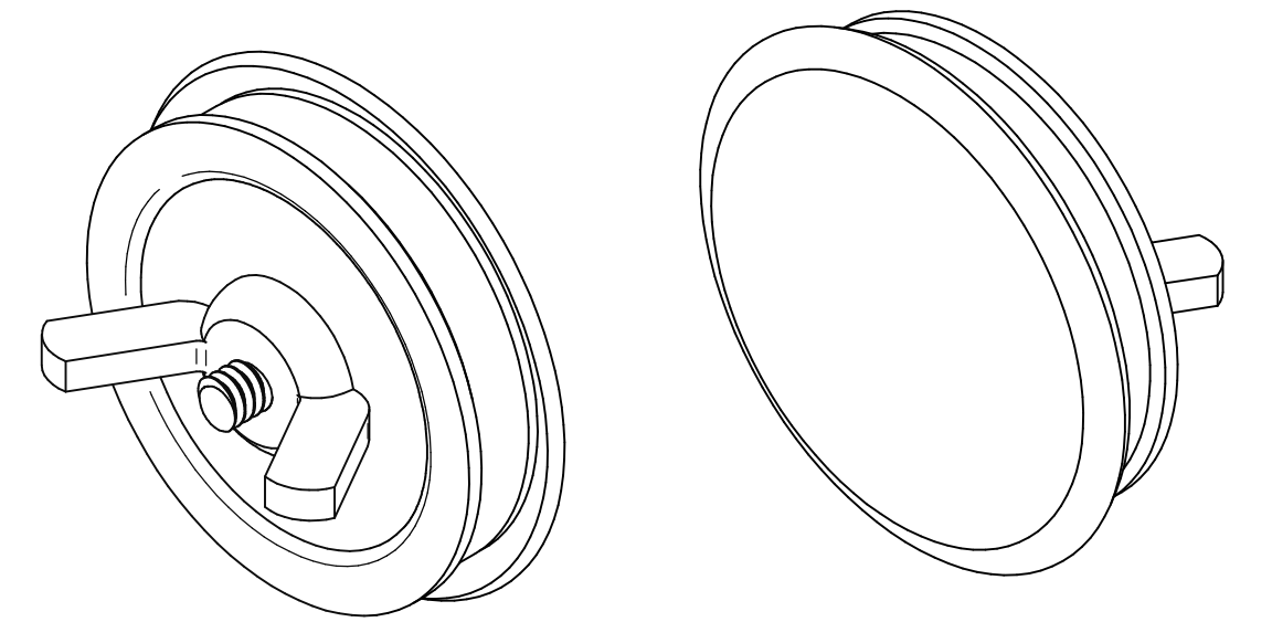
ISOMETRIC VIEWS
