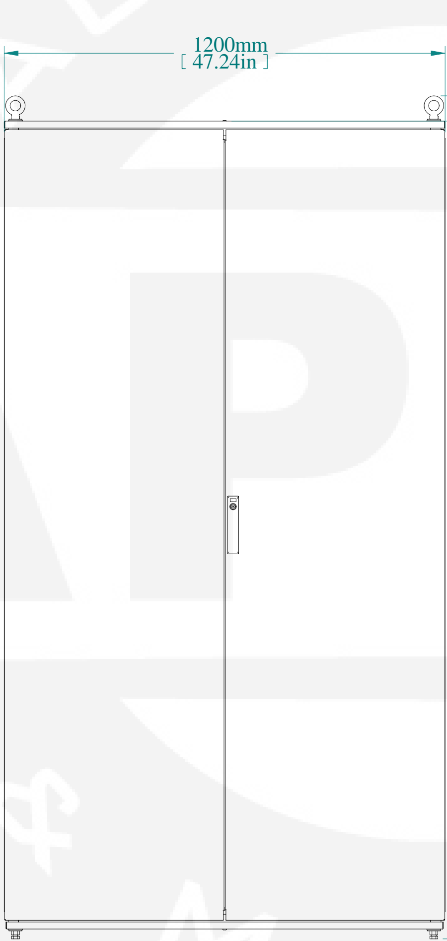
FRONT VIEW
