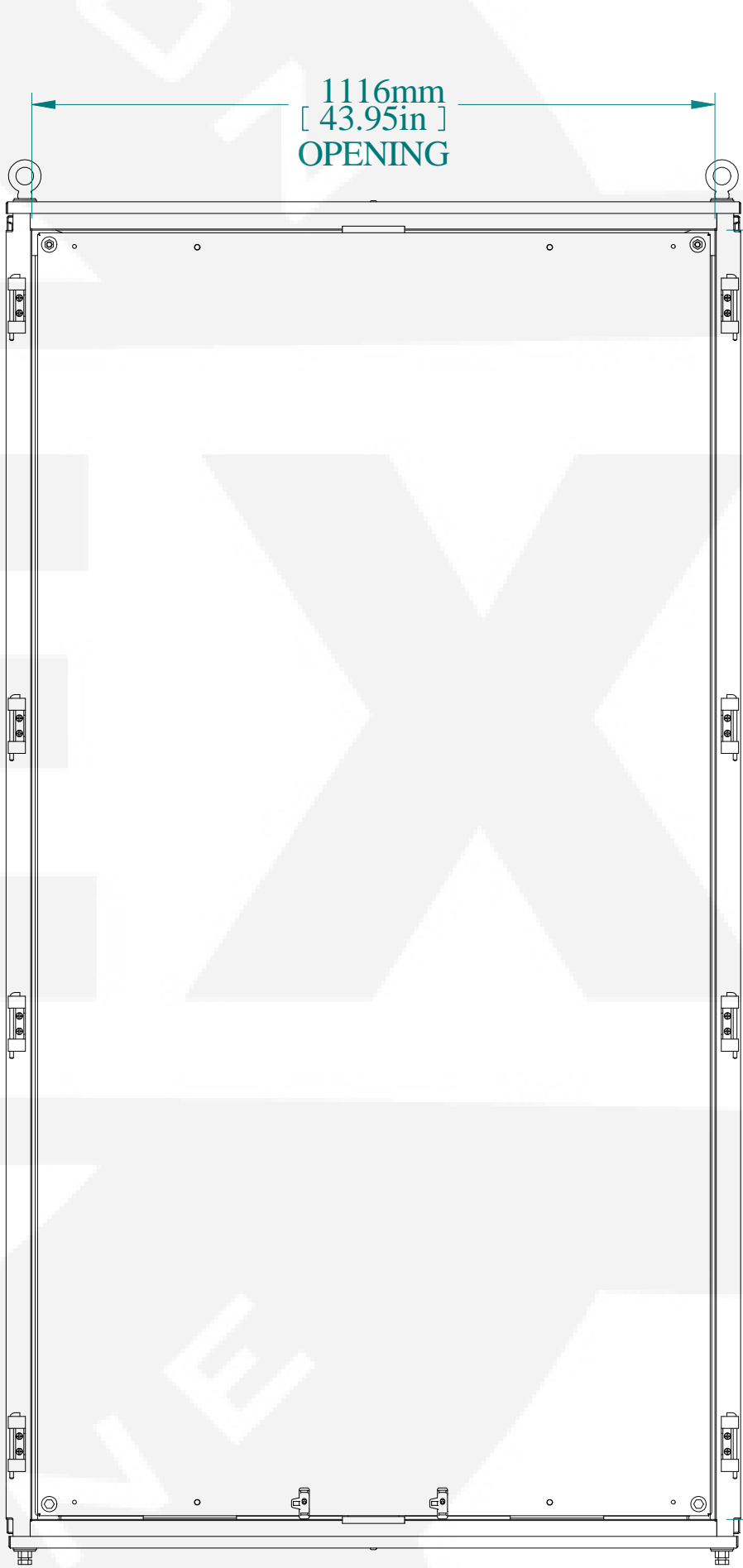
FRONT VIEW DOOR REMOVED
