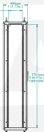
L.S. VIEW
