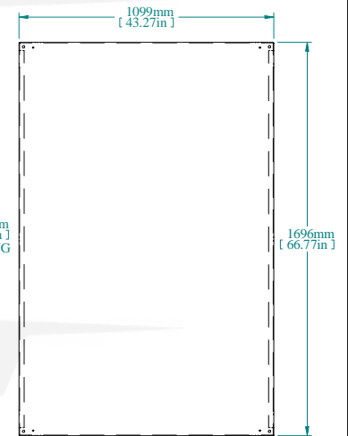
INNER PANEL
