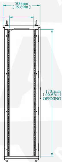
L.S. VIEW
