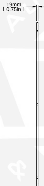
L.H. SIDE VIEW
